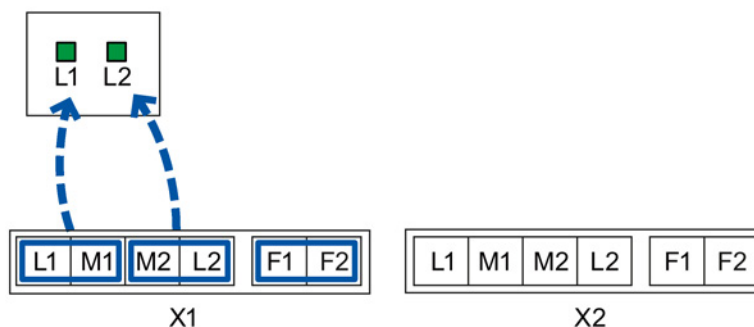
Figure 6-2 Assignment of the LED display to the pins for redundant power supply with devices with two power supply units
