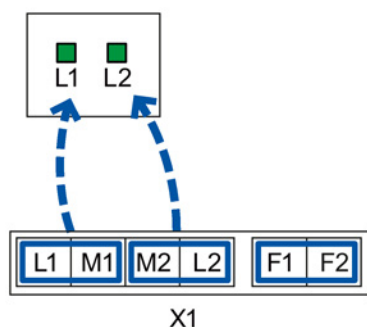
Figure 6-1 Assignment of the LED display to the pins for redundant power supply with devices with one power supply unit
