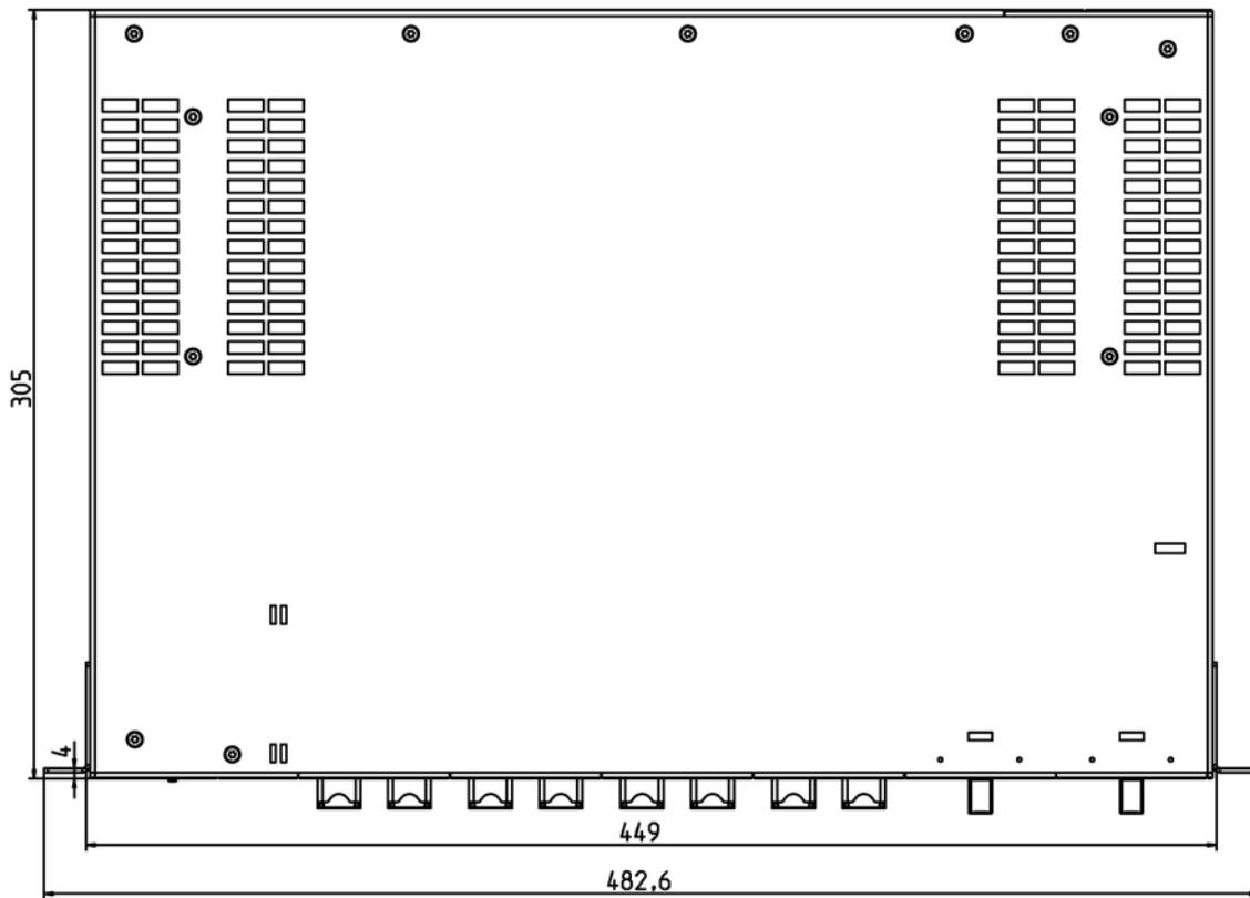
Figure 11-36 XR324-4M PoE and XR324-4M PoE TS: From above
