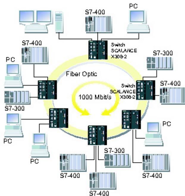
Figure 3-4 Ring with FO cable and redundancy manager
