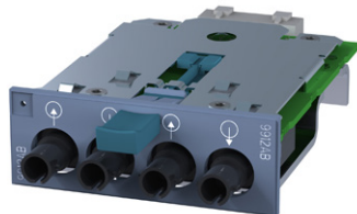
Figure 4-30 MM991-2 [9912AB]
