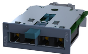
Figure 4-39 MM992-2LH [9922AN]
