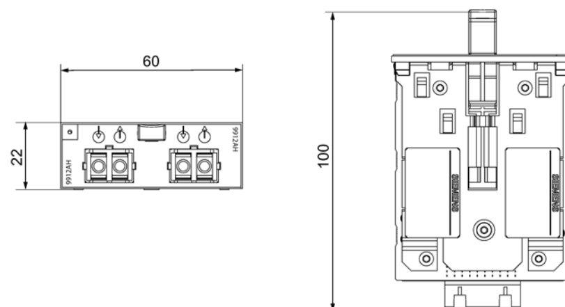
Figure 11-28 MM900 dimension drawing 7: SC RJ ports optical
