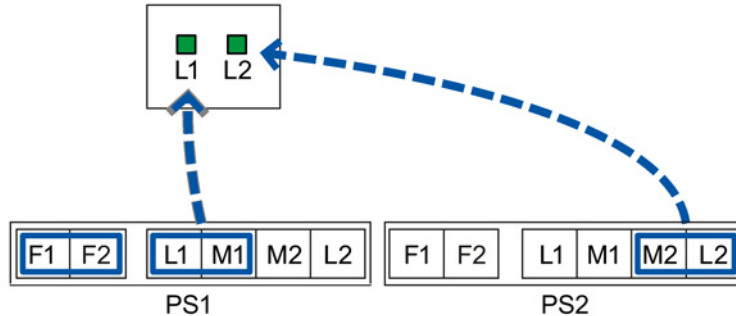
Figure 6-6 Assignment of the LED display to the pins for redundant power supply with devices with two power supply units.
