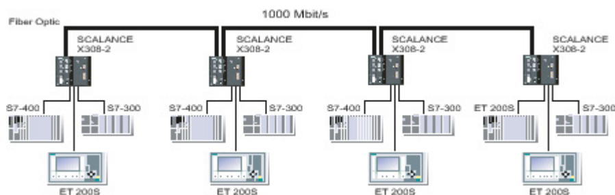
Figure 3-1 Linear structure (optical)
