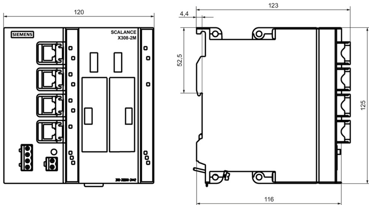
Figure 11-8 X308-2M dimension drawing
