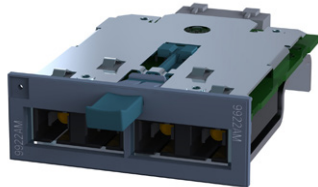
Figure 4-38 MM992-2LD [9922AM]
