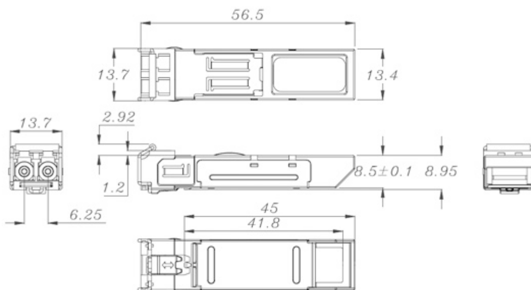
Figure 11-29 SFP dimension drawing
