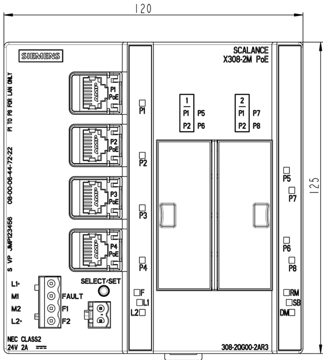
Figure 11-30 X308-2M PoE: Front view
