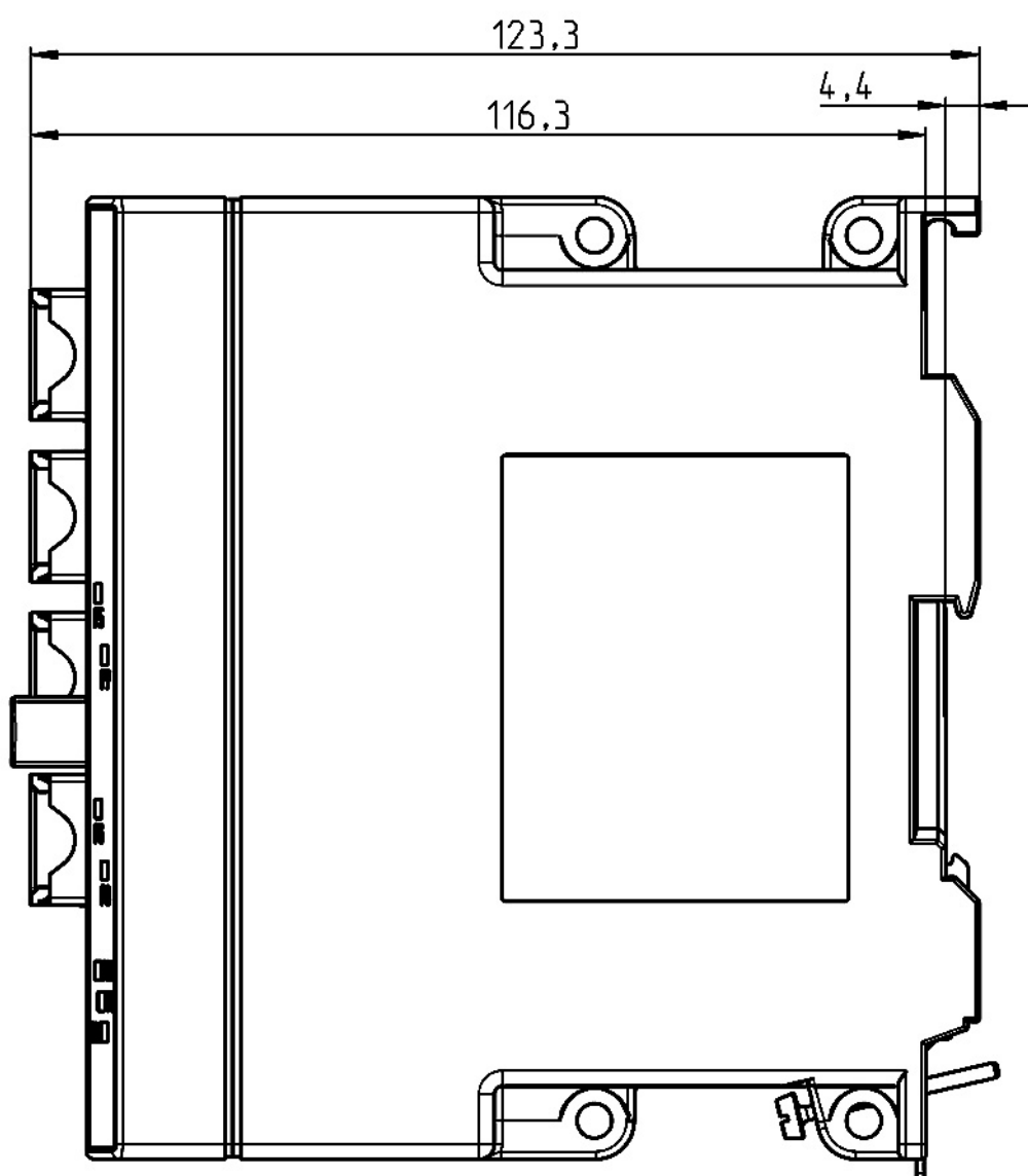
Figure 11-31 X308-2M PoE: Side view
