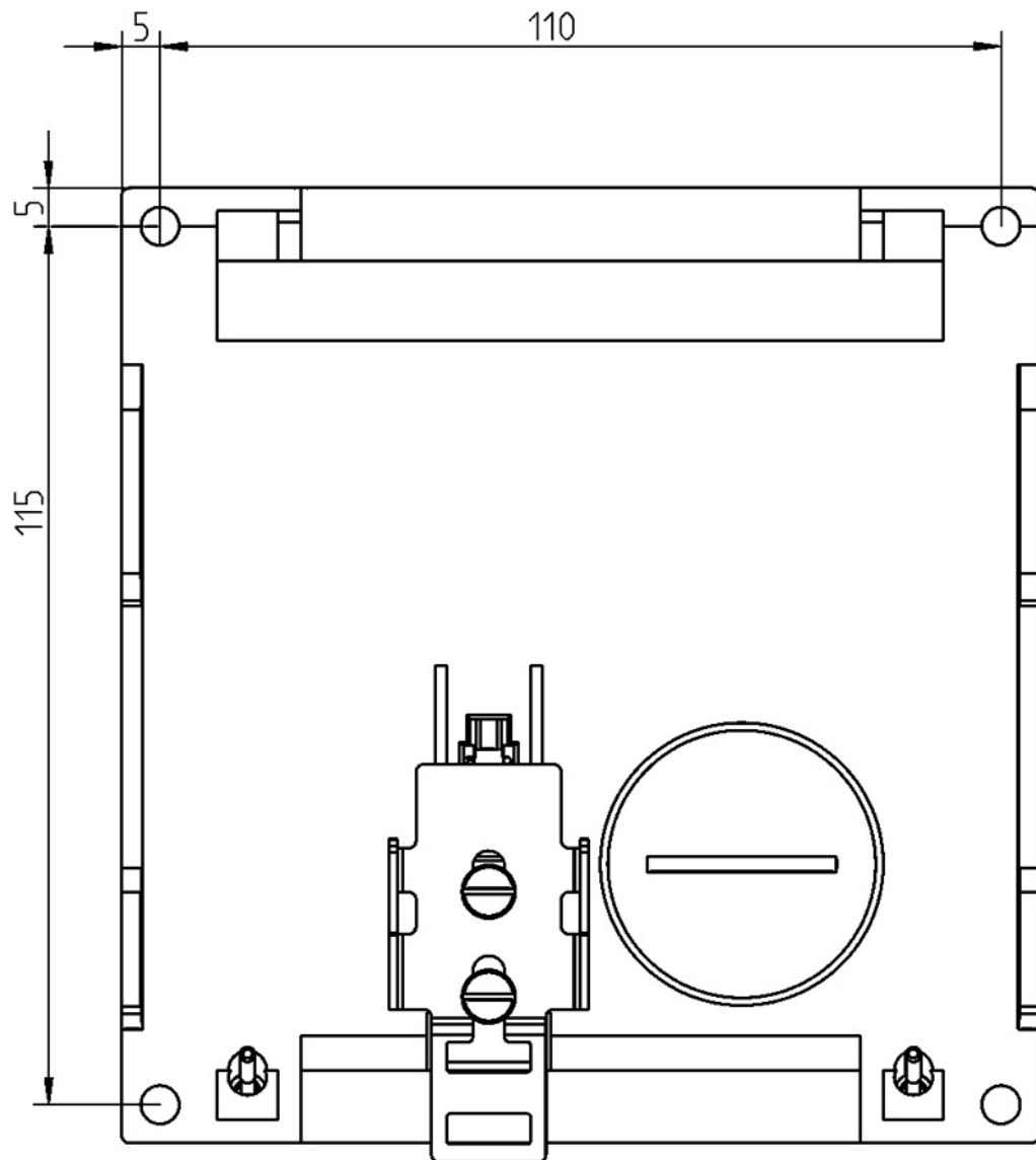
Figure 11-32 X308-2M PoE: Drilling template
