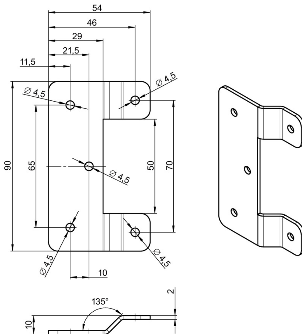
Figure 11-18 X-300EEC wall mounting (dimensions in mm)
