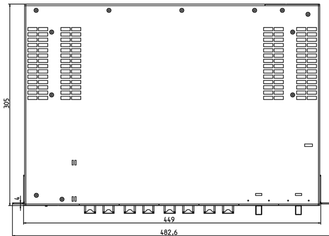
Figure 11-17 Top of the housing
