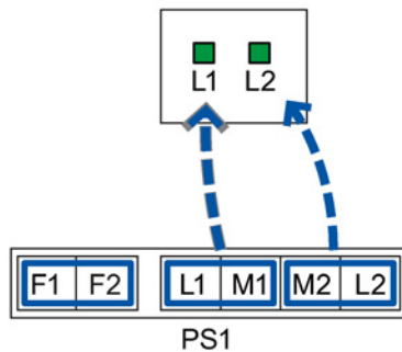
Figure 6-4 Assignment of the LED display to the pins for redundant power supply with devices with one power supply unit
