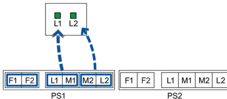
Figure 6-5 Assignment of the LED display to the pins for redundant power supply with devices with two power supply units
