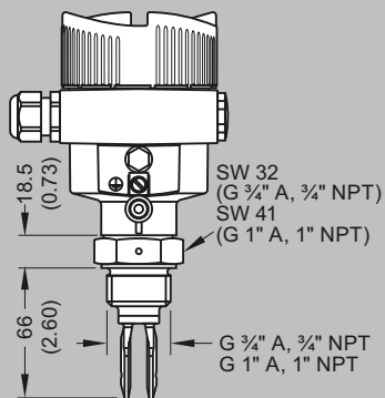
Threaded
