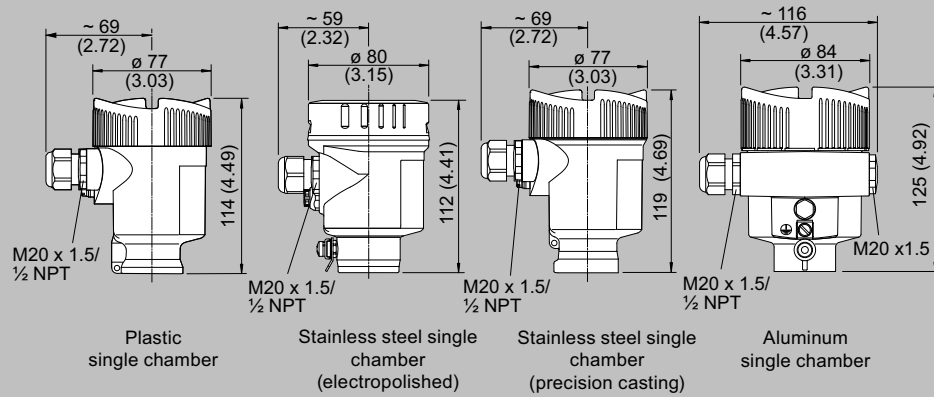
SITRANS LVL200, housing
