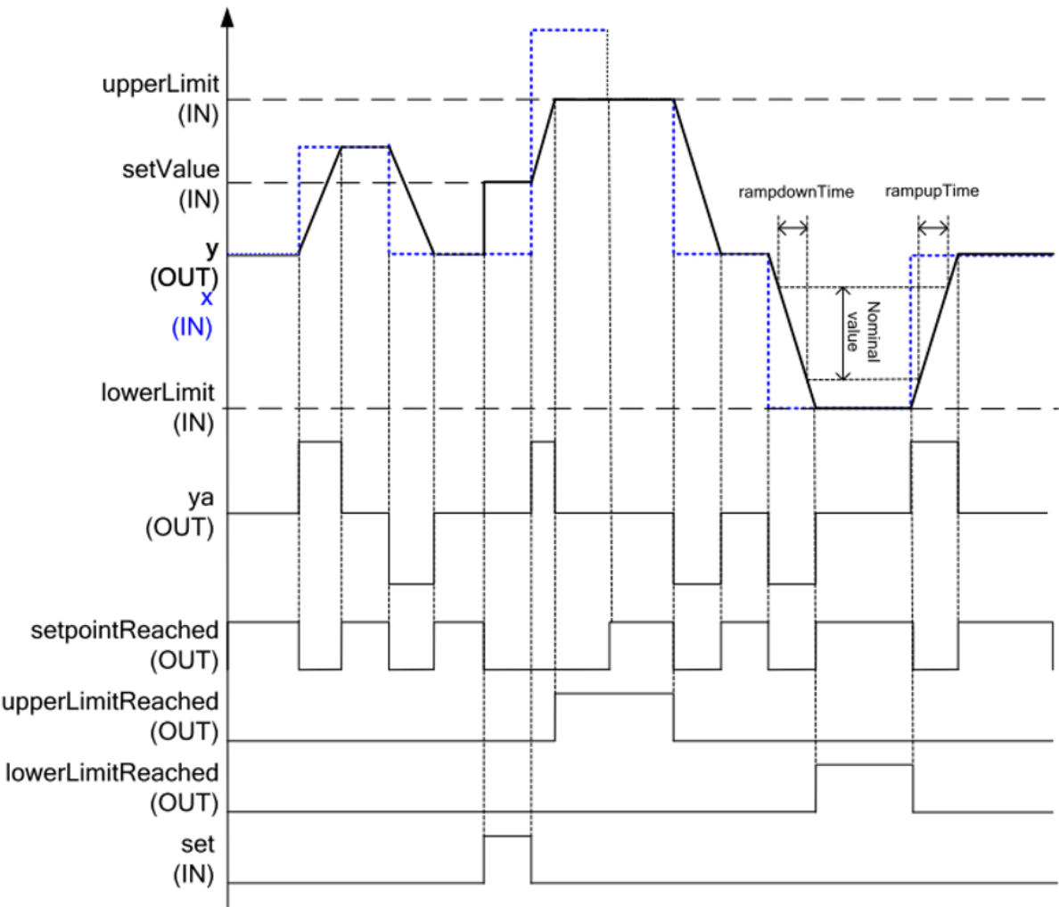
Timing Diagram - Normal Operation
