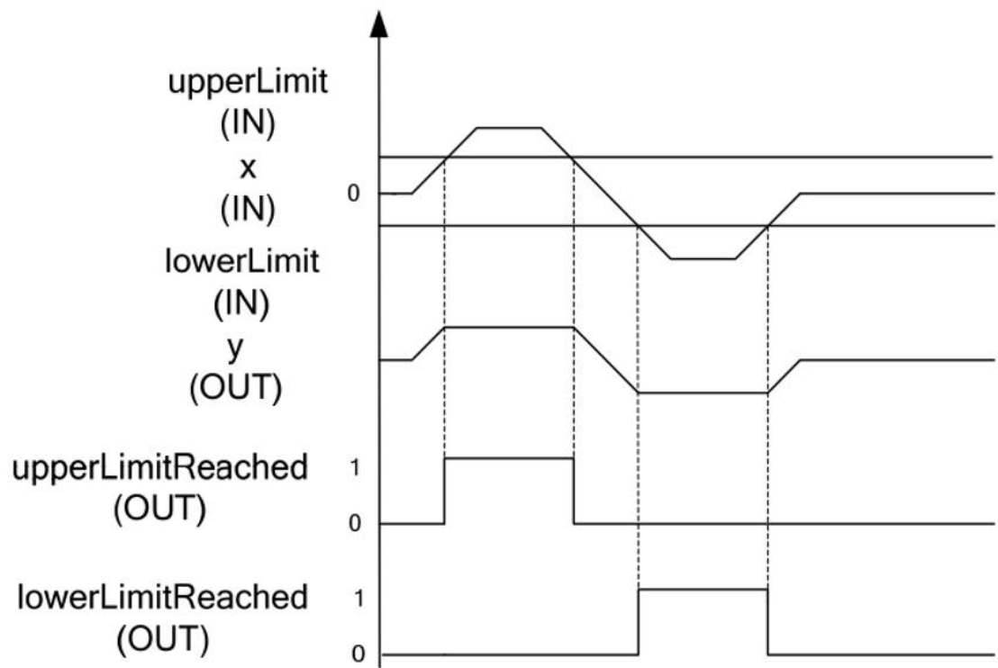
Timing diagram
