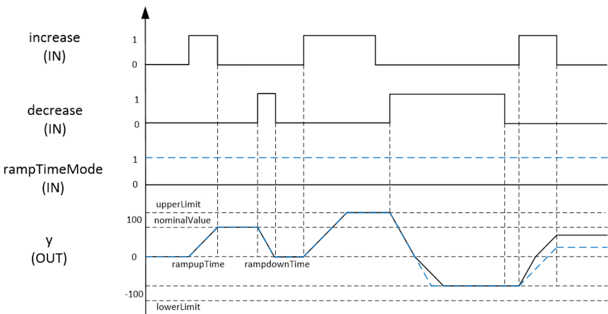
Timing Diagram - Potentiometer
