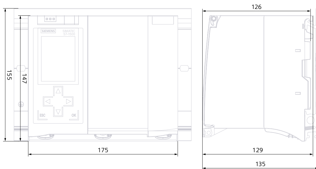
Figure A-1 Dimensional drawing of the CPU 1516T-3 PN/DP, front and side view
