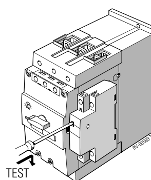
Fig. 2-8: Circuit breaker/MSP with overload relay function (frame sizes S0 to S3)
