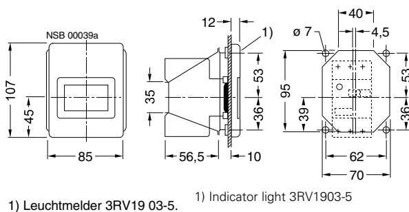
Fig. 2-55: 3RV19 13-4C (Frame size S00)
