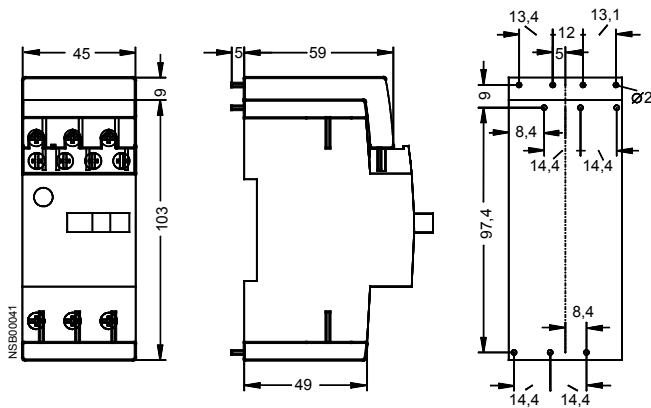
Fig. 2-57: 3RV19 18-5A/-5B (Frame size S00)
