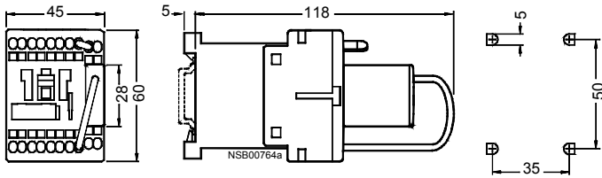
Fig. 3-117: 3RT10 17, 3RH 11
