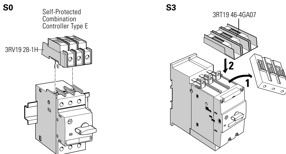
Fig. 2-21: Terminals for "Combination Motor Controller Type E"
