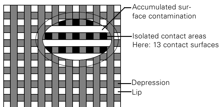
Fig. 3-6: Contact areas
