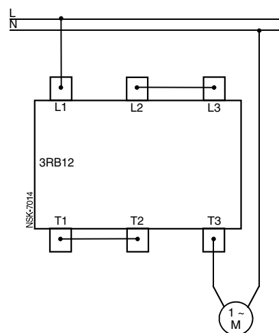
Fig. 4-30: Wiring diagrams for single-phase motors using 3RB12
