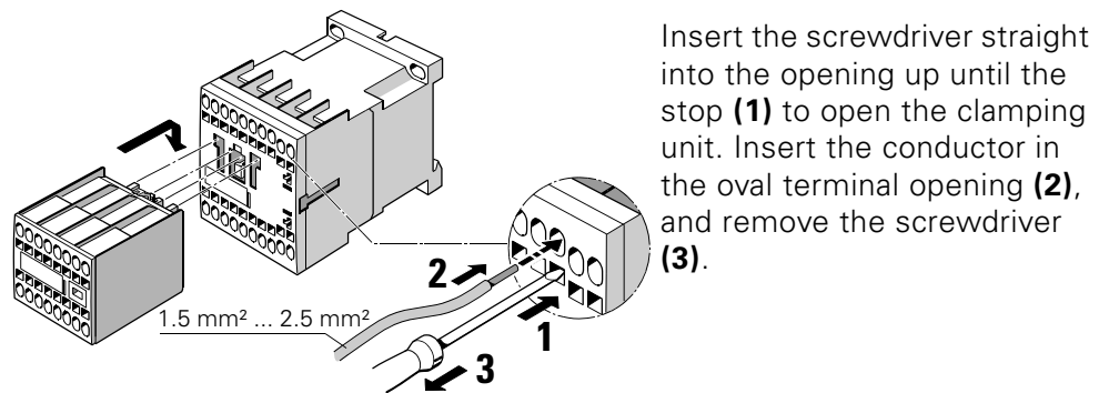
Fig. 3-82: Cage Clamp terminals
