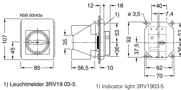
Fig. 2-56: 3RV19 23-4B, 3RV19 23-4E (Frame size S0, S2, S3); 3RV19 23-4G (only for Frame size S0)
