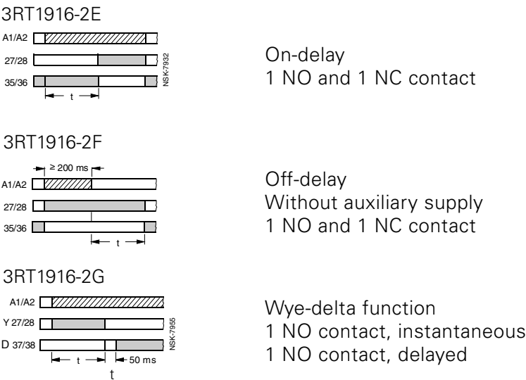
Fig. 3-51: Function diagrams of the time-delay auxiliary switches (frame size S00)
