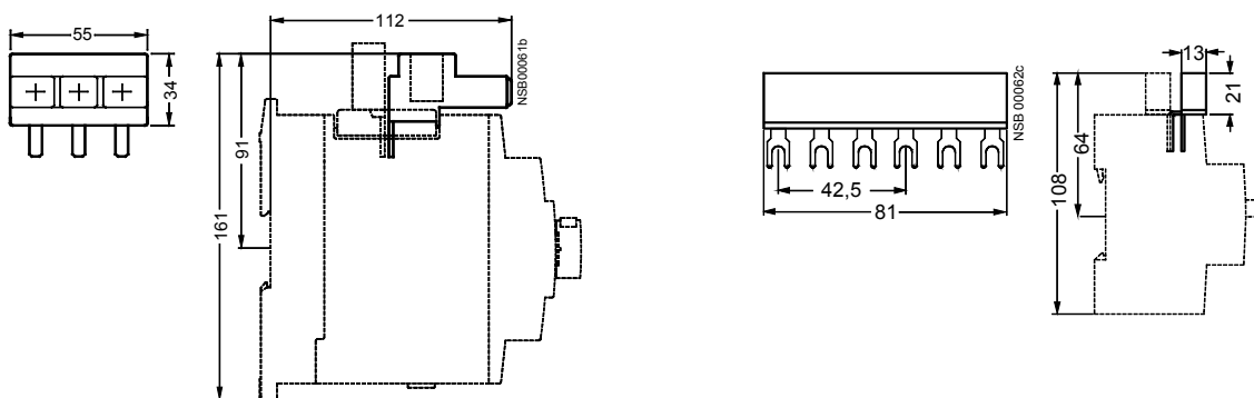
Fig. 2-77: 3RV19 35-5A Connection from above (for frame size S2)
