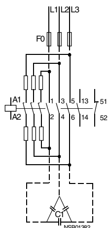
Fig. 3-19: Capacitor contactors, circuit diagram
