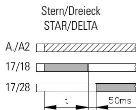
Fig. 7-13: 3RP15 74 function diagram
