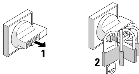
Fig. 2-20: Locking the thru-the-door rotary operator outside the enclosure
