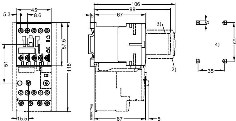
Fig. 3-96: 3RT1. 10 1/3RH11 contactors
