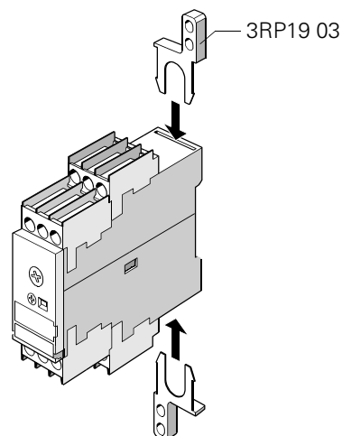
Fig. 7-14: Panel mounting
