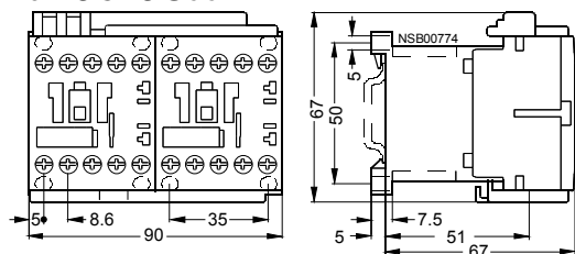
Fig. 3-129: Reversing contactor combinations
