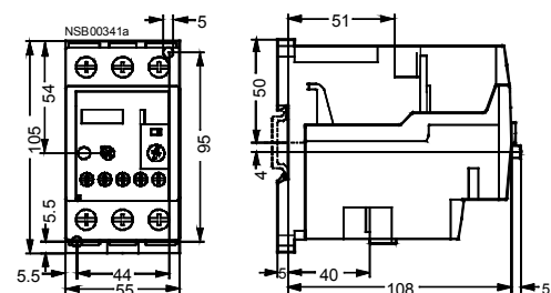
Fig. 4-35: 3RU11 36-..B., 3RB10 36-..B., (Frame size S2) with adapter for stand-alone installation
