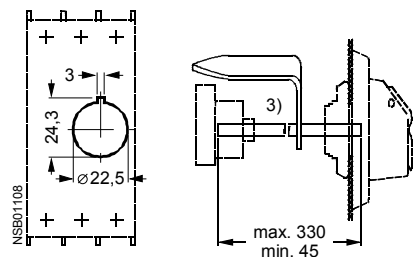
Fig. 2-59: 3RV19 26-0. (Long shaft (with support) for circuit breaker/MSP Frame sizes S0, S2, S3)
