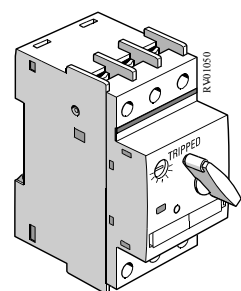
Fig. 2-4: Tripped position, 3RV (example: frame size S0)
