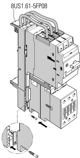
Fig. 5-13: Busbar system, mounting/removal (frame sizes S00 to S2)
