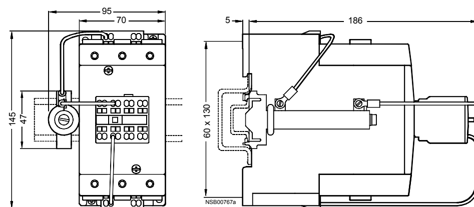
Fig. 3-120: 3RT104
