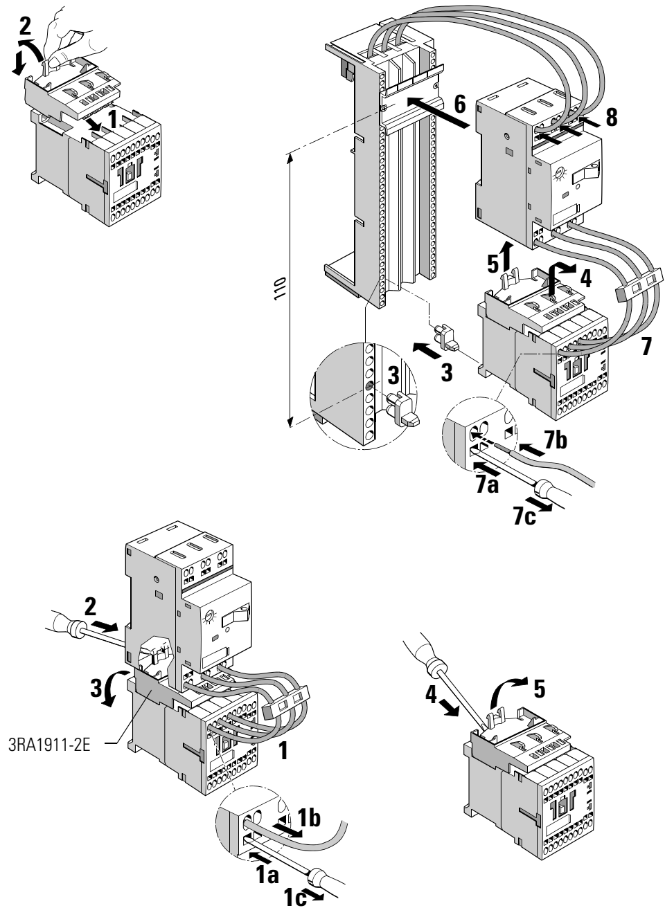
Fig. 5-9: Self-assembly, busbars, direct starters (frame size S00/S0, Cage Clamp)
