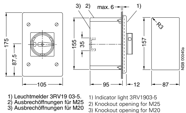
Fig. 2-54: 3RV19 23-2DA00/-2GA00 (Frame size S0)
