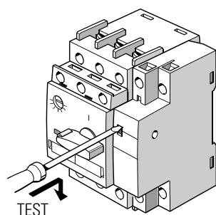
S0: 3RV11 21-....
