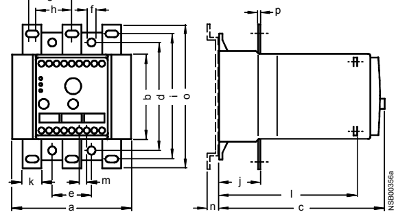
Fig. 4-38: 3RB12 5. / 3RB12 62
