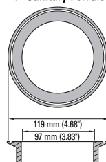
4" Sanitary Ferrule
