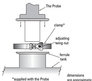
4" Sanitary Ferrule
