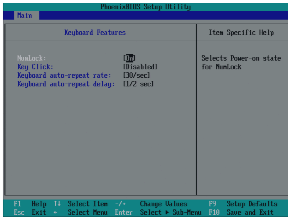
图 17-12 “Keyboard Features (键盘功能)” 域
