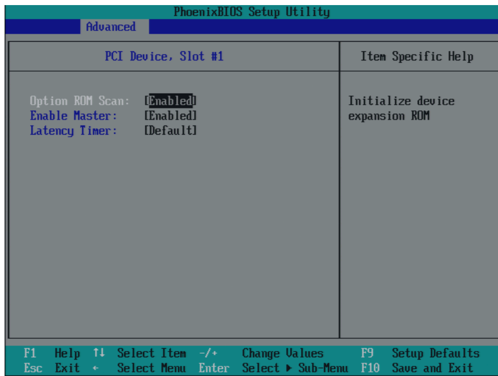
图 17-19 “PCI Devices, slot #1 (PCI 设备, 1 号插槽)” 子菜单 (实例)
