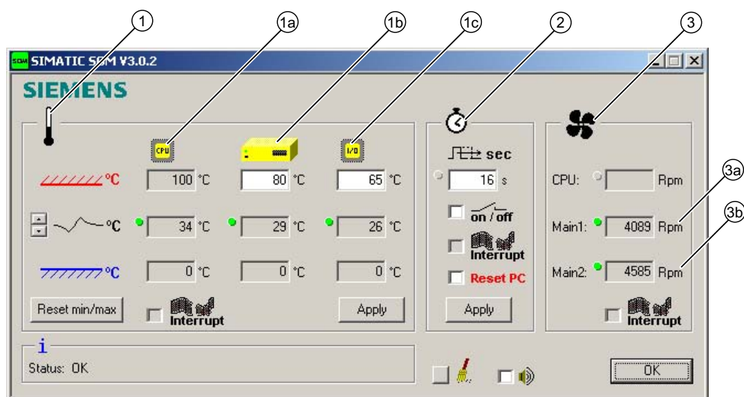
图 11-1 Safecard on Motherboard
