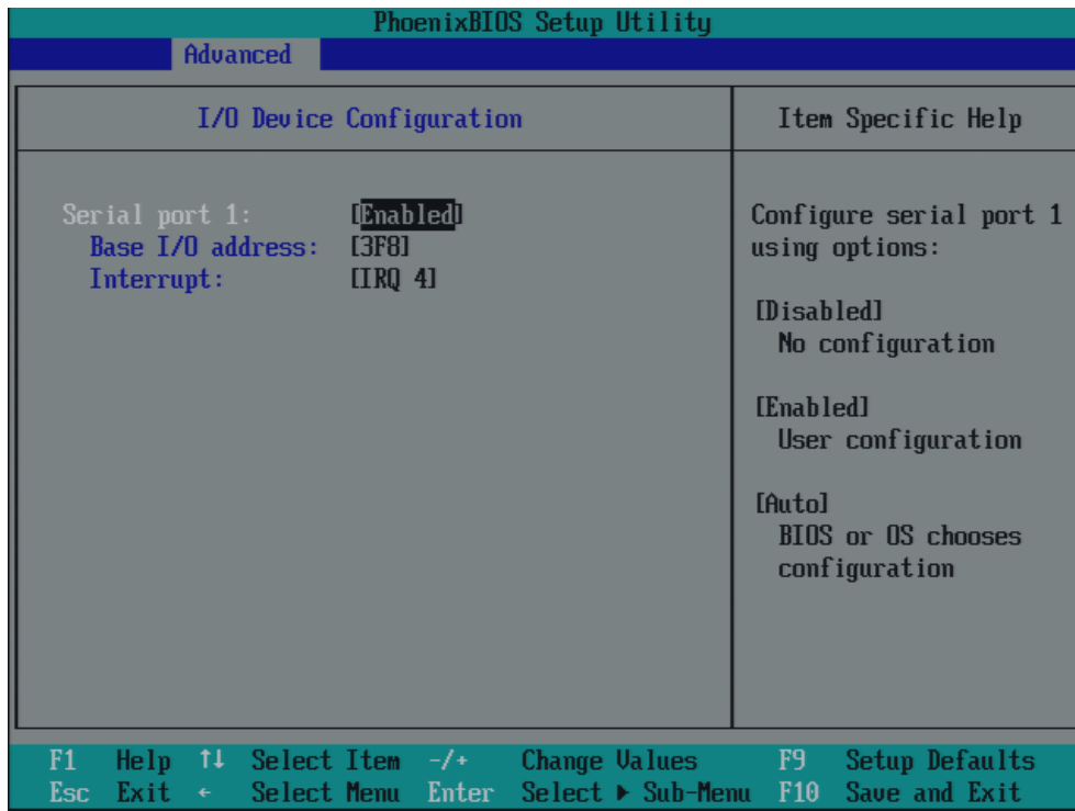
图 17-17 “I/O Device Configuration (I/O 设备组态)” 子菜单
