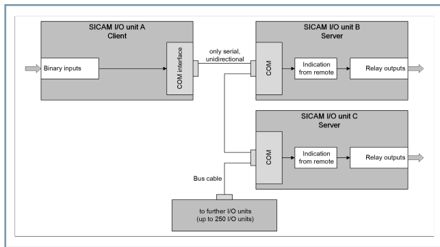
[hw_30-Mirror_unidirect-trans-sicam-io-unit_2_en_US]
