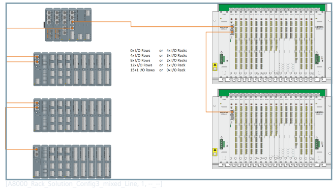
Figure 2.4/4 SICAM A8000 Rack – Combination Example 2
