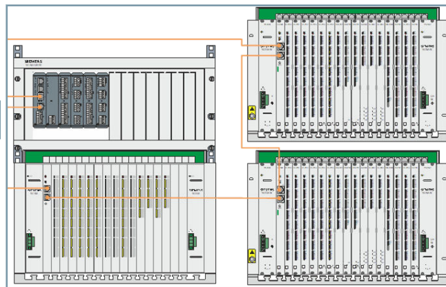
Figure 2.4/2 SICAM A8000 Rack – Swing-Frame Mounting
