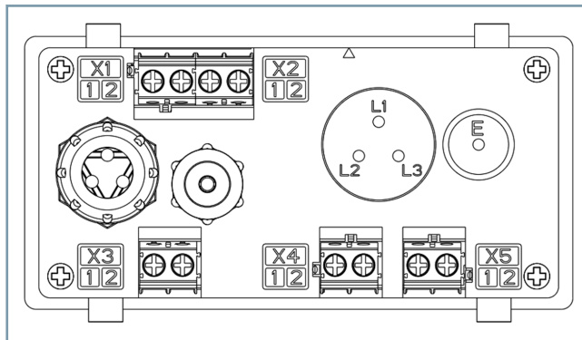
Figure 7.3/3 Rear View
