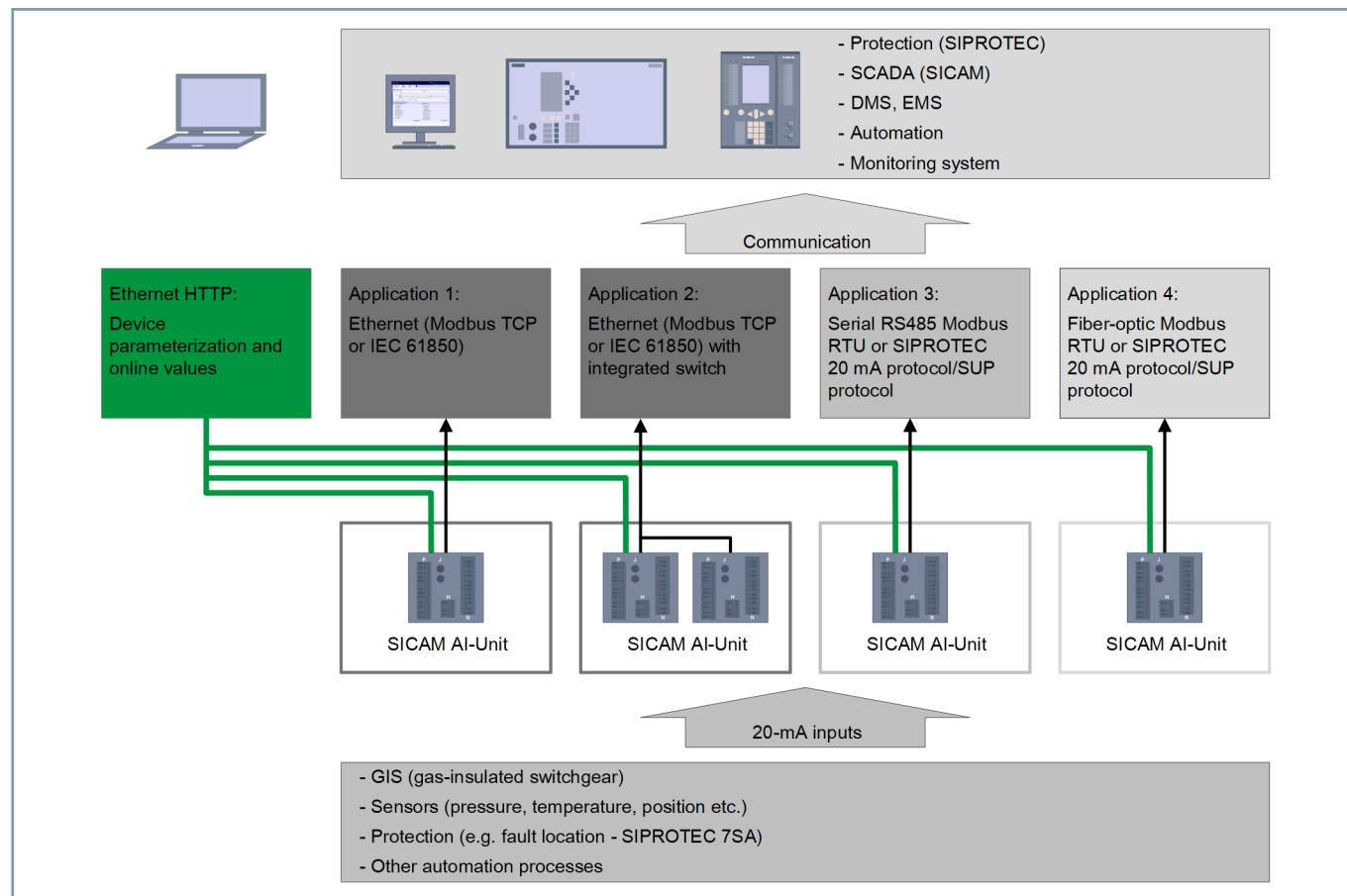
Figure 8.2/2 Application Example
