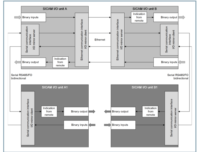
[hw_log-config_of_io-to-bo_2_en_US]
