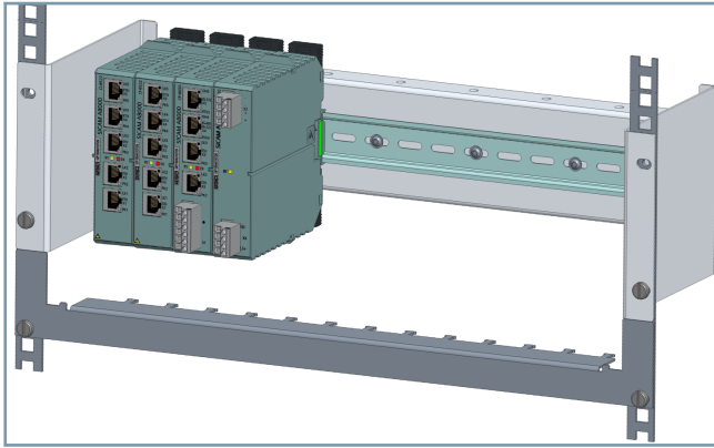
Figure 2.4/5 SICAM A8000 Module Rack CM-8846
