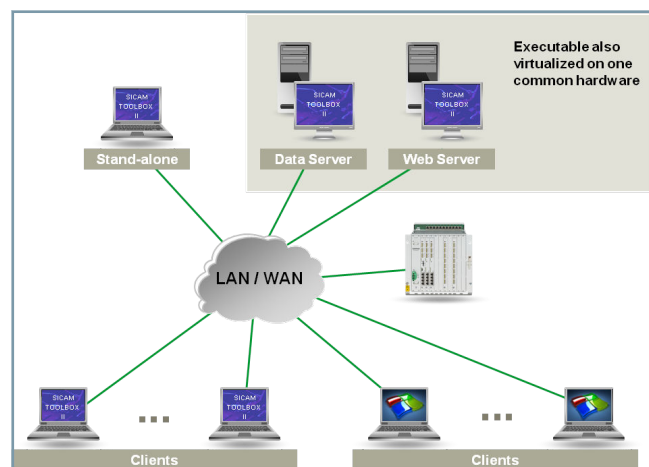
Figure 4.2/4 SICAM TOOLBOX II Server/Client Configuration
