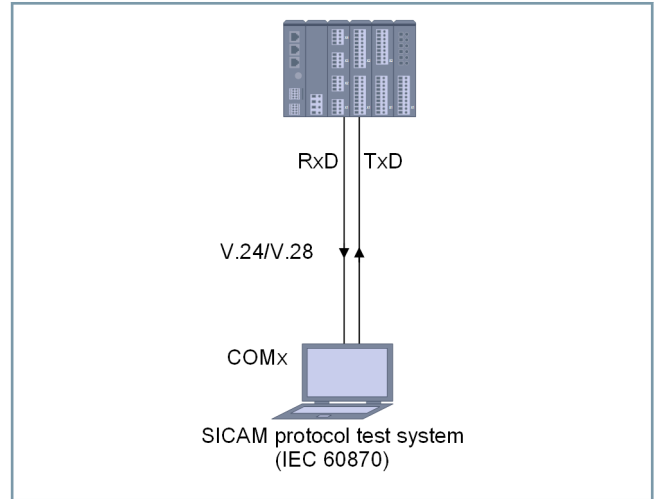
[dw_sicam-protocol_simulation_iec60870_4_en_US]
