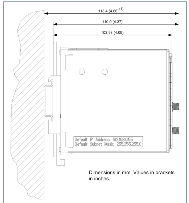
Figure 7.7/2 Dimensional Drawing
