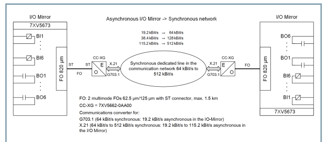
Figure 8.1/10 Binary Signal Exchange via a Communication Converter with a G.703.1-/X.21 Interface via a Communication Network
