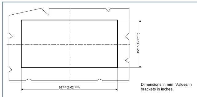
Figure 7.3/4 RMU Panel Cut-Out
