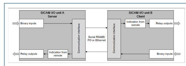
[diw_Io-Mirror_bidirect-trans-2-device_2_en_US]
