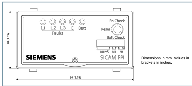
Figure 7.3/2 Front View
