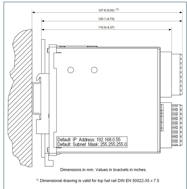
Figure 8.2/3 Dimensions of the SICAM AI-Unit 7XV5674
