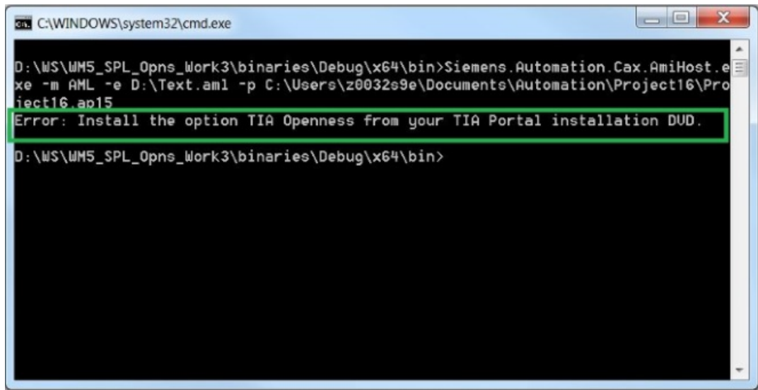
图 8-3 OpennessNotInstalled-Commandline
