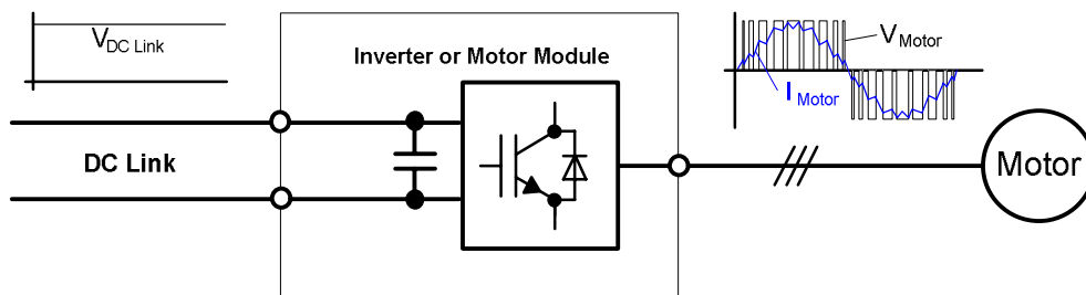
SINAMICS S120 inverter or Motor Module
