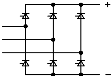
6-pulse three-phase bridge circuit with thyristors
