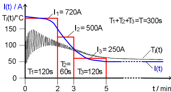
Time characteristic of the motor current I(t) and the junction temperature T_j(t) of the IGBT chips during starting
