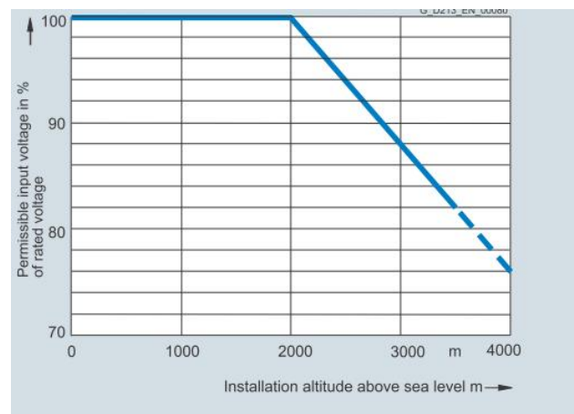
Input voltage derating as a function of altitude
