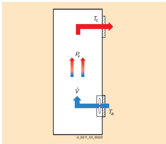
Cooling of a cabinet by forced ventilation
