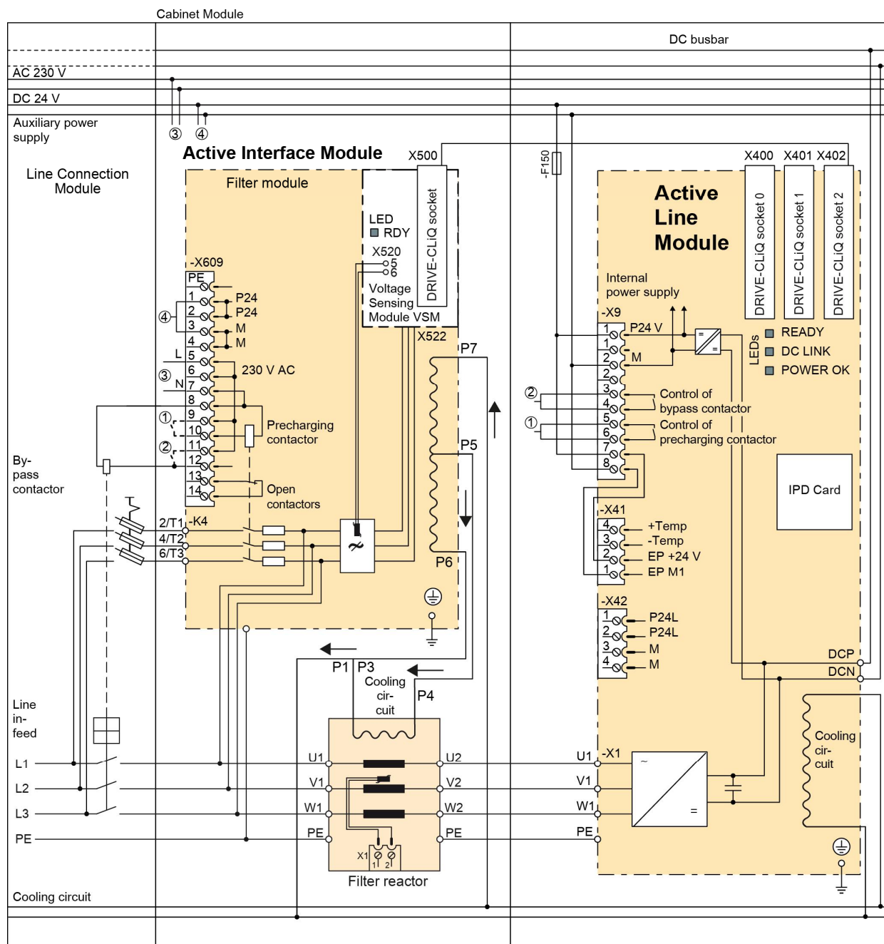
Example of a liquid-cooled Active Line Connection Module (> 800 A) with circuit breaker in the Line Connection Module and a liquid-cooled Active Line Module including liquid-cooled Active Interface Module
