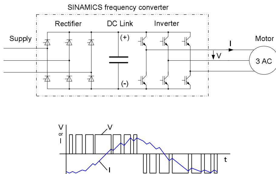
Principles of operation of SINAMICS frequency converters and schematic representation of output voltage V and motor current I
