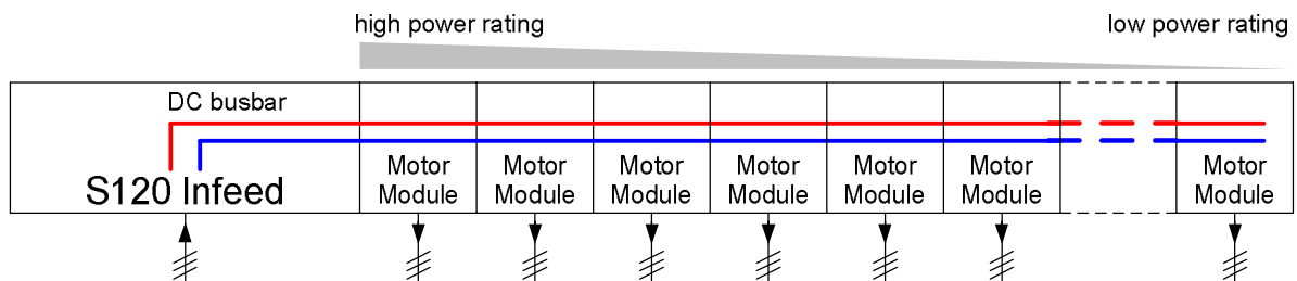
Example 1: Linear arrangement of a DC busbar with the Infeed at the left-hand end of the configuration
