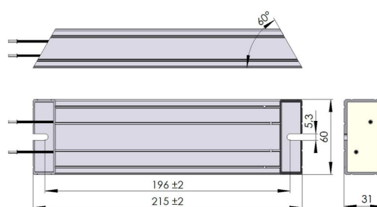
Dimensions of resistor 6SL3000-0KH14-0AA0 / 4.0 Ω
