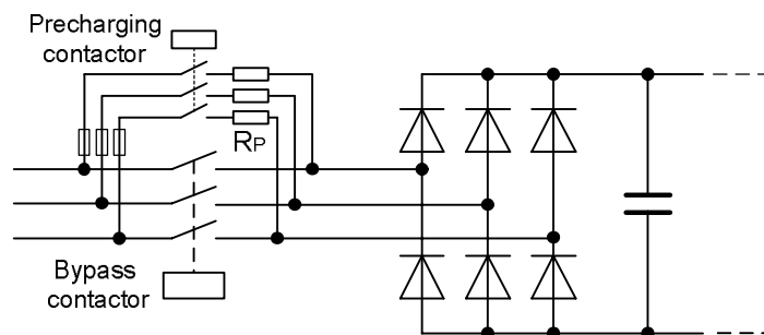
Precharging with S120 Basic Line Modules equipped with diodes via precharging contactor and precharging resistors
