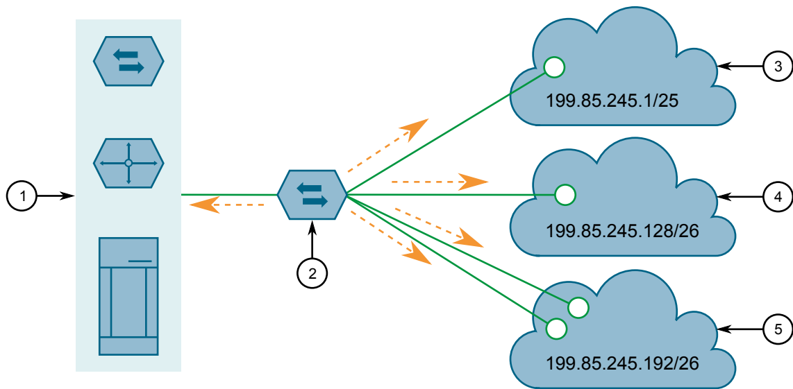
Figure 86 : Communications inter-VLAN
