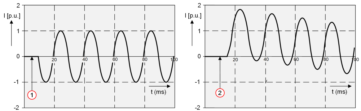
Figure 1-14 Reduction of the Inrush Currents when Switching on a Grounded Reactance Coil
