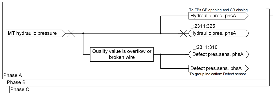
Figure 3-14 Logic Diagram of the Pressure Supervision
