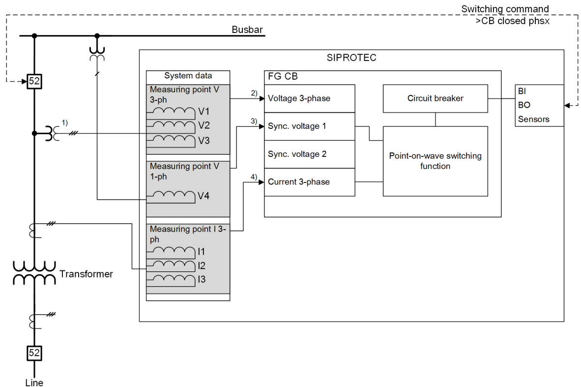
Figure 1-10 Transformer
