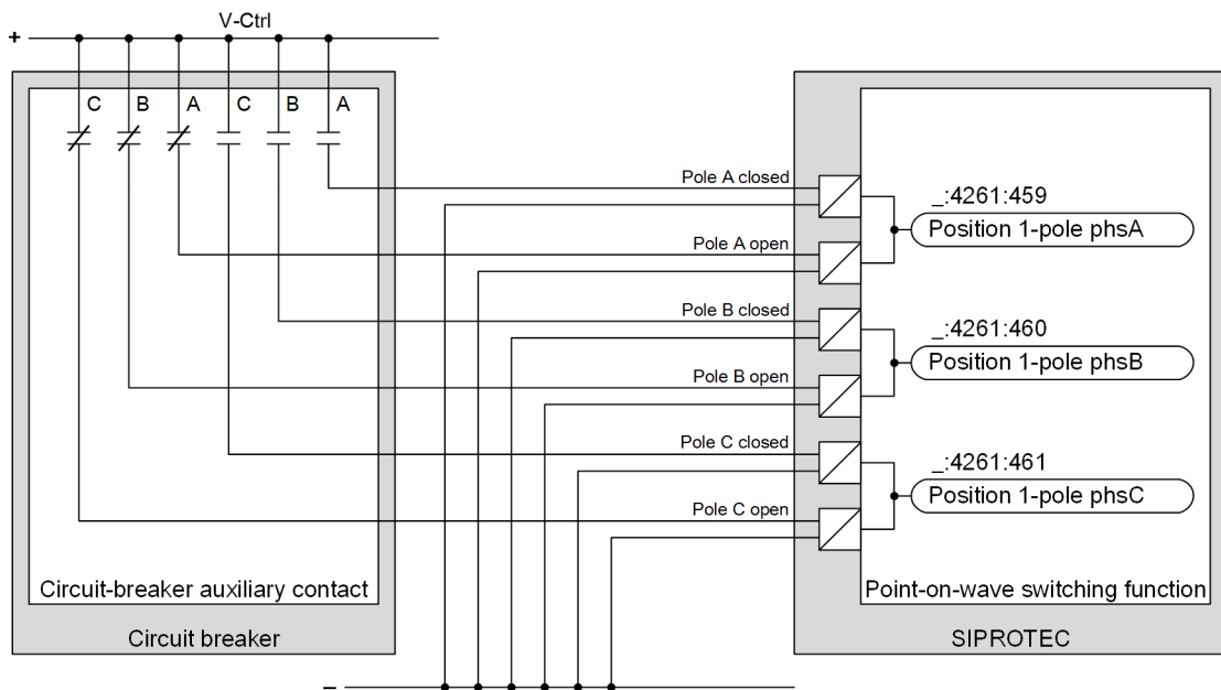
Figure A-5 Connection of Non-Siemens Circuit-Breaker Auxiliary Contacts for PoW Switching-Accuracy Supervision
