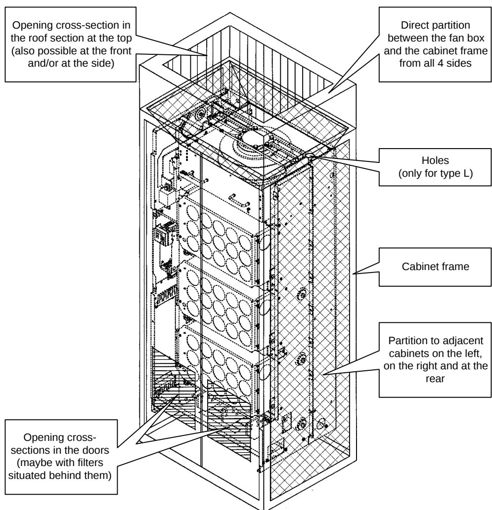
Fig. 5-8 Partition measures
