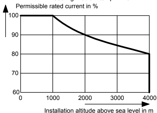
Fig. 13-1 Derating curves
