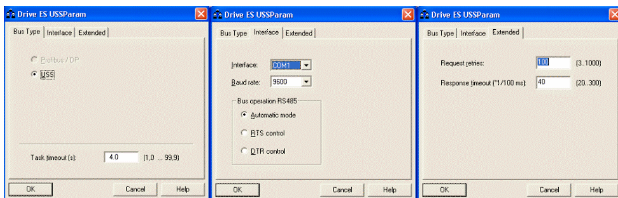
Fig. 8-4 Interface configuration
