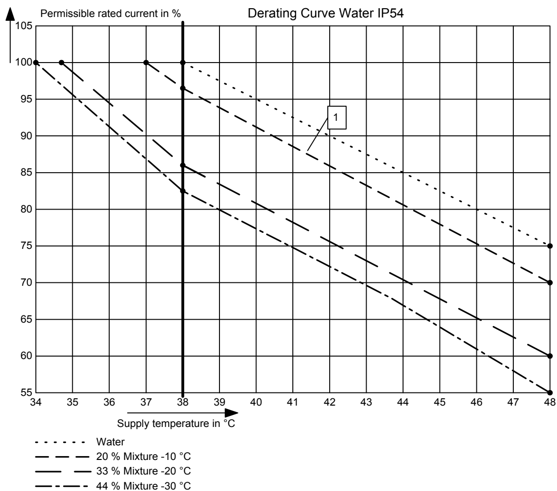
Fig. 13-5 Reduction curve 2 applying to installation in IP54 cabinets
