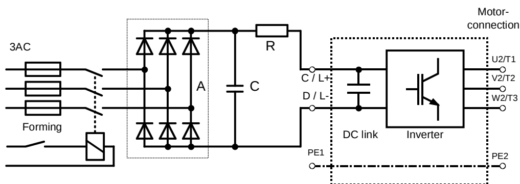
Fig. 12-1 Forming circuit
