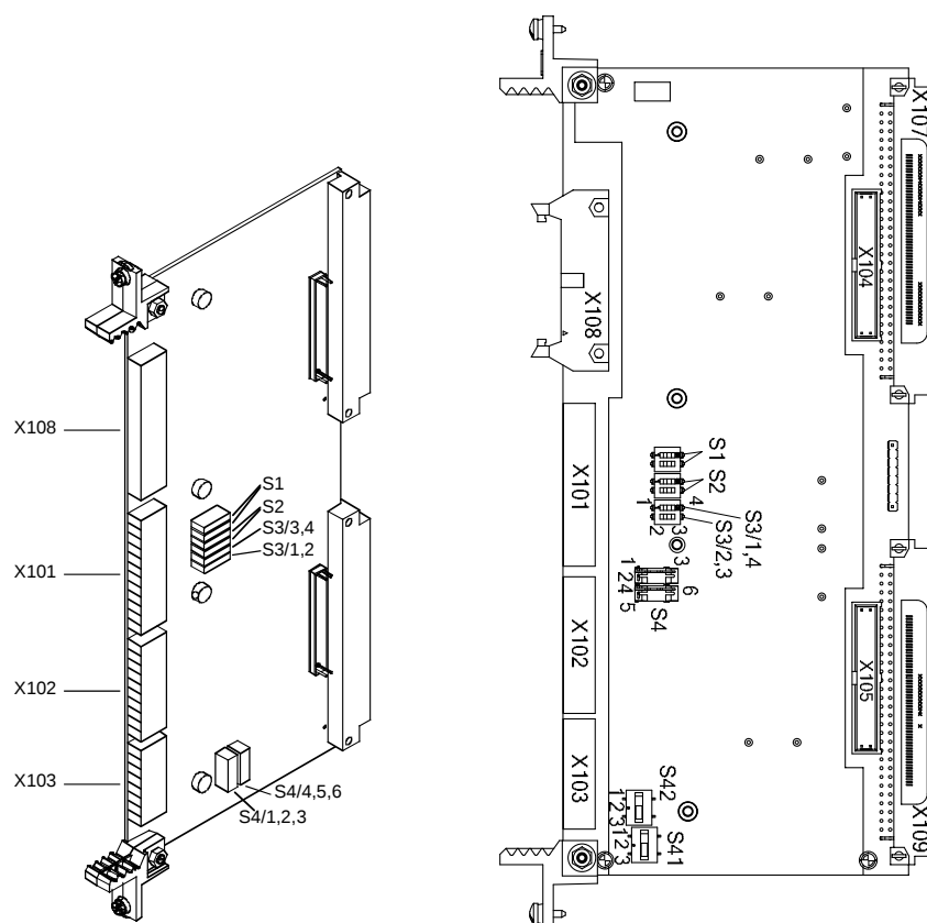
Fig. 7-4 View of the CUVV
