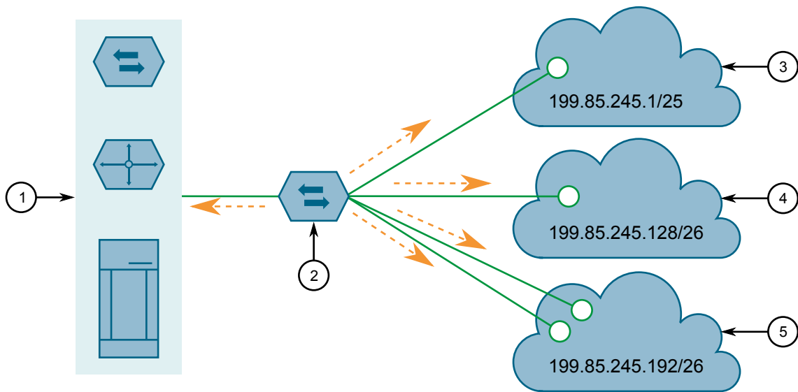
Figure 77 : Communications inter-VLAN
