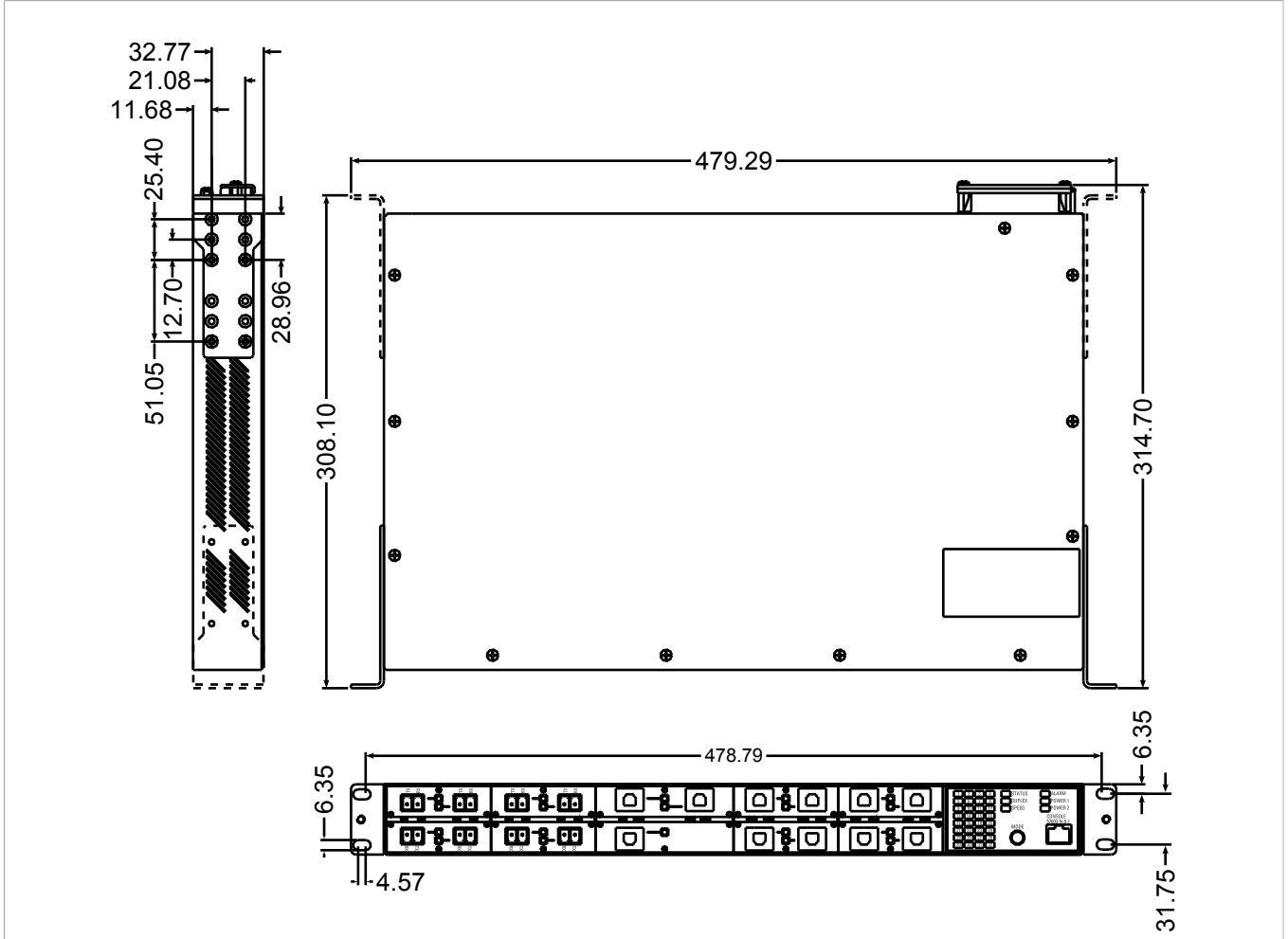
Figure 38: Rack Mount Dimensions
