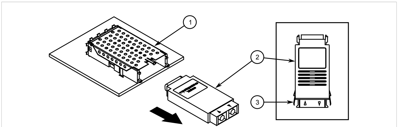
Figure 35: Removing a GBIC Optical Port
