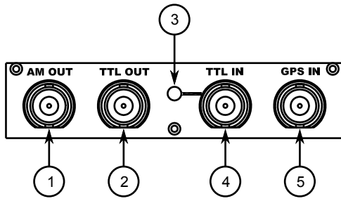
Figure 36: PTP Module
