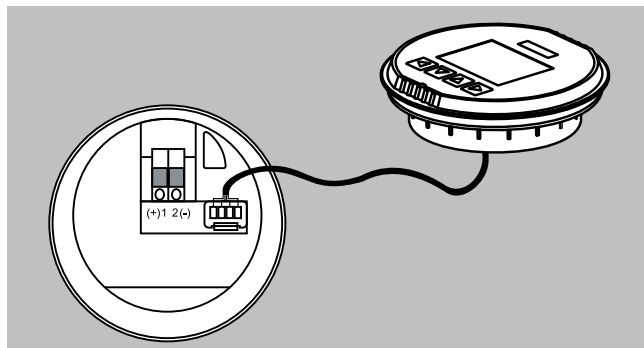
SITRANS LR150 connections
