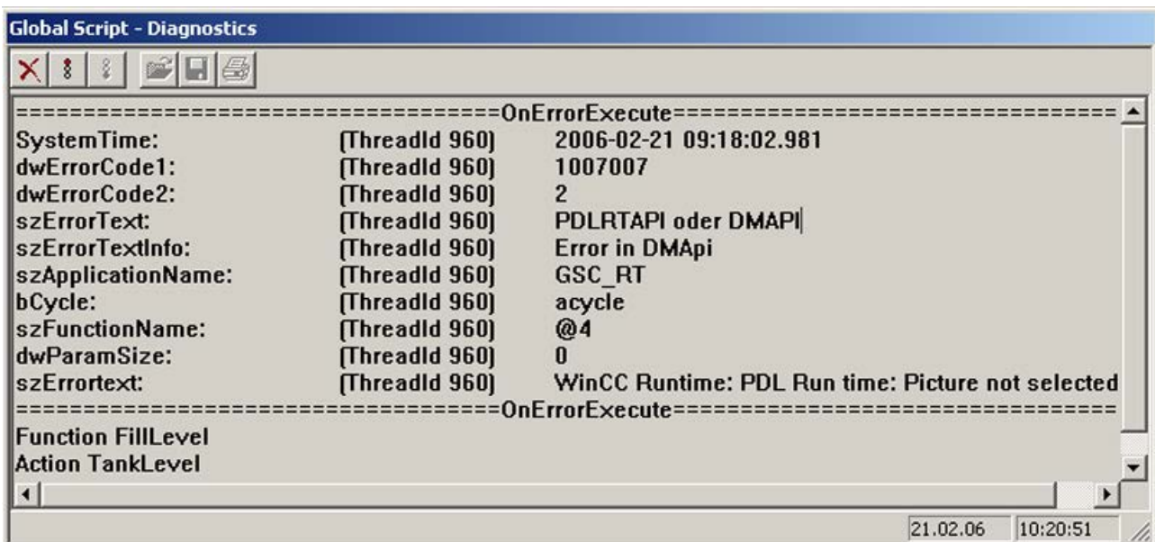
Image 2-1 Diagnose window of GSC Diagnose
