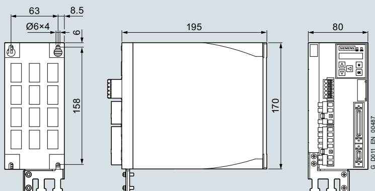
SINAMICS V90, 200 ... 240 V 1 AC/3 AC, frame size FSC
