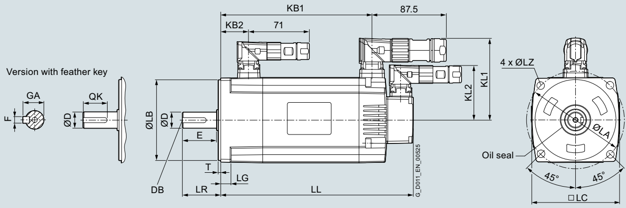
SIMOTICS S-1FL6 Low Inertia servomotor, shaft height 50
