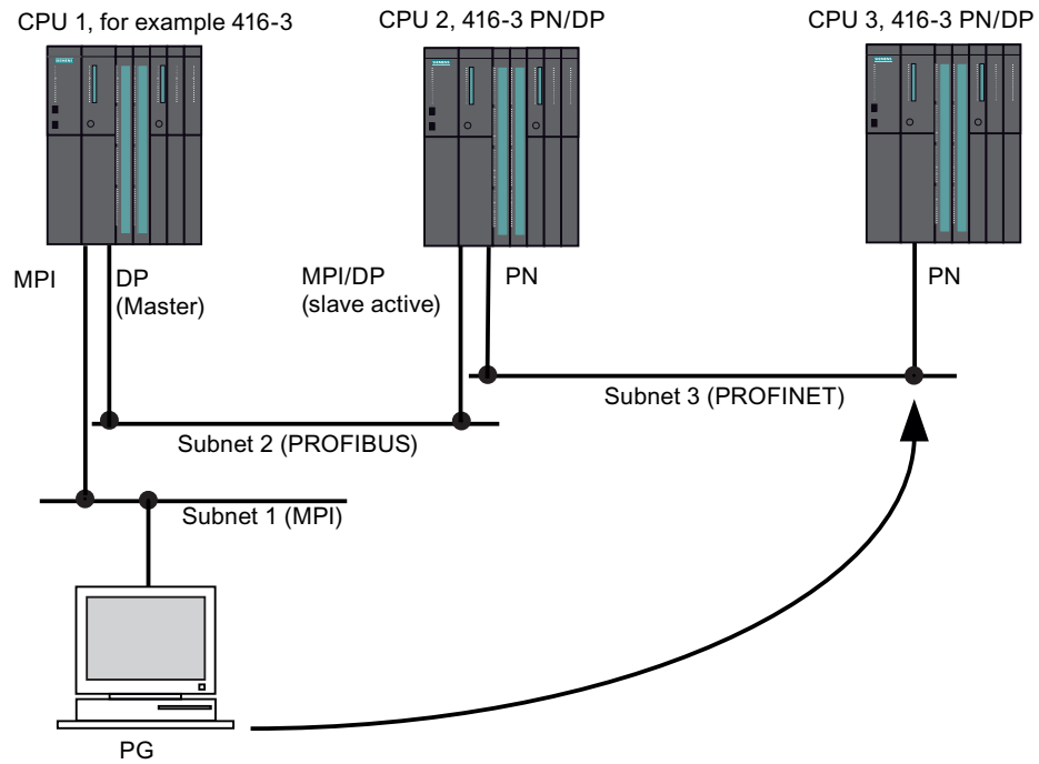
Figure 4-2 S7 routing gateways: MPI - DP - PROFINET
