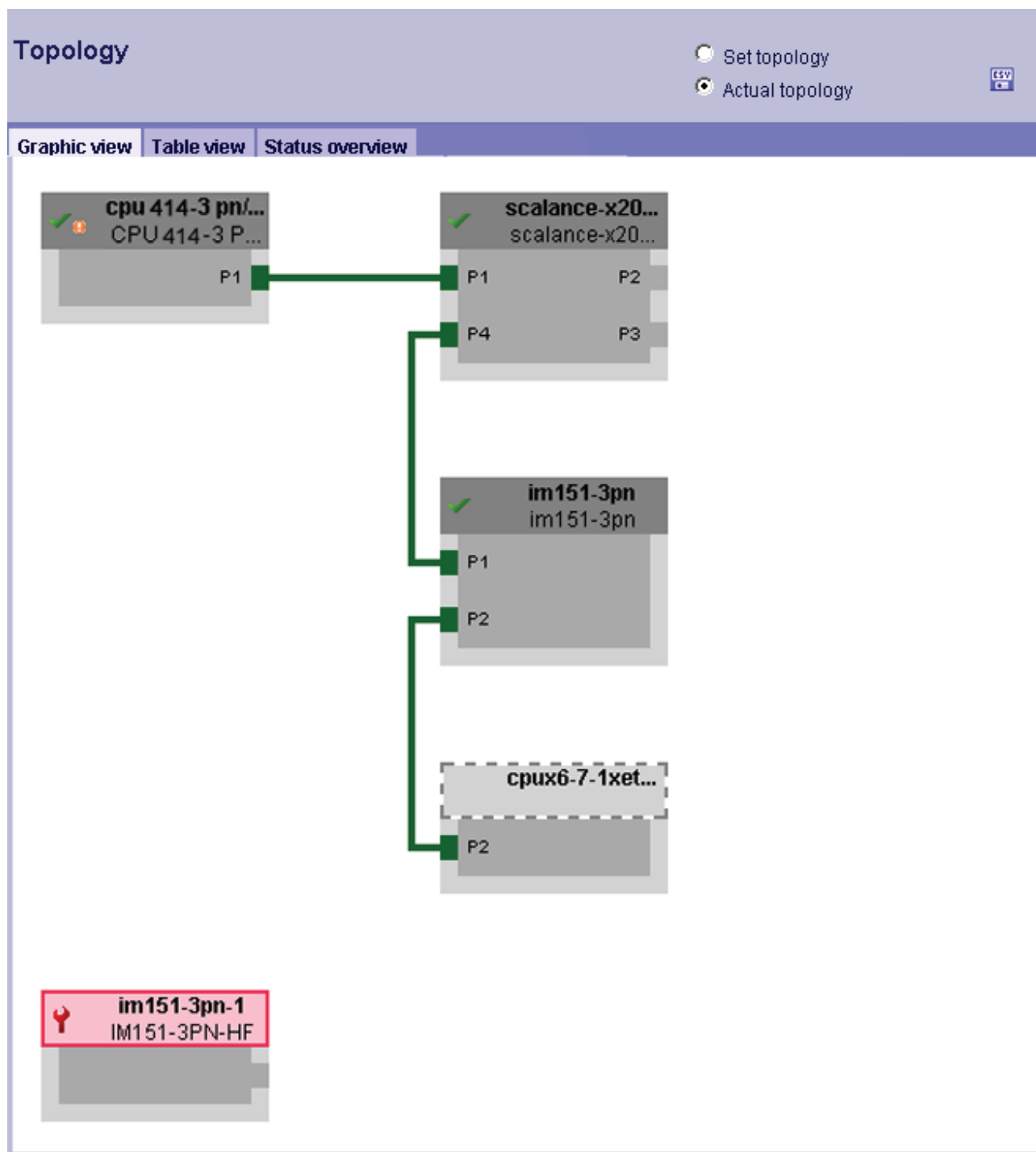
Figure 4-25 "Actual topology" with failed device
