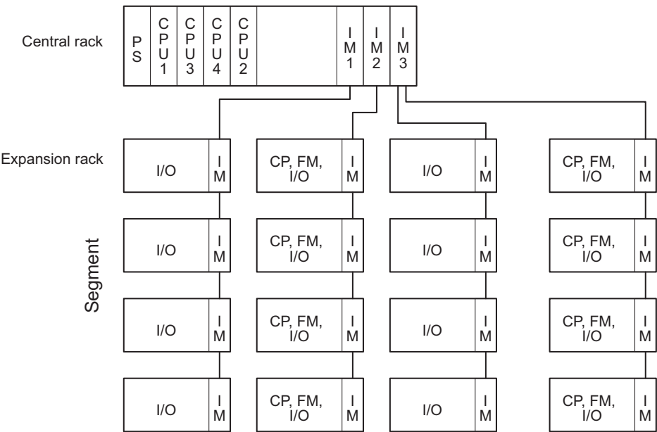
Figure 3-2 Example of multicomputing
