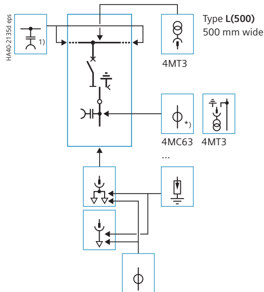
Vacuum circuit-breaker
