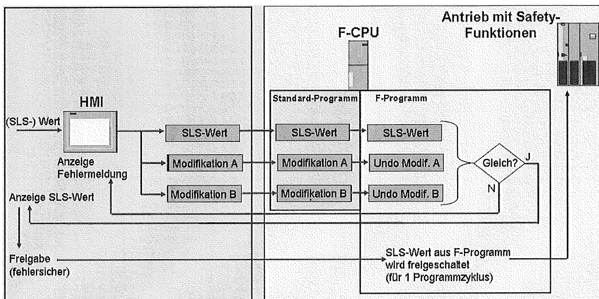
Figure 1: System overview of the configuration environment SIMATIC SLS with HMI
