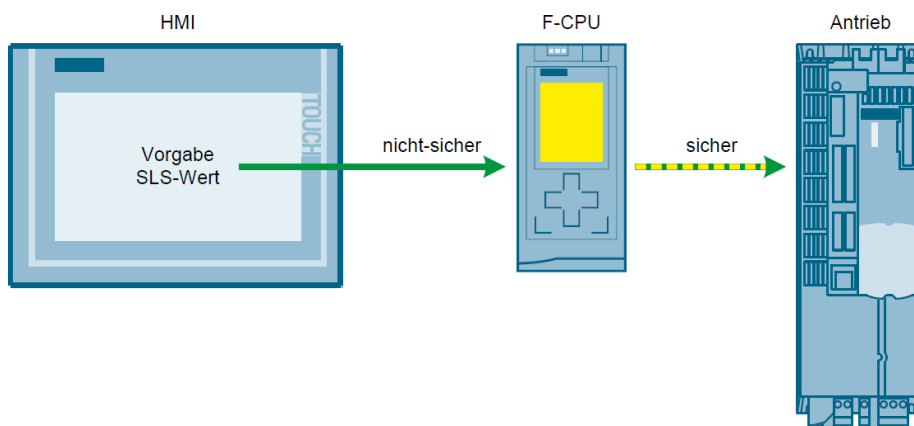
Figure 1: Overview of the Configuration Environment SIMATIC SLS with HMI
