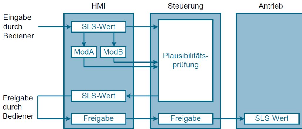
Figure 2: Basic functionality of the SIMATIC SLS with HMI
