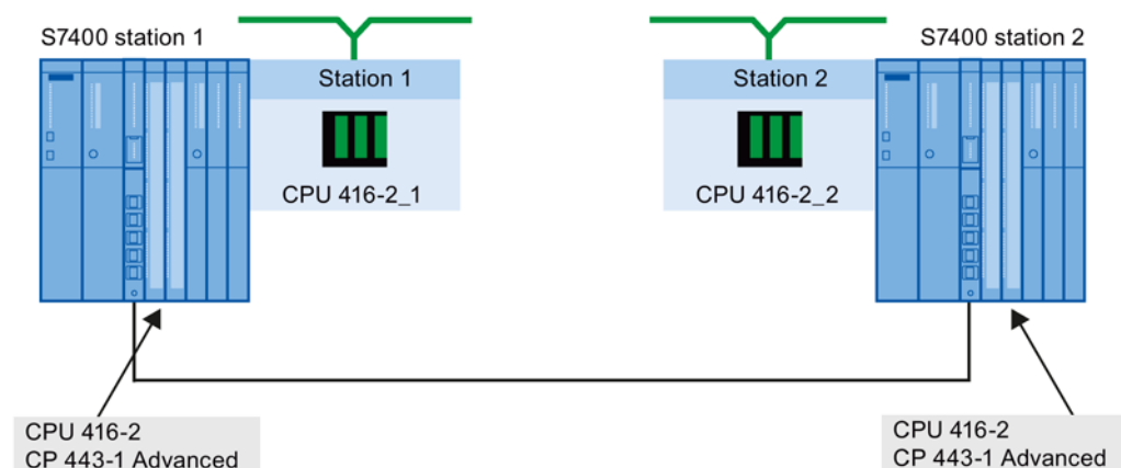
Image 2-2 Measurement setup with 2 S7-400s
