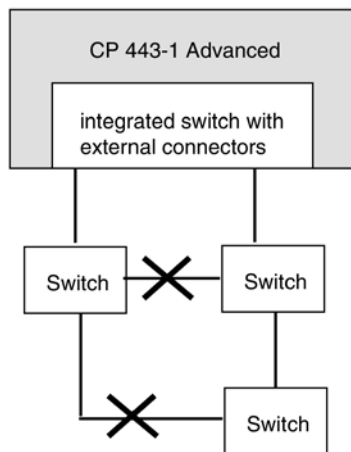
Image 5-1 Connecting switches
