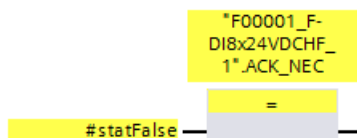
Figure 3-19: Programming automatic reintegration
