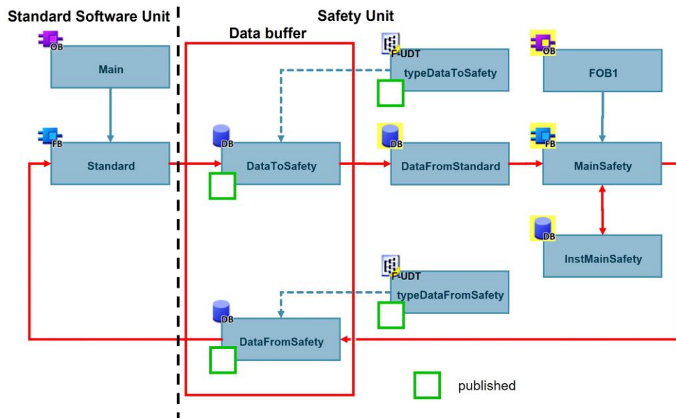
Figure 3-14: Overview diagram for data exchange between Safety Unit and Standard Unit
