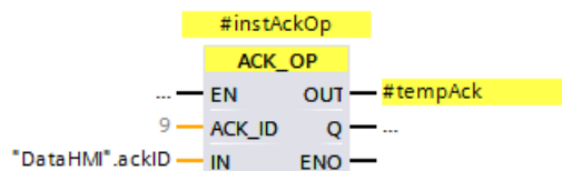
Figure 3-13: System block "ACK_OP"
