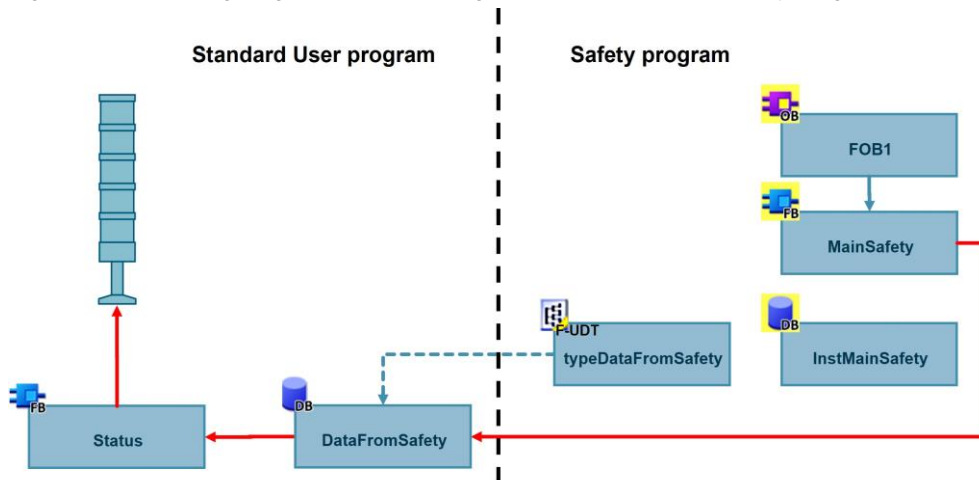
Figure 3-10: Reading diagnostic and message information from the safety program
