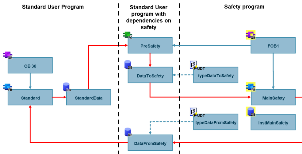
Figure 3-9 Reading standard data which can change during runtime of the safety program
