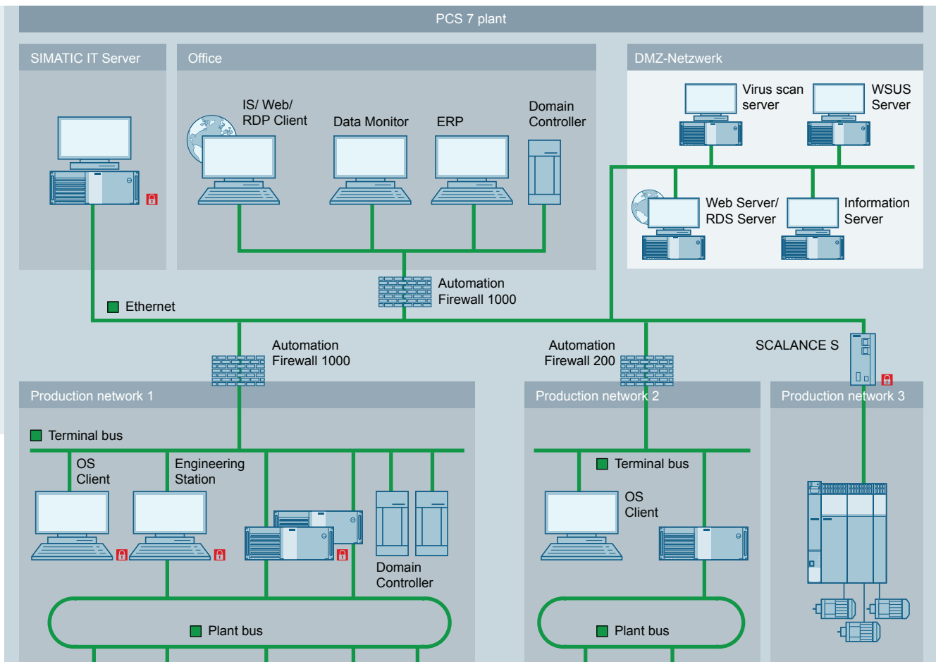
PCS 7 Security – Example of staggered security architecture
