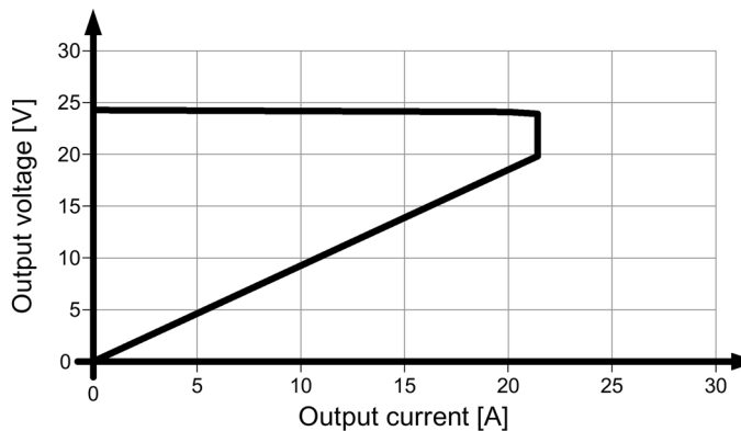
Figure 6-11 6EP1336-3BA10 latching shutdown output characteristic
