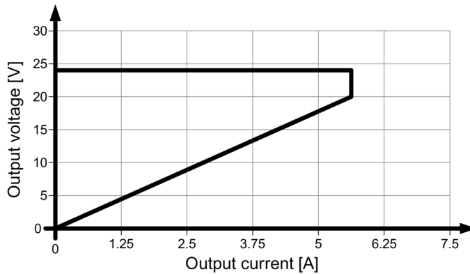
Figure 6-9 Output characteristic curve 6EP3333-8SB00-0AY0 latching shutdown
