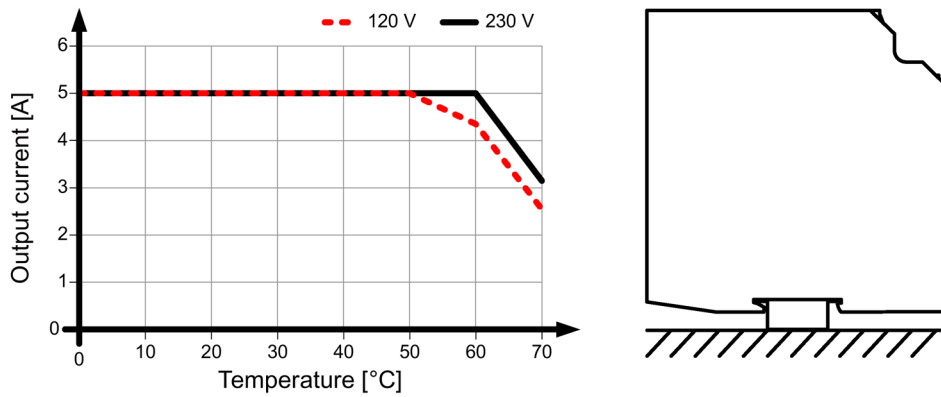
Figure 4-8 6EP3333-8SB00-0AY0 mounting position (4)
