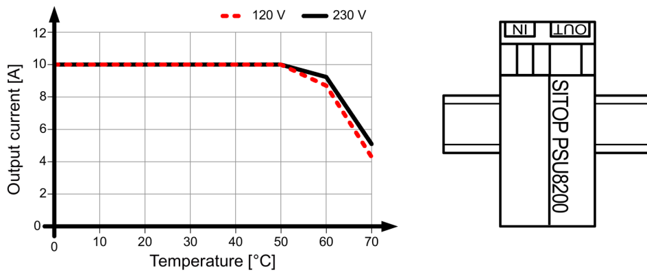
Figure 4-12 6EP3334-8SB00-0AY0 mounting position (3)
