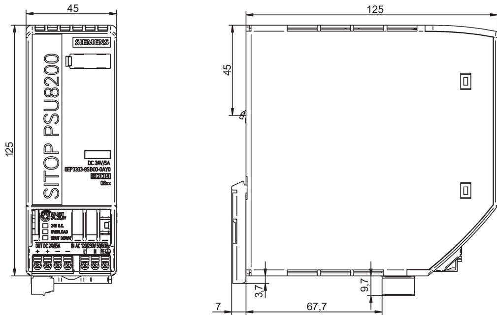
Figure 2-12 Dimension drawing 6EP3333-8SB00-0AY0
