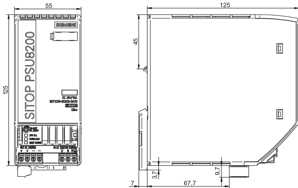
Figure 2-13 Dimension drawing 6EP3334-8SB00-0AY0
