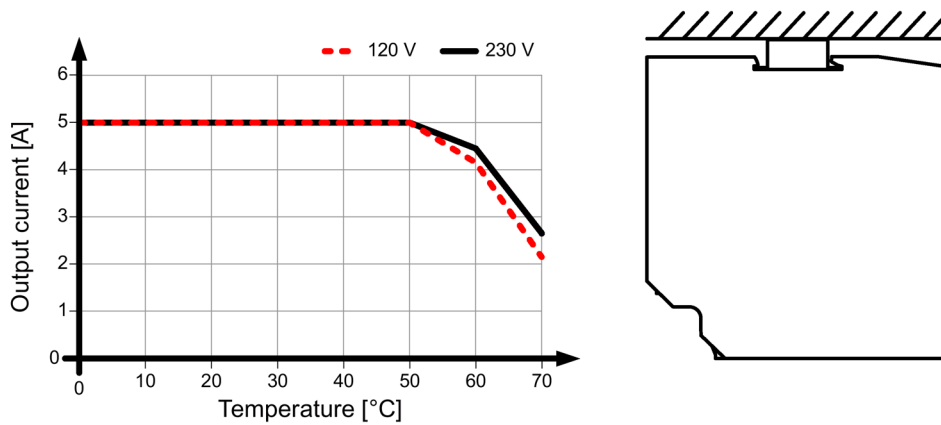
Figure 4-9 6EP3333-8SB00-0AY0 mounting position (5)
