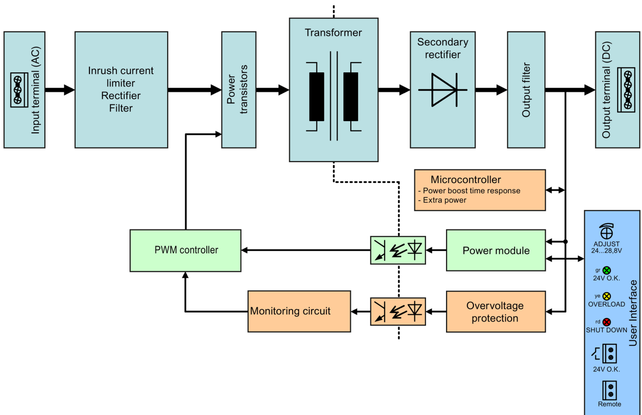
Figure 2-10 Block diagram for 6EP3333-8SB00-0AY0 and 6EP3334-8SB00-0AY0
