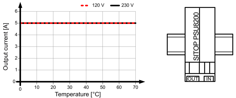
Figure 4-1 6EP3333-8SB00-0AY0 standard mounting position
