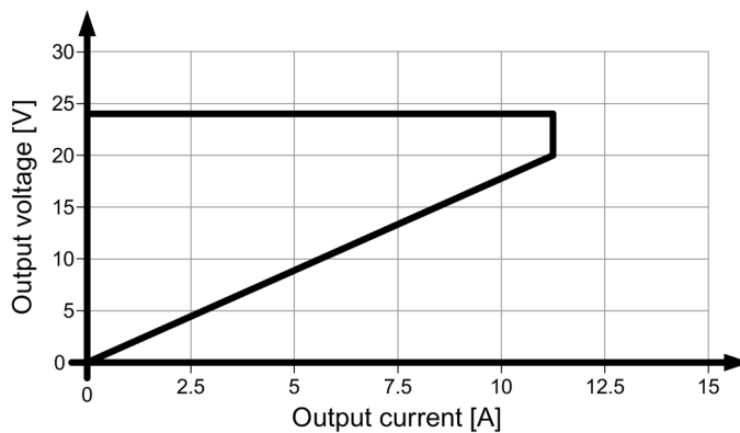
Figure 6-10 Output characteristic curve 6EP3334-8SB00-0AY0 latching shutdown
