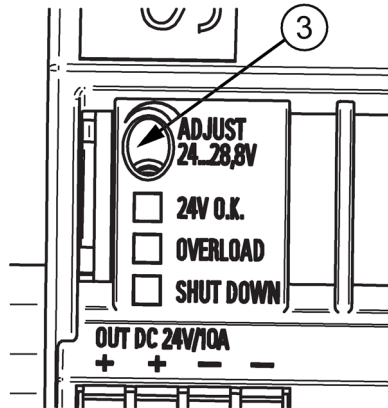
Figure 2-5 Potentiometer (example: 6EP3334-8SB00-0AY0)
