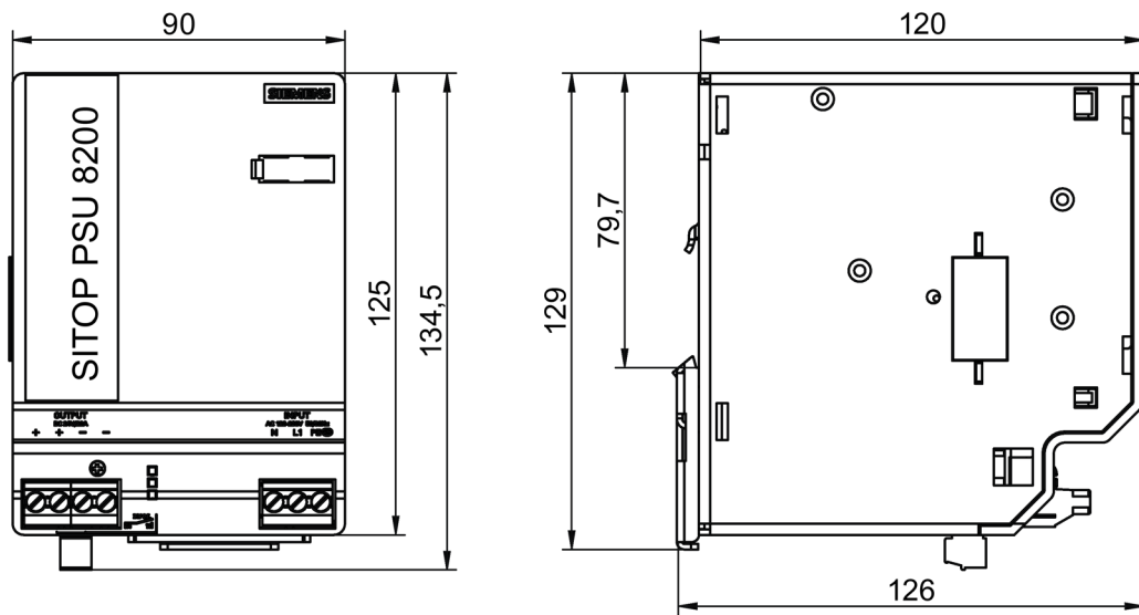
Figure 2-14 Dimension drawing for 6EP1336-3BA10
