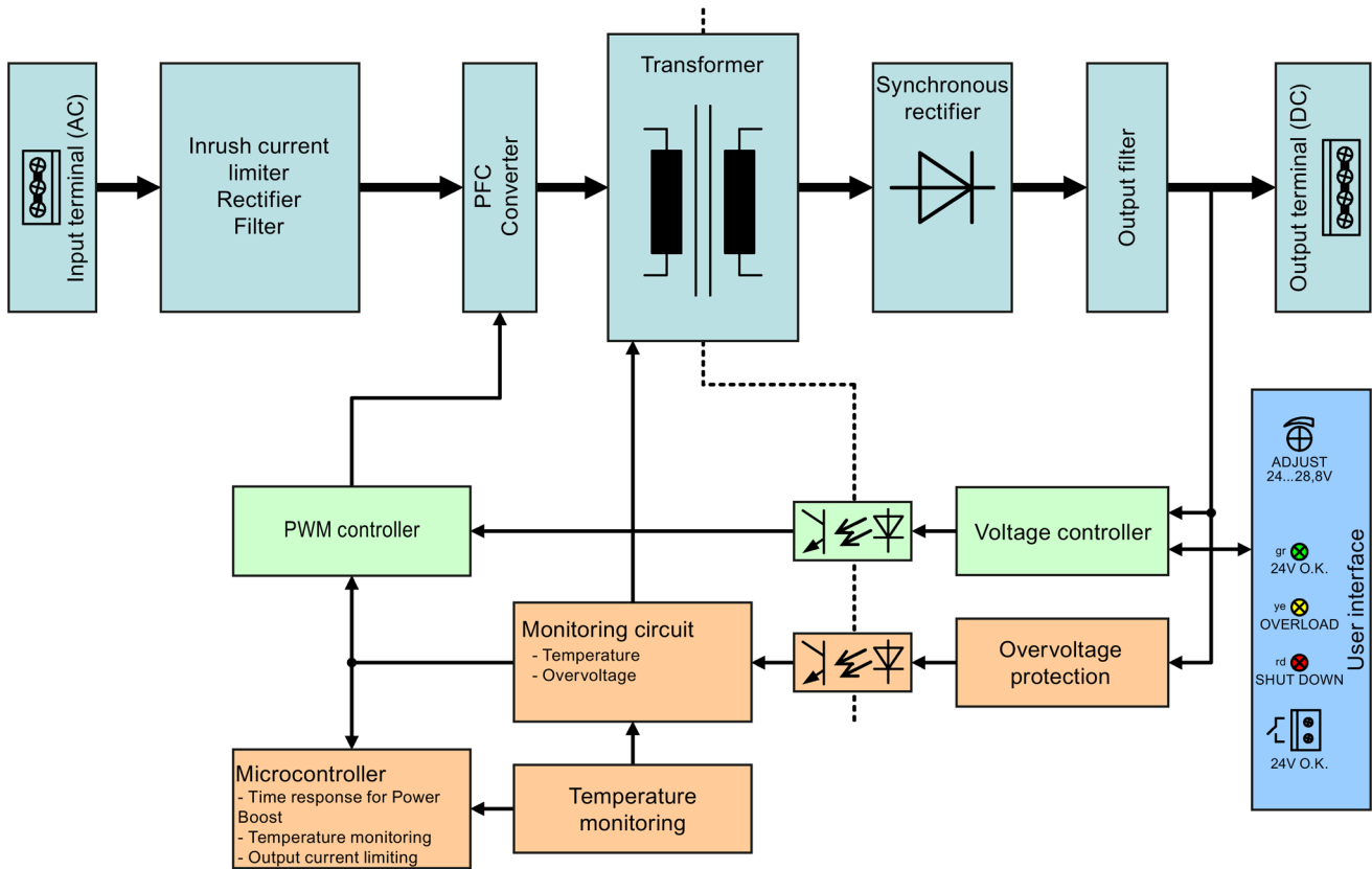
Figure 2-11 Block diagram for 6EP1336-3BA10
