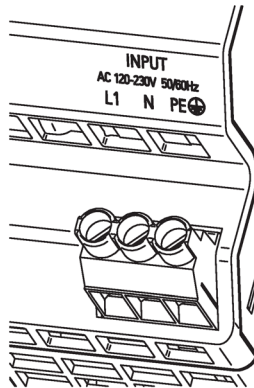
Figure 5-2 Line connection for 6EP1336-3BA10
