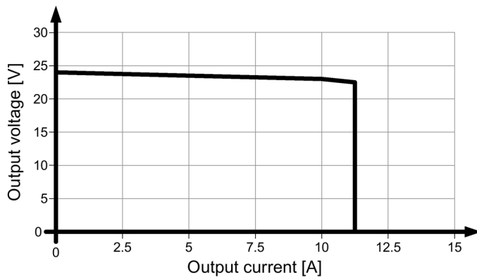
Figure 6-7 Output characteristic curve 6EP3334-8SB00-0AY0 parallel operation
