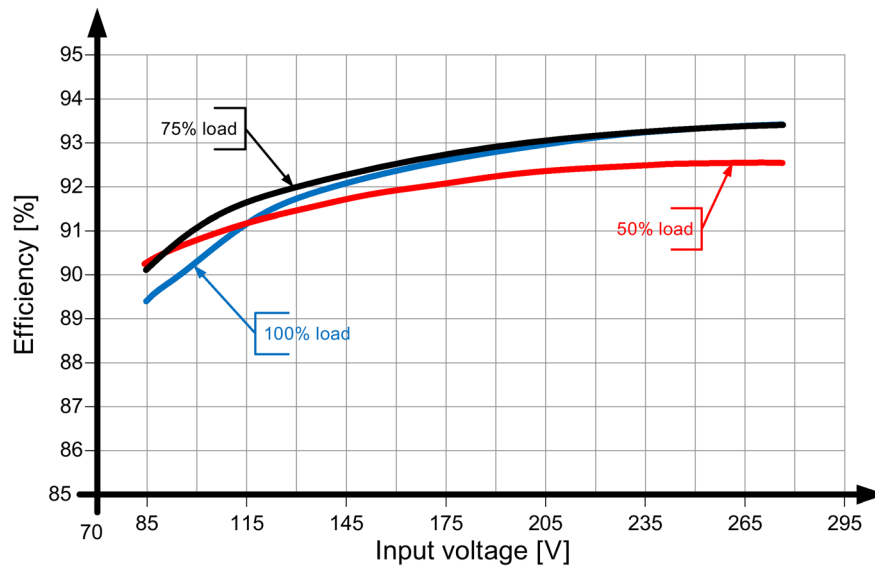
Figure 6-14 Efficiency 6EP1336-3BA10
