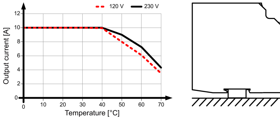
Figure 4-13 6EP3334-8SB00-0AY0 mounting position (4)
