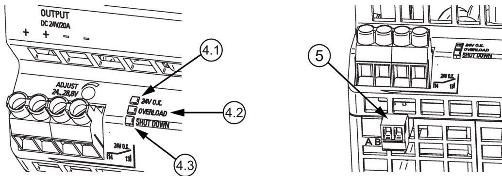
Figure 2-7 Operating display and signaling contact for 6EP1336-3BA10
