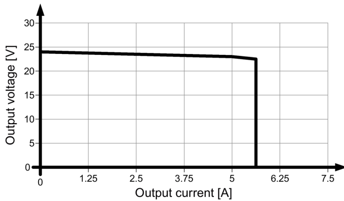
Figure 6-6 Output characteristic curve 6EP3333-8SB00-0AY0 parallel operation
