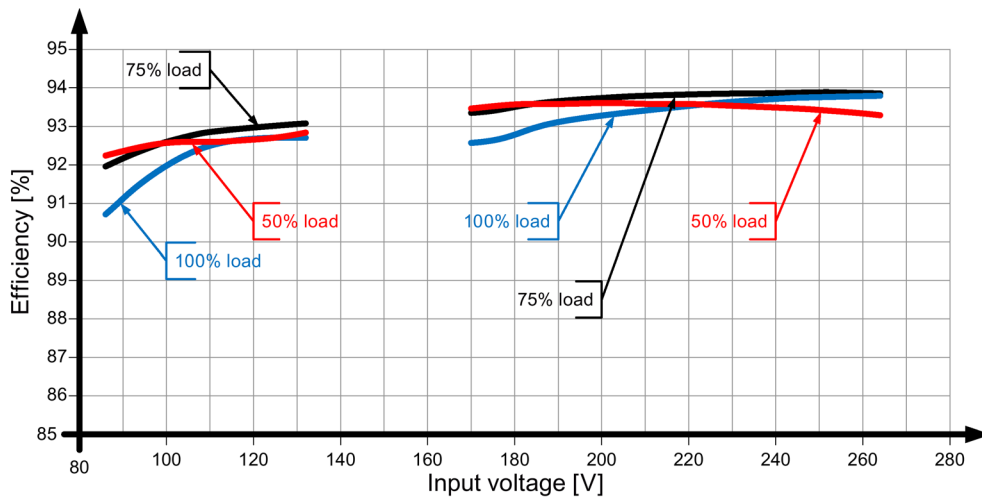
Figure 6-13 Power efficiency 6EP3334-8SB00-0AY0
