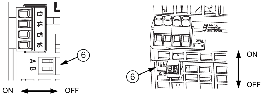
Figure 2-8 Selector switch
