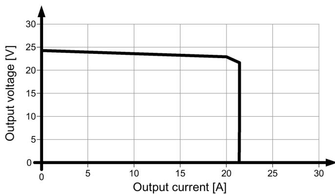
Figure 6-8 6EP1336-3BA10 parallel operation output characteristic
