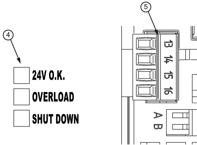
Figure 2-6 Operating display and signaling contact for 6EP3333-8SB00-0AY0 and 6EP3334-8SB00-0AY0
