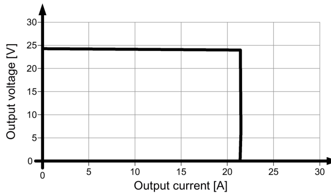
Figure 6-5 6EP1336-3BA10 single operation output characteristic
