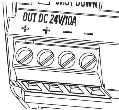
Figure 5-3 Output connection (example: 6EP3334-8SB00-0AY0)
