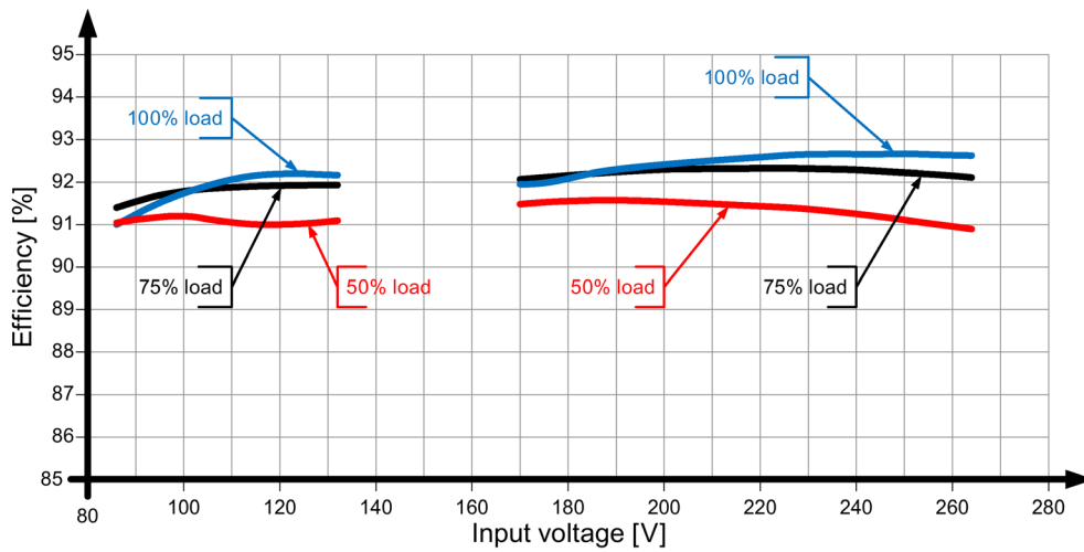
Figure 6-12 Power efficiency 6EP3333-8SB00-0AY0
