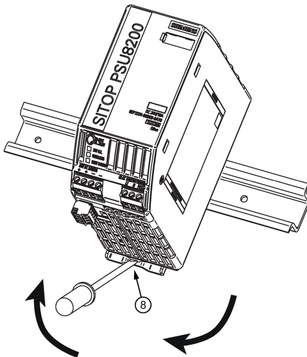
Figure 3-1 Mounting/removal (example): 6EP3334-8SB00-0AY0)
