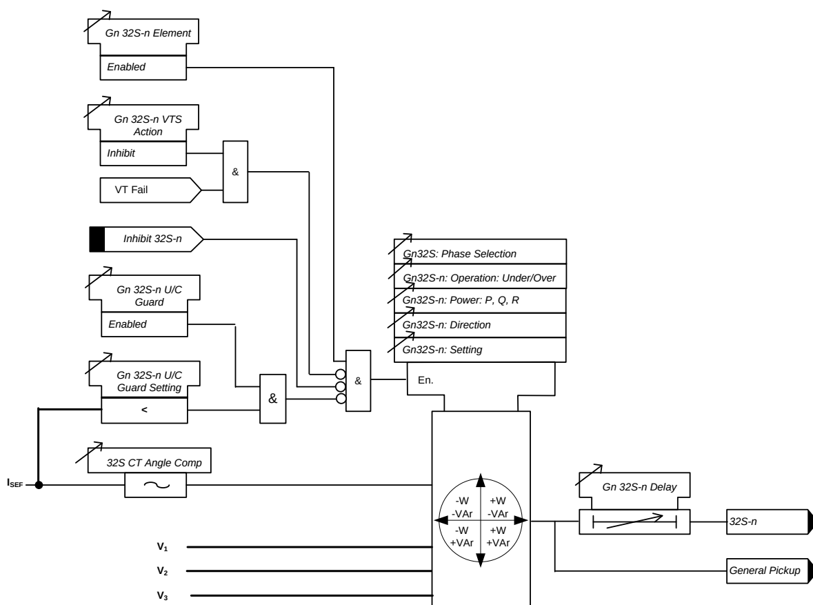
Figure 3-32 Logic Diagram: Sensitive Power Protection (32S)
