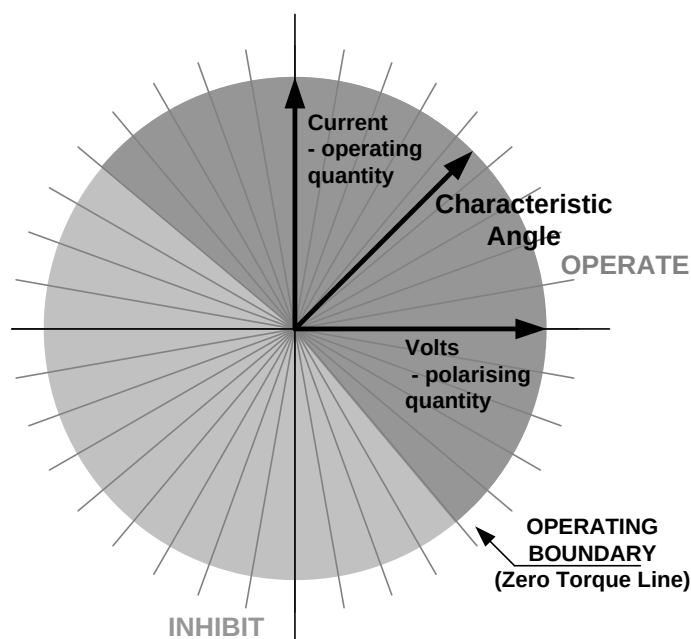
Figure 2.7-1 Directional Characteristics
