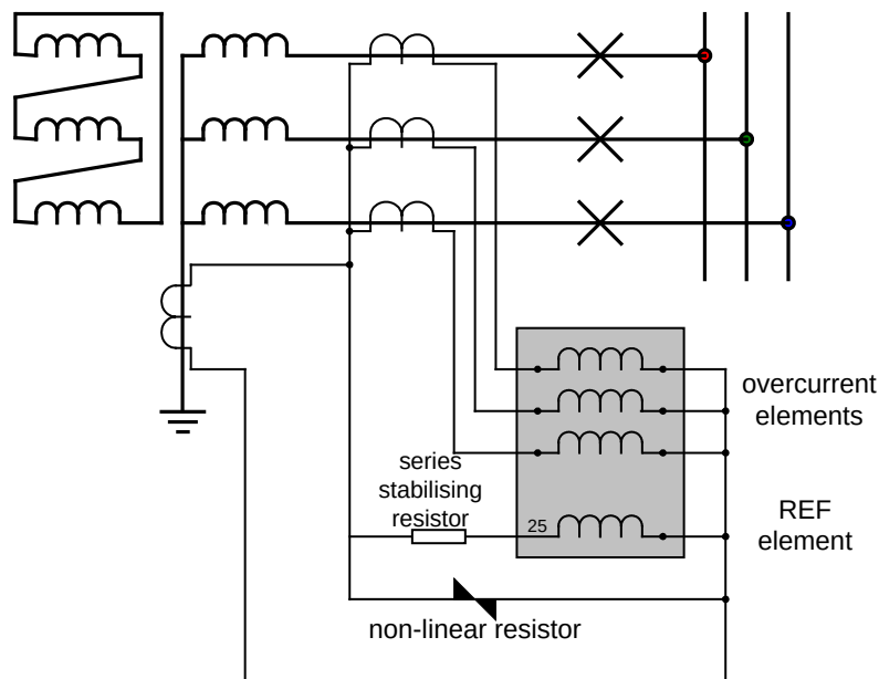
Figure 2.9-2 Composite Overcurrent and Restricted Earth-fault Protection
