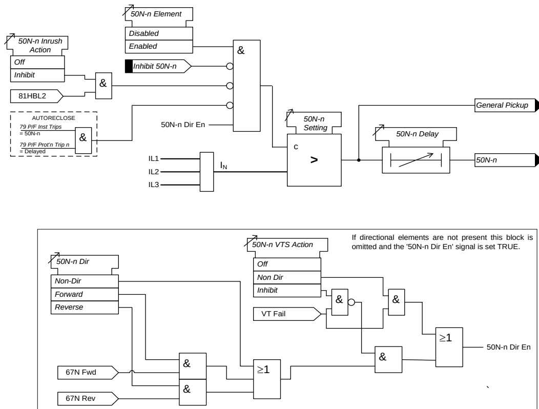
Figure 3-6 Logic Diagram: Derived Instantaneous Earth Fault Element
