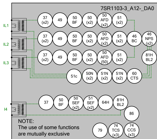
Figure 1-4 Functional Diagram of 7SR1103-3_A12-_DA0 Relay
