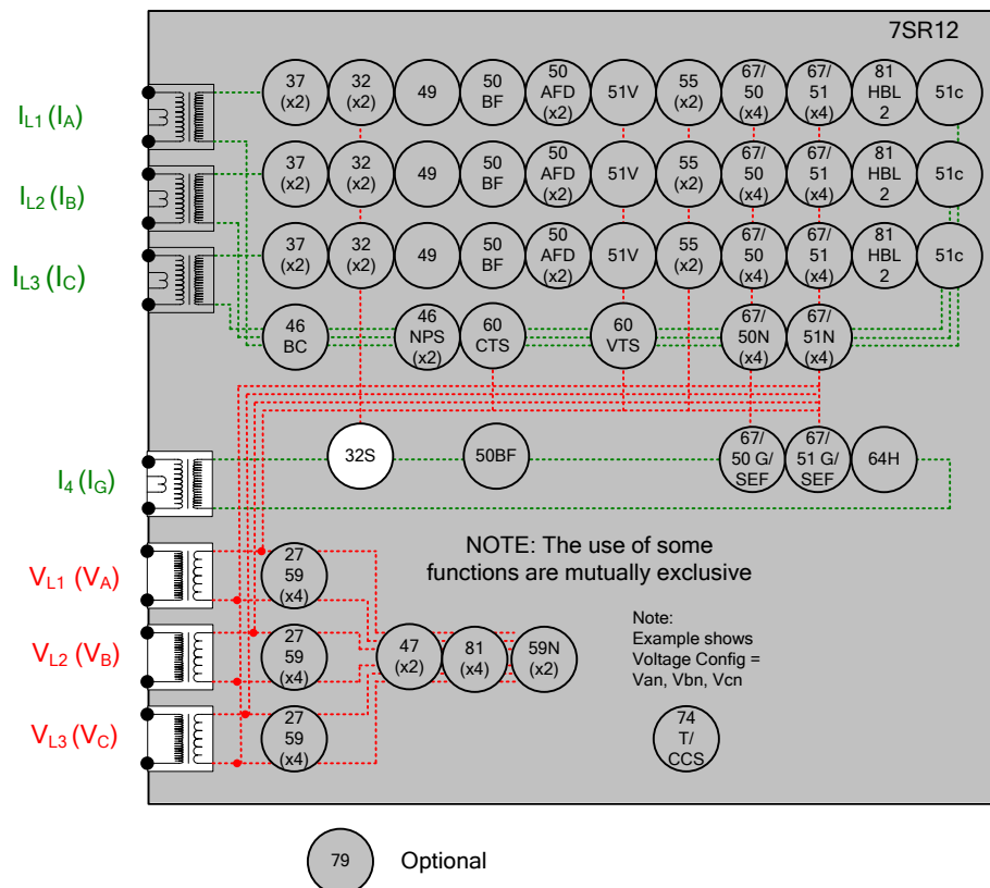
Figure 2-20 Sensitive Power
