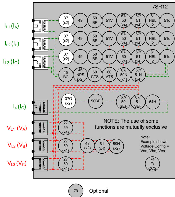
Figure 2-13 Undercurrent
