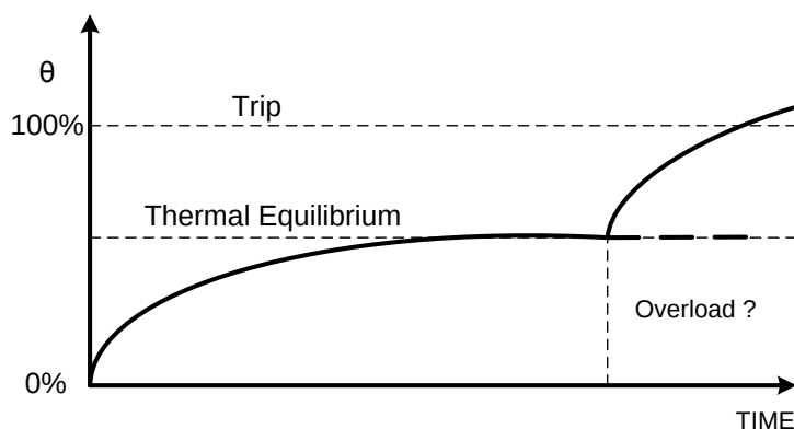
Figure 2.12-1 Thermal Overload Heating and Cooling Characteristic
