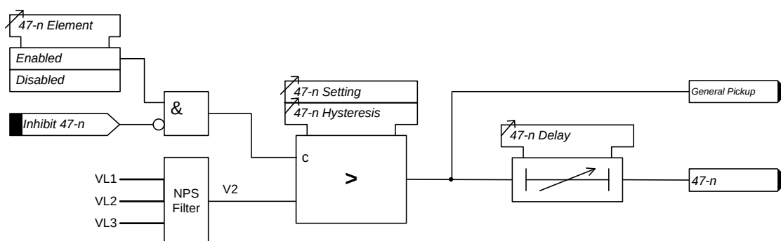
Figure 3-28 Logic Diagram: NPS Overvoltage Protection (47)
