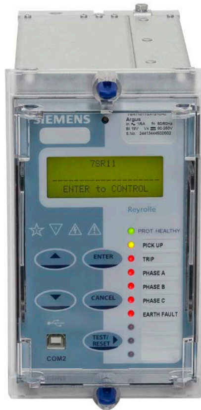
Figure 1.1-3 Fascia of a 7SR11 relay (E4 Case)
