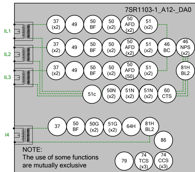
Figure 1-3 Functional Diagram of 7SR1103-1_A12-_DA0 Relay
