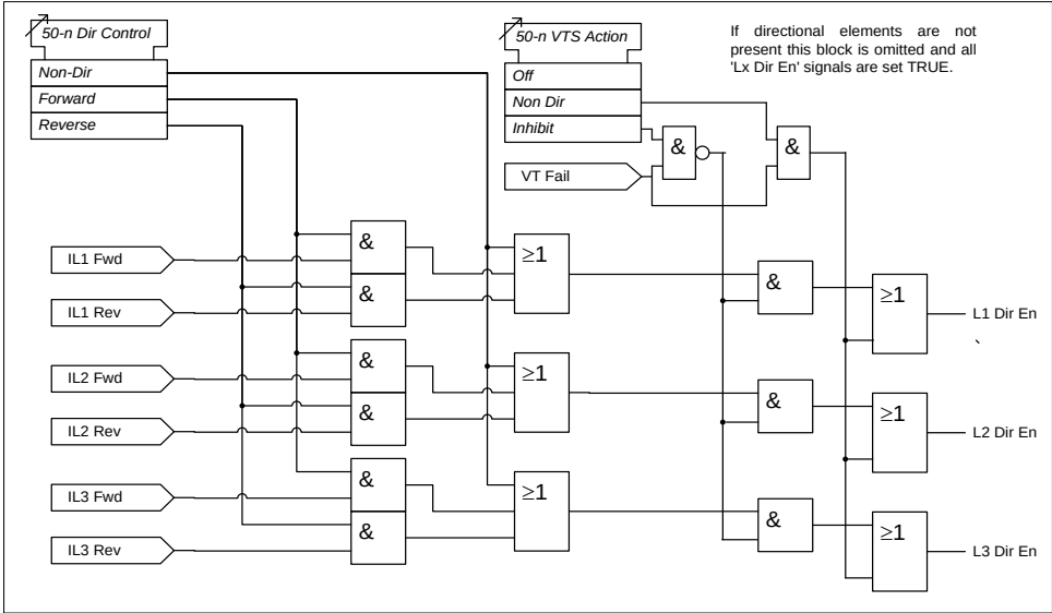
Figure 3-2 Logic Diagram: Instantaneous Over-current Element
