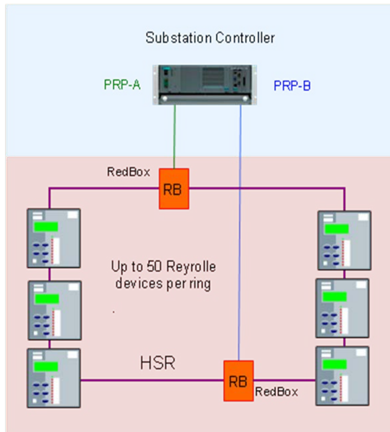
Figure: 6.3-3 HSR Ethernet Network Ring Configuration
