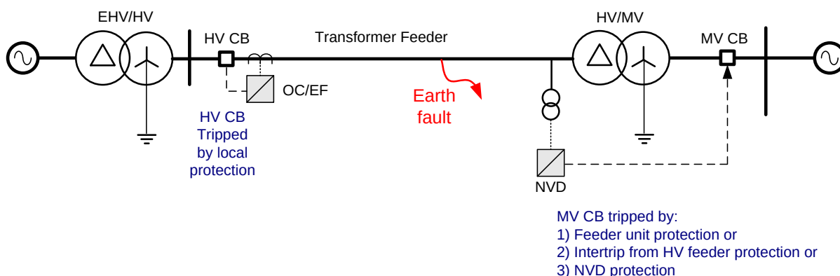
Figure 2.14-1 NVD Application
