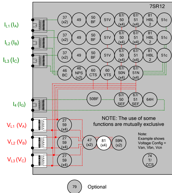
Figure 2-18 Under/Over Frequency
