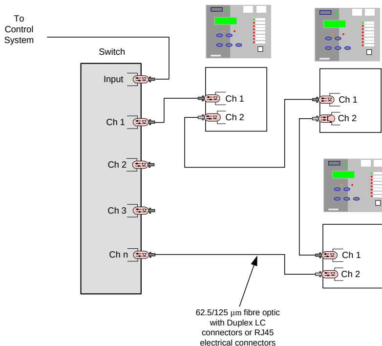
Figure: 6.2-2 Ethernet connection for IEC 61850 (ring connection)
