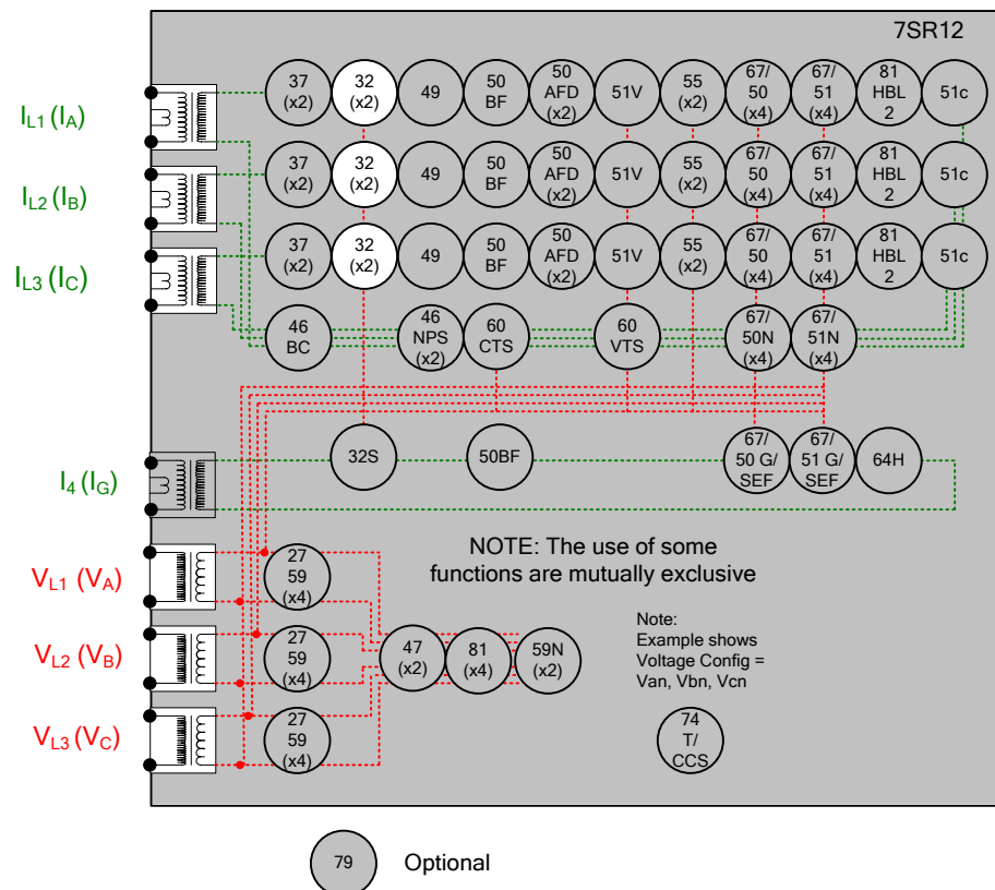
Figure 2-19 Power
