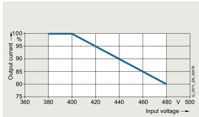
Permissible output current as a function of input voltage for 400 V SINAMICS G120X converters, frame sizes FSH and FSJ, at low overload (LO)
