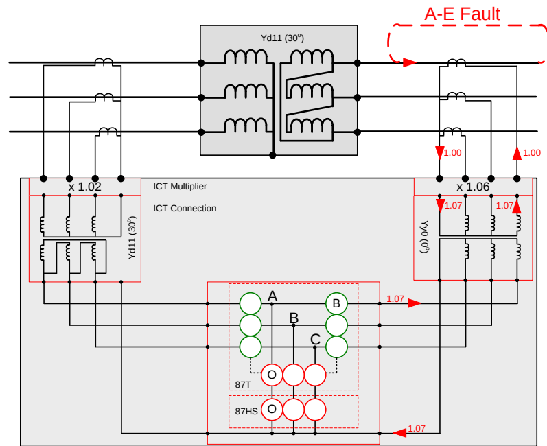
Figure 2-9: Relay Currents - Delta Winding Internal Earth Fault
