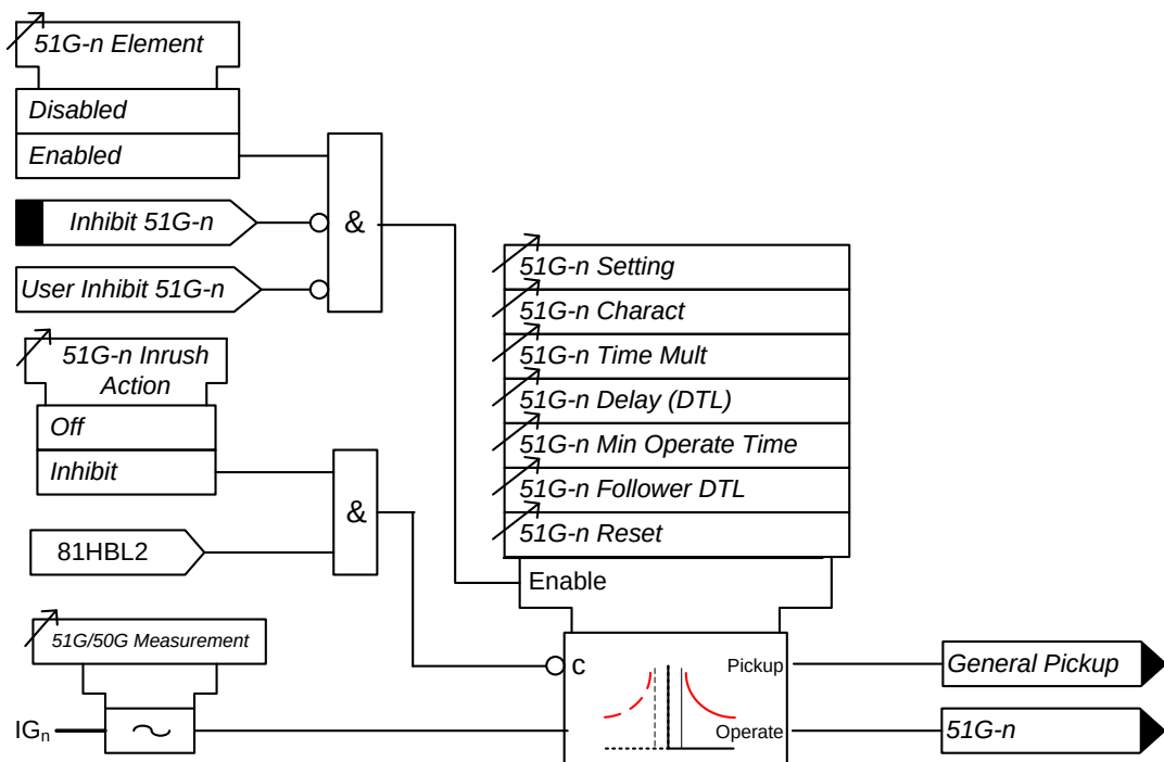
Figure 3-10 Logic Diagram: Time Delayed Measured Earth Fault Element (51G)
