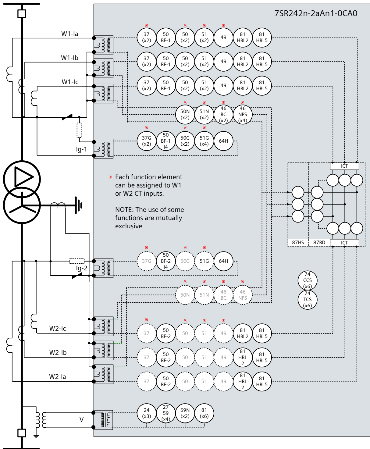
Figure 1-3 Function Diagram: 7SR242n-2aAnn-0CA0 Relay
