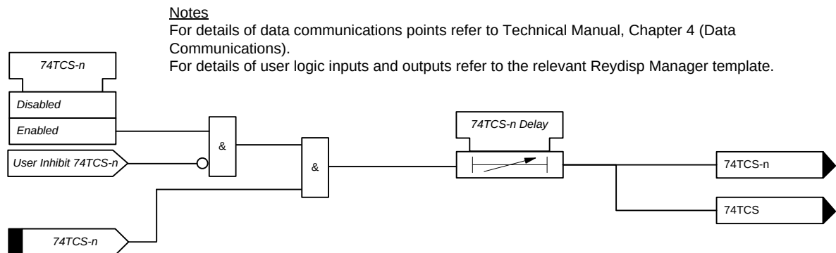
Figure 5-2 Logic Diagram: Trip Circuit Supervision Feature (74TCS)
