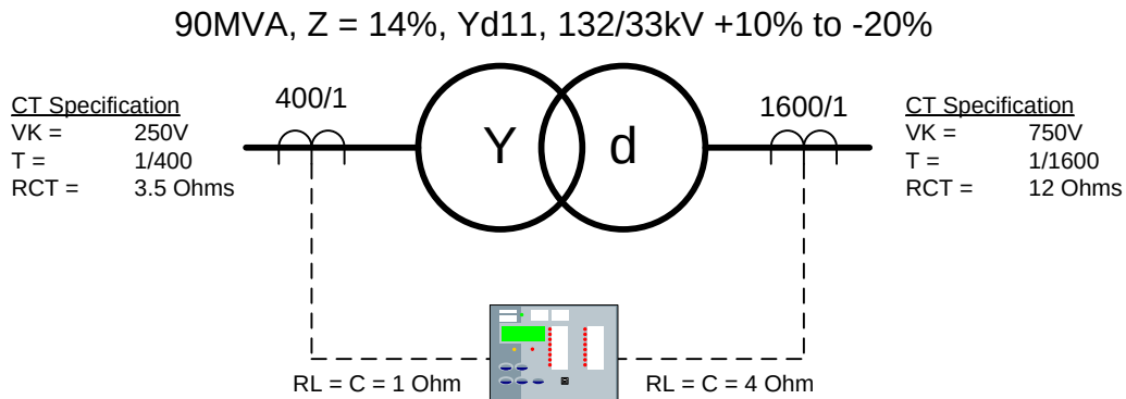
Figure 3-1 CT Requirements
