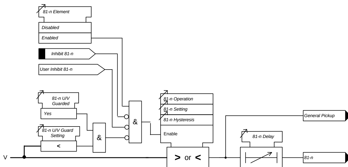
Figure 3-20 Logic Diagram: Under/Over Frequency Detector (81)
