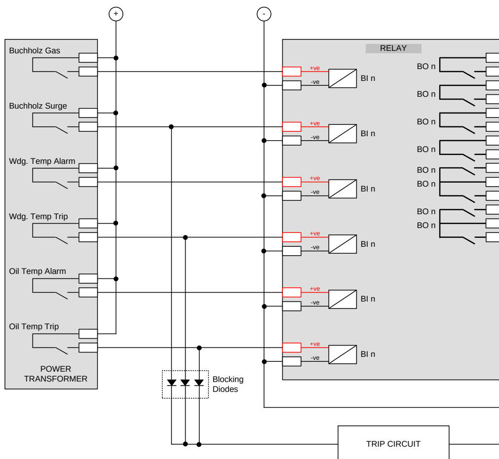
Figure 7-2 Example of Transformer Alarm and Trip Wiring
