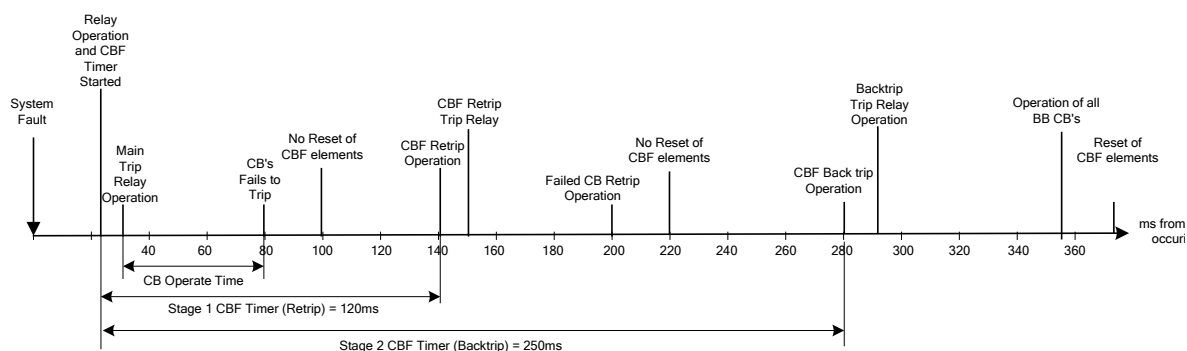
Figure 5-3 - Two Stage Circuit Breaker Fail Timing
