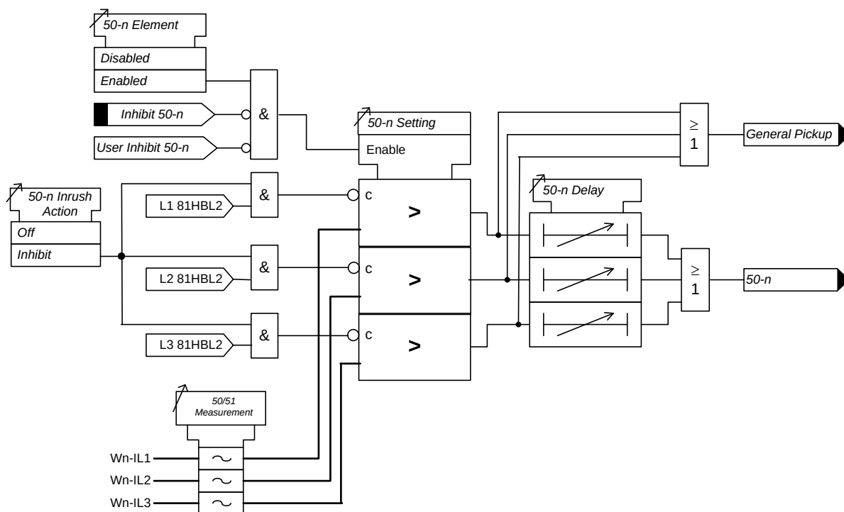
Figure 3-5 Logic Diagram: Instantaneous Over-current Element
