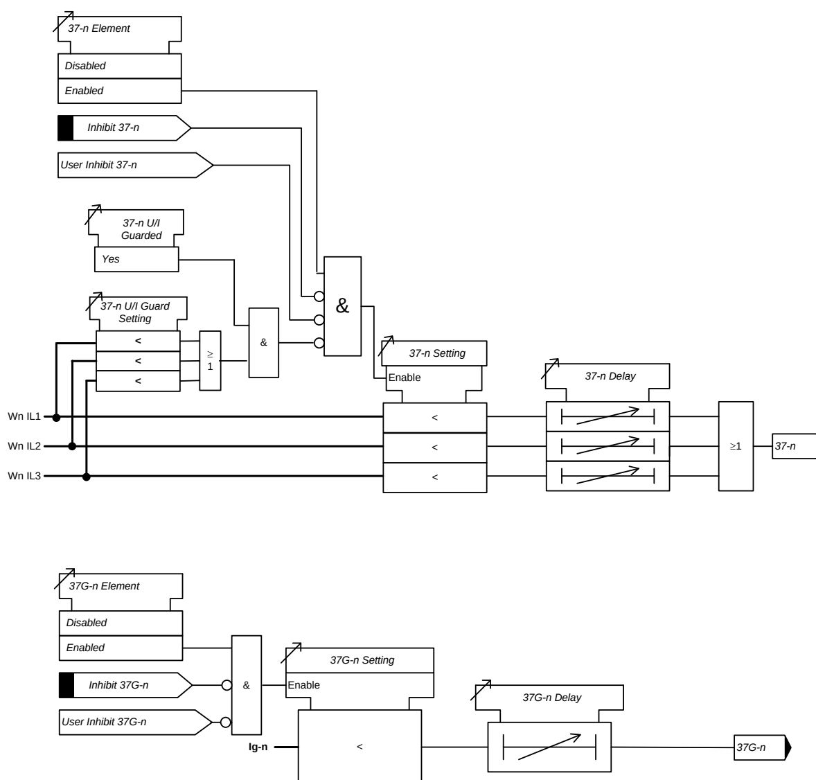
Figure 3-14 Logic Diagram: Undercurrent Detector (37, 37G)
