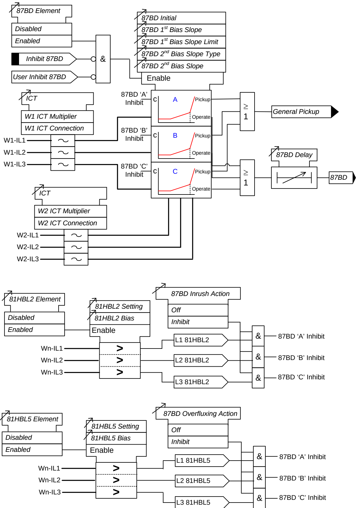
Figure 3-2 Functional Diagram for Biased Current Differential Protection
