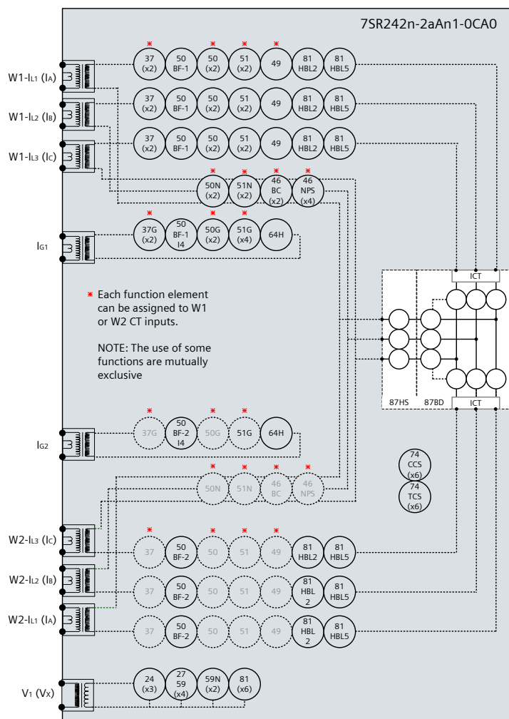
Figure 2-1 Biased Differential
