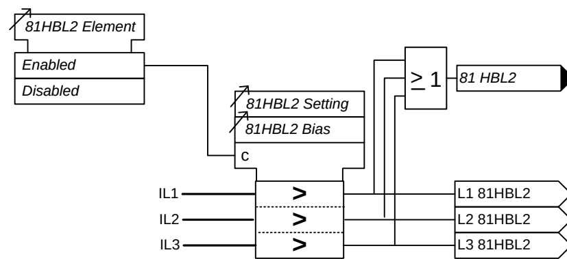
Figure 5-4 Logic Diagram: Inrush Detector Feature (81HBL2)
