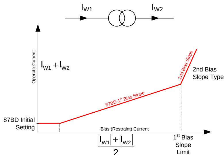
Figure 2-2: 87BD Characteristic
