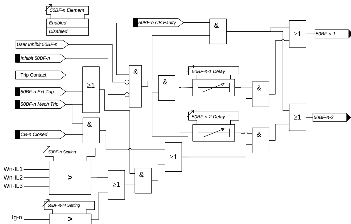
Figure 5-1 Logic Diagram: Circuit Breaker Fail Protection (50BF)
