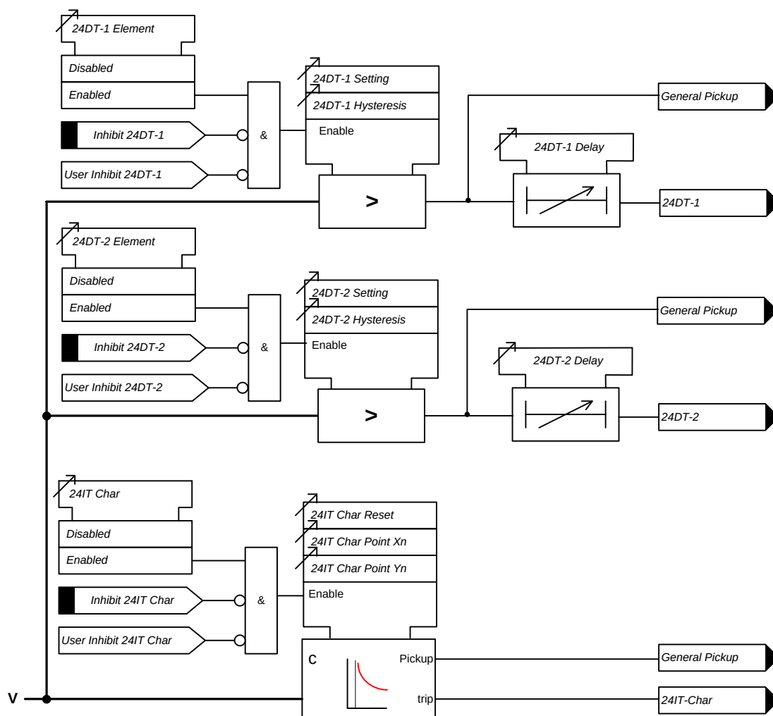
Figure 3-17 Logic Diagram: Overfluxing Elements (24)
