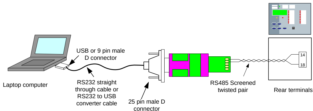
Figure 2-2 RS485 connection to PC
