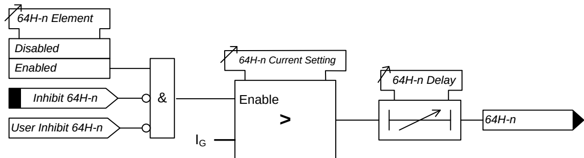
Figure 3-11 Logic Diagram: High Impedance REF (64H)
