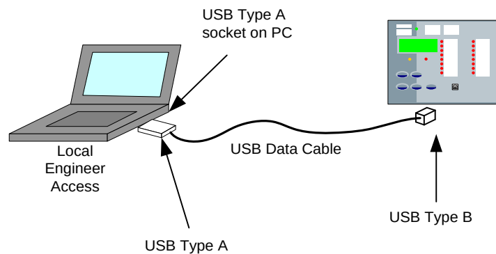
Figure 2-1 USB connection to PC
