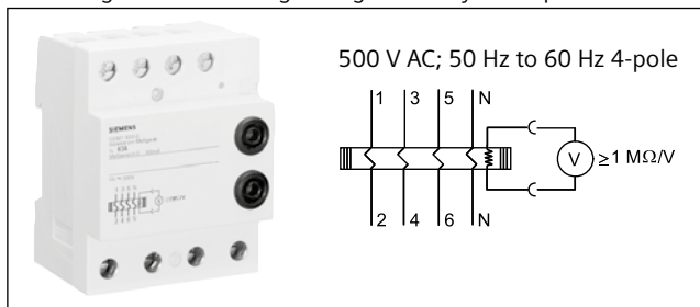
Figure 26: 5SM1 930-0 leakage current measurement device
