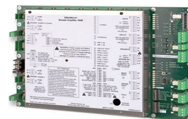
Model EBA2004-A1 Main Board
