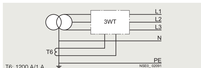
3-pole circuit breakers, current transformers in the grounded neutral point of the transformer
