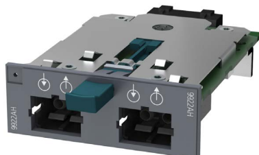
图 4-31 MM991-2P (SC RJ) [9912AH]
