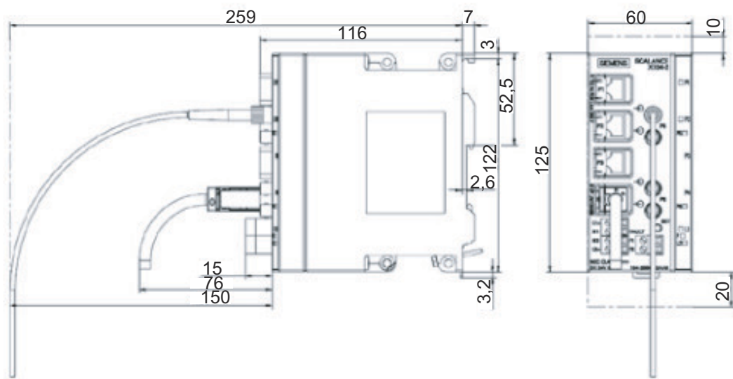
Figure A-4 Side view SCALANCE X-200
