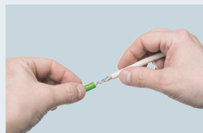
Remove the outer sheath and expose the braided shield
