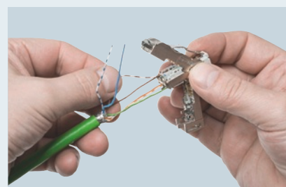
Insert the wires into the plug according to color code and pull them out the opposite side
