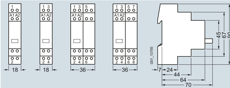
5TT4101 5TT4102 5TT4103 5TT4104 5TT4105 5TT4115
