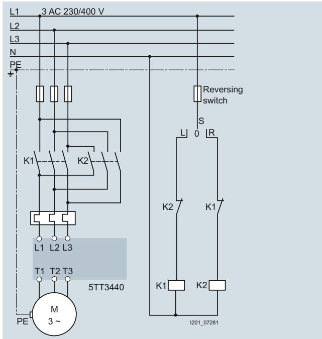
Typical circuit for 5TT3440
