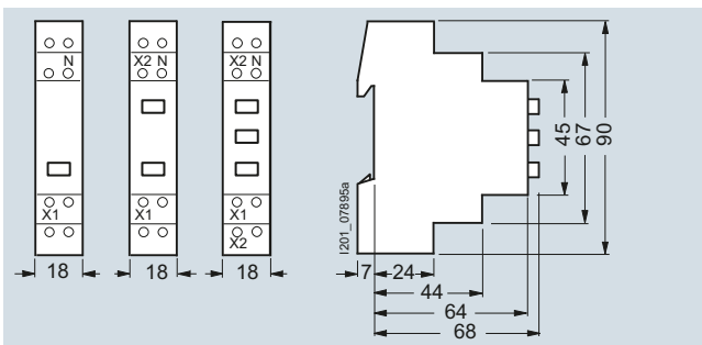
5TE5800 5TE5801 5TE5802 5TE5804 5TE5803
