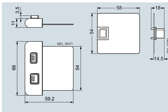
7LF4941-0 USB adapter
