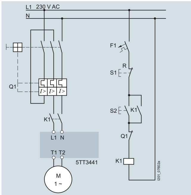
Typical circuit for 5TT3441
