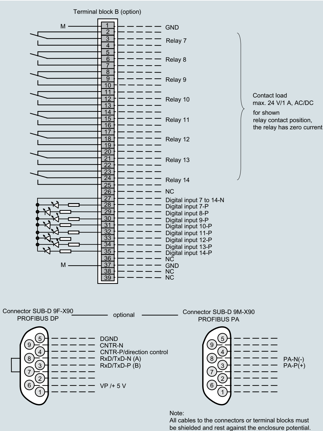
ULTRAMAT 6, field device, pin and terminal assignment of the AUTOCAL board and PROFIBUS connectors
