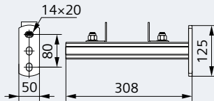
LR ... -BHW1
