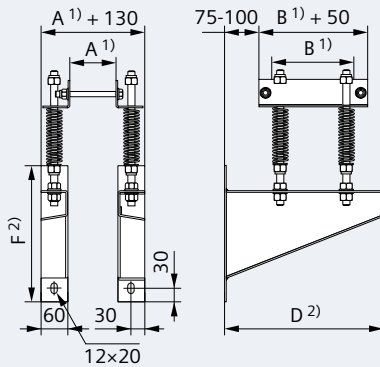
LR ... -BVW
