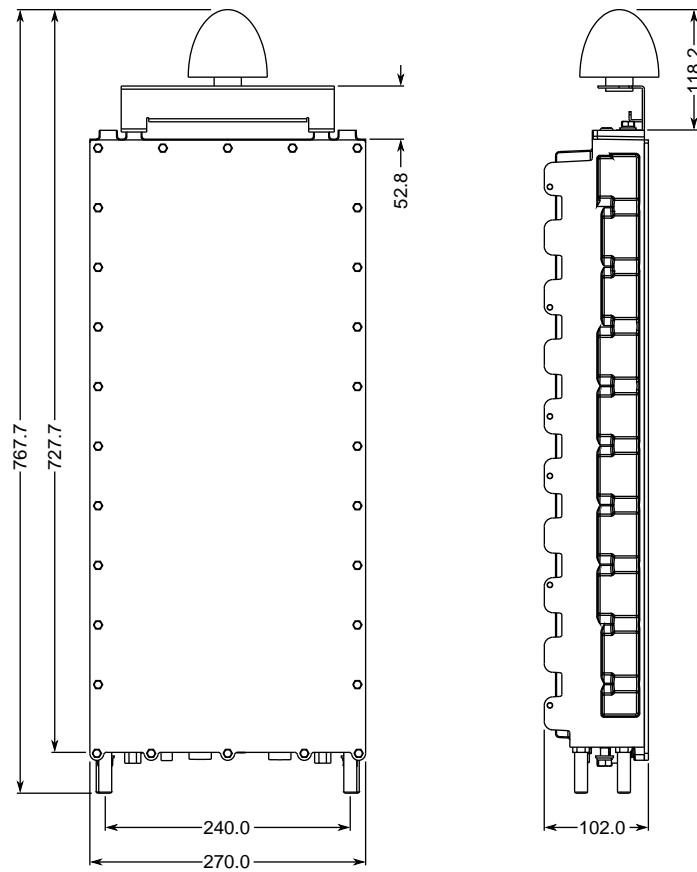
Figure 20: RUGGEDCOM WIN7025 Dimensions without Mounting Bracket
