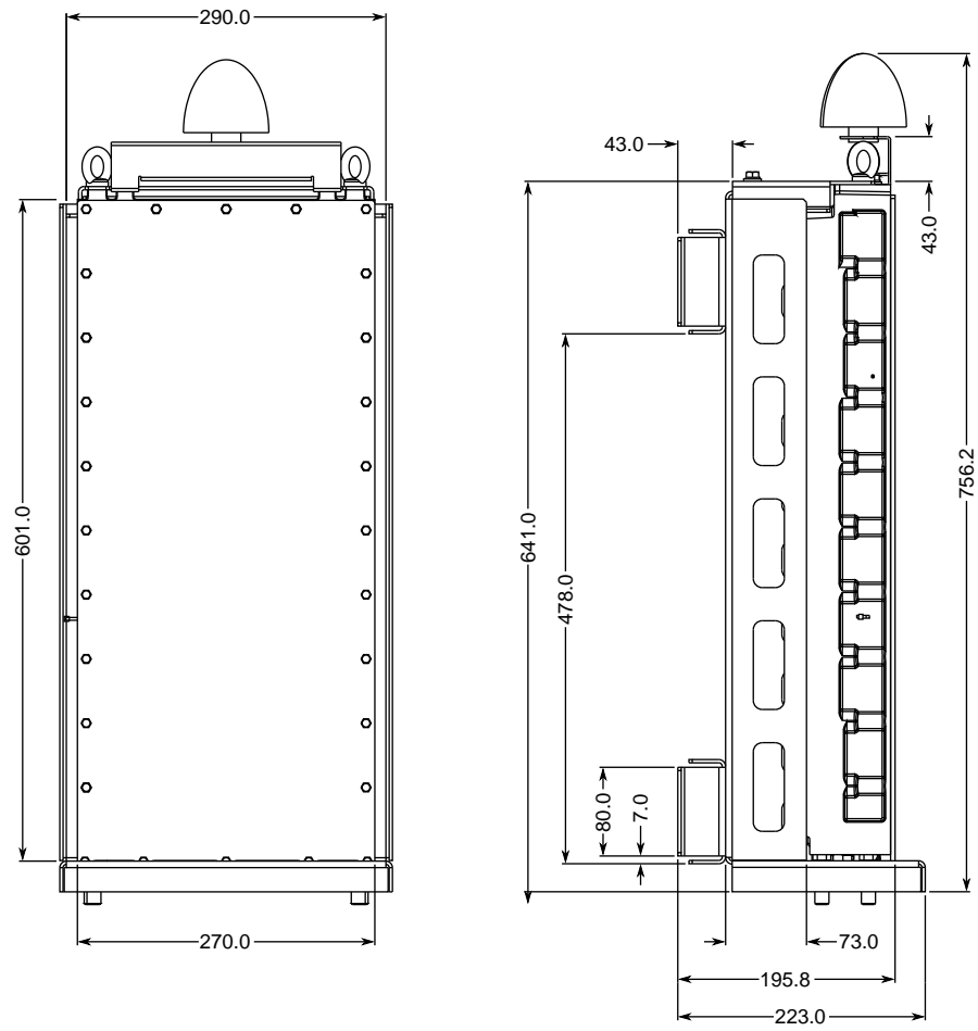
Figure 21: RUGGEDCOM WIN7025 Dimensions with Mounting Bracket
