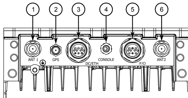
Figure 2: RUGGEDCOM WIN7025 Communication Ports for SFA and SFD Models
