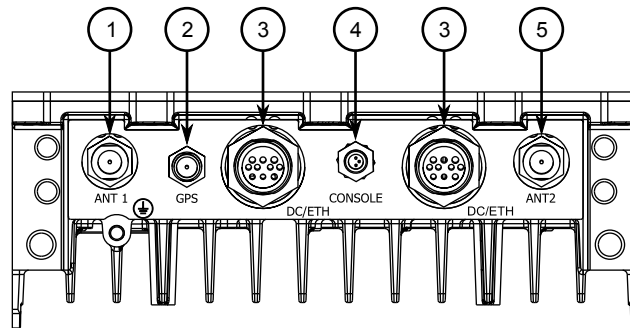
Figure 1: RUGGEDCOM WIN7025 Communication Ports for PEC Model
