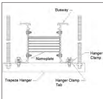
Flat Mounted
