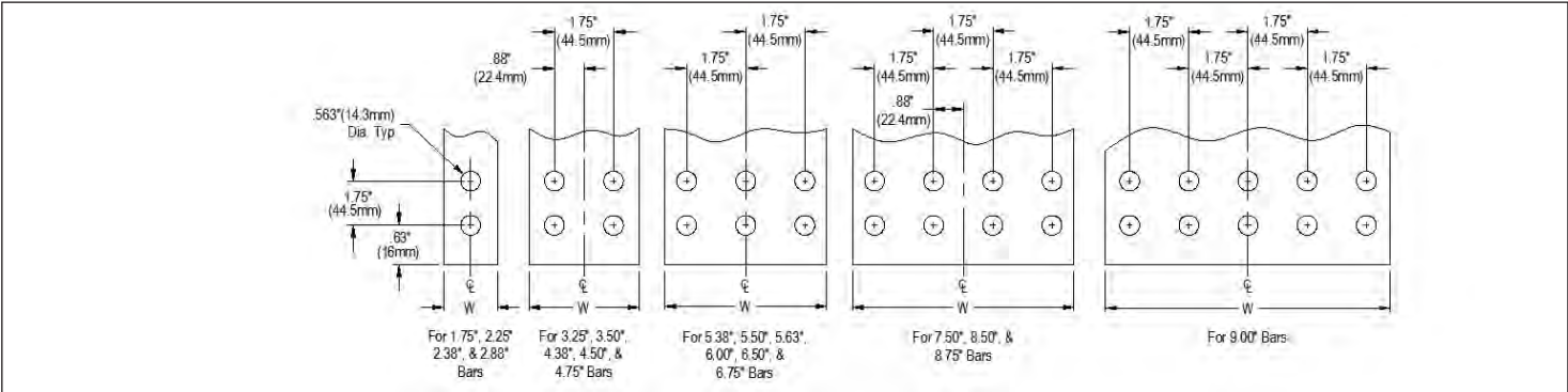
Flanged End Bus Bar Drilling Pattern (NEMA) ① (Same pattern for 2 bus bars per pole, see figure 2 above.)
