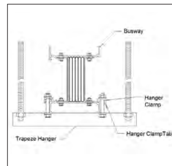
Edge Mounted
