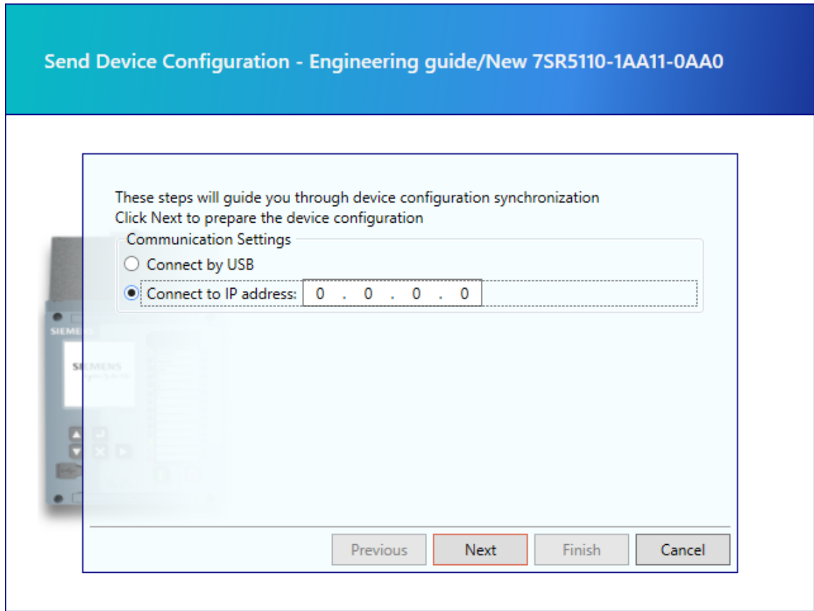
[sc_7SR5_ReydispManager2ConnectionOptions, 1, --,--]
