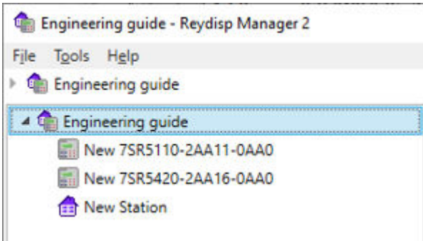
[sc_7SR5_ReydispManager2NewStationProjectTree, 1, --]
