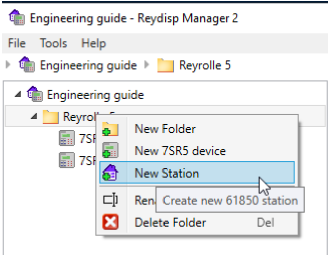
[sc_7SR5_ReydispManager2NewStation, 1, --]
