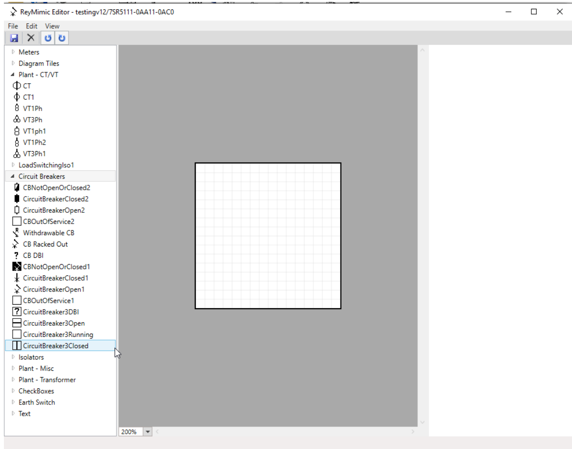
[sc_7SR5_ReydispManager2ReymimicDisplayEditor, 1, --]
