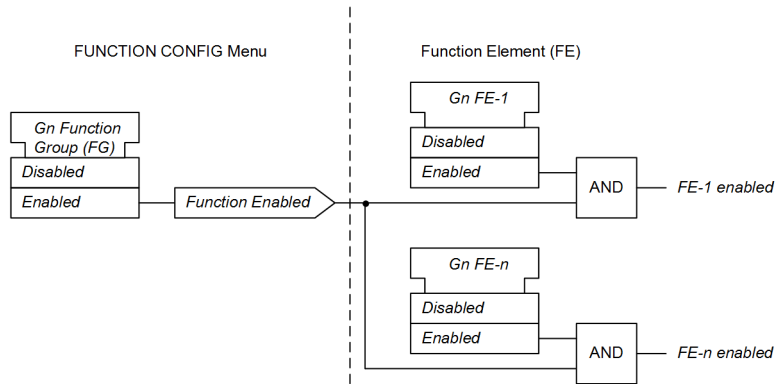
Figure 2-81 Reydisp Manager 2 Function Configuration Logic Diagram
