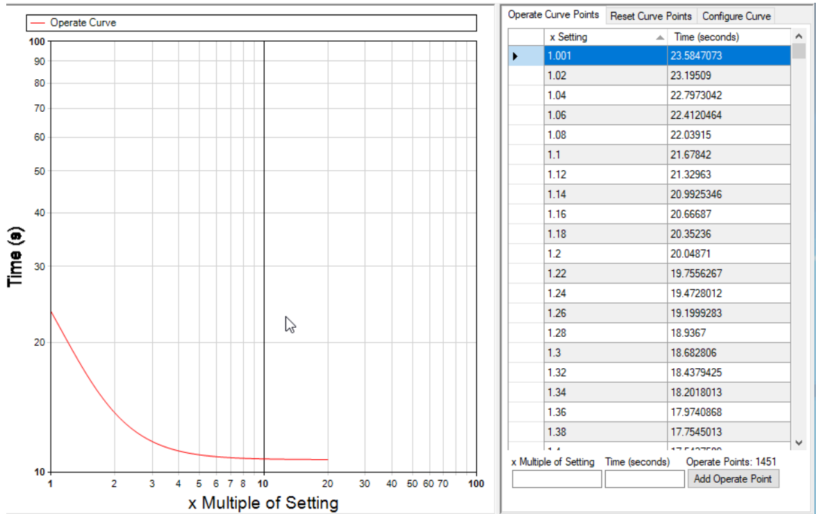
Figure 2-75 Reydisp Manager 2 Operate Curve Points
