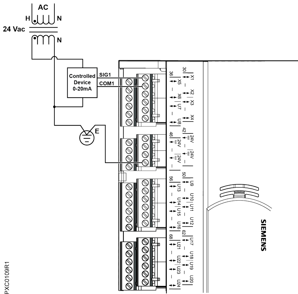
Connecting an Analog Output (0 to 20 mA) (PXC-36).
