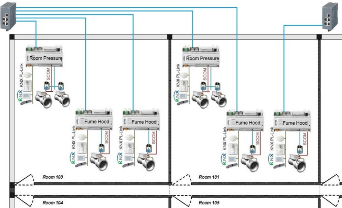
Fig. 86: Lab DXR2 network - Star
