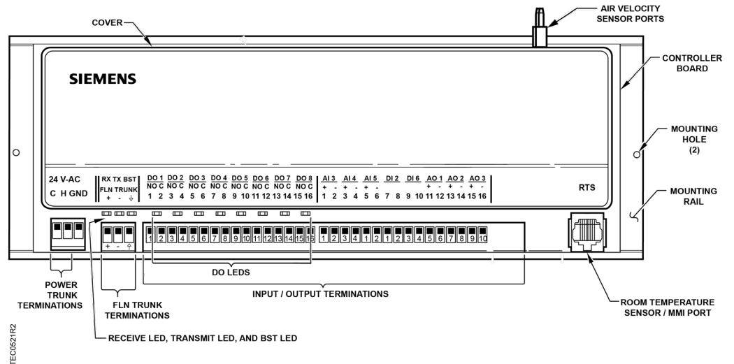
Fig. 179: 8 DO Controller with Air Velocity Sensor.
