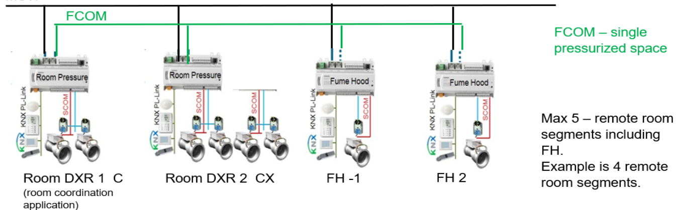
Fig. 74: Lab MSTP – Combination Multi-room and Fume Hoods
