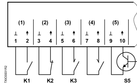
Dry Contacts; Supervised, Digital Input Module.
