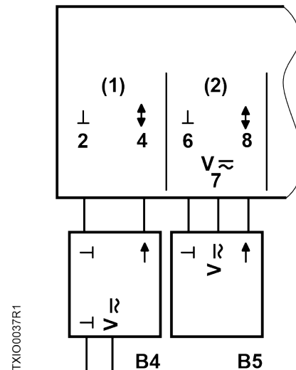
0-10 Vdc Input (Voltage); Supervised, Universal and Super Universal Modules.
