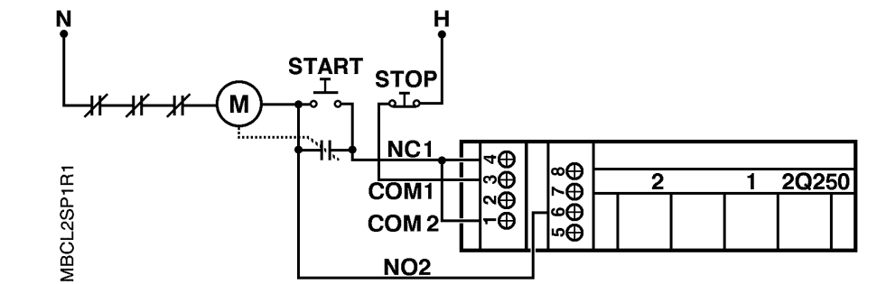
Fig. 149: Connecting an L2SP (No Proof).
