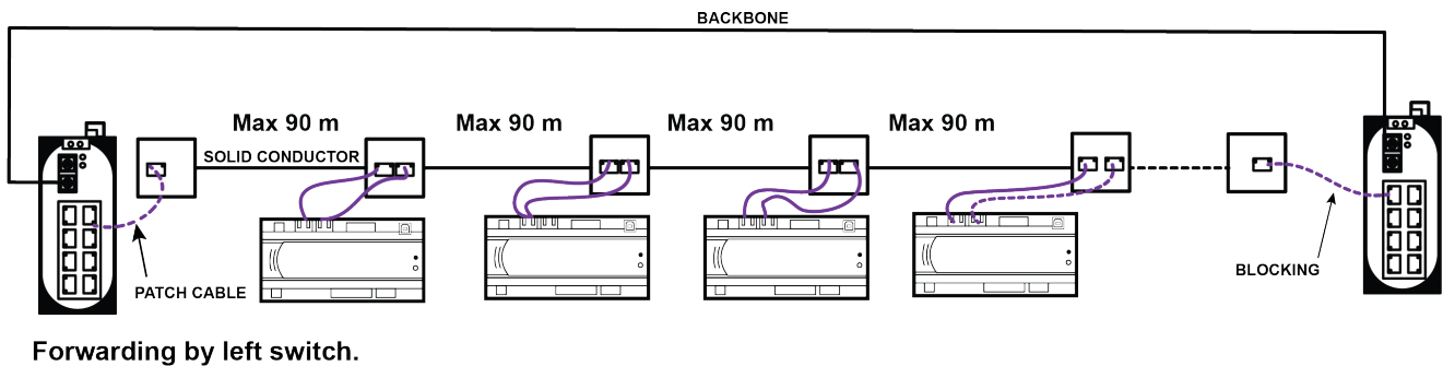
Fig. 5: Wiring Diagram one Line of up to 8 Dual Port Ethernet Controllers within a STP Loop Configuration (fault tolerant).
