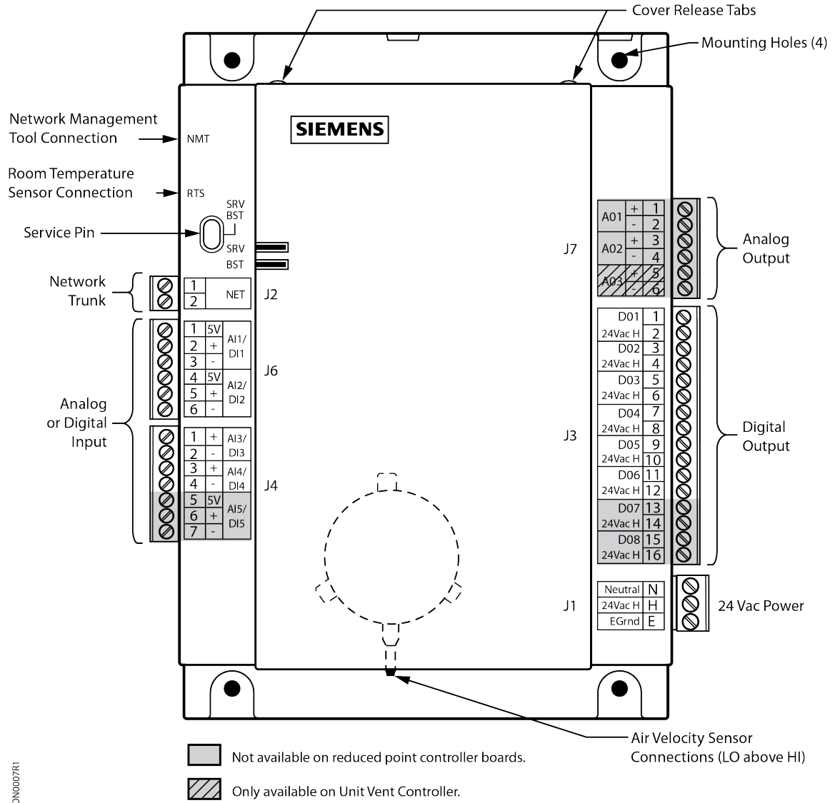
Fig. 159: LTEC Wiring Designations.
