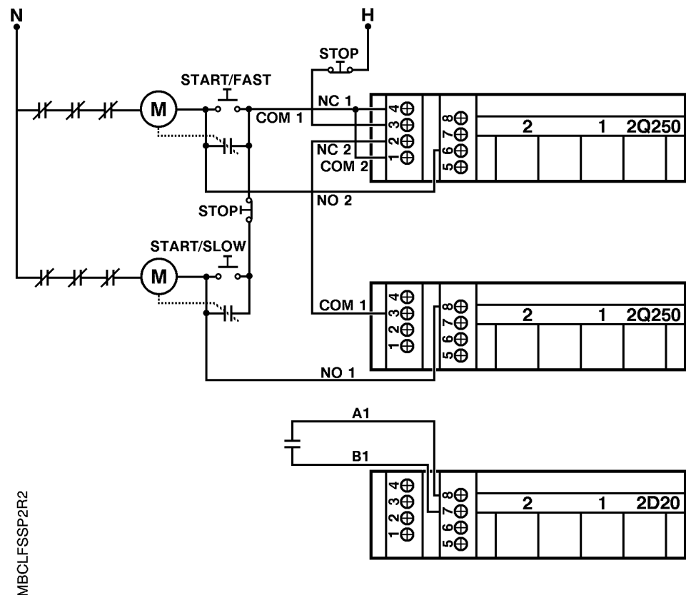
Fig. 138: Connecting an LFSSP (Proof of Contact).
