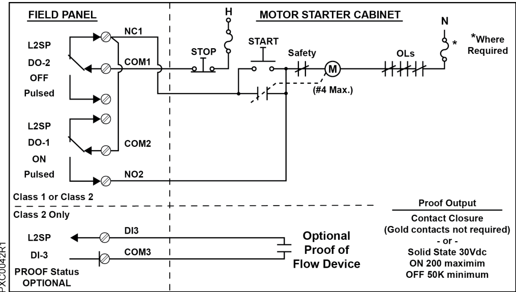
Fig. 48: Connecting an L2SP (Proof Optional).
