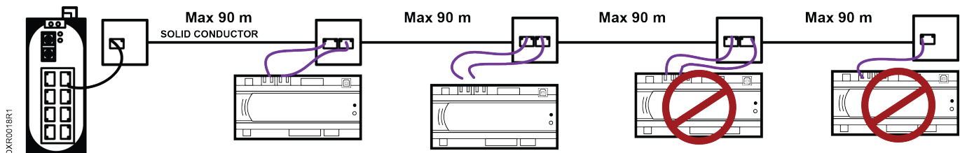
Fig. 6: Wiring Diagram one Line of Dual Port Ethernet Controllers (not fault tolerant downstream will lose connectivity).
