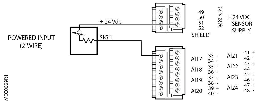
Fig. 105: Connecting a 2-Wire Analog Input (4 to 20 mA).
