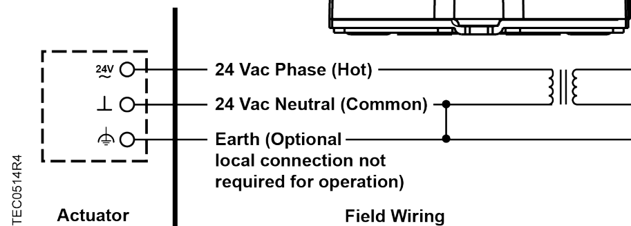
Fig. 93: Power Trunk Connection to ATEC.
