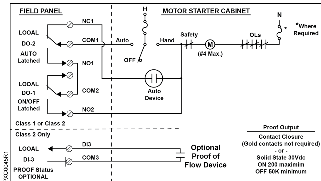
Fig. 45: Connecting an LOOAL (Proof Optional).
