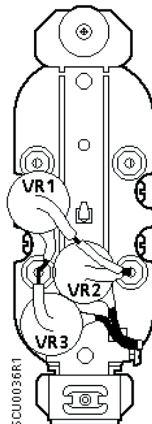
Fig. 153: SCU Receptacle with MOVs.
