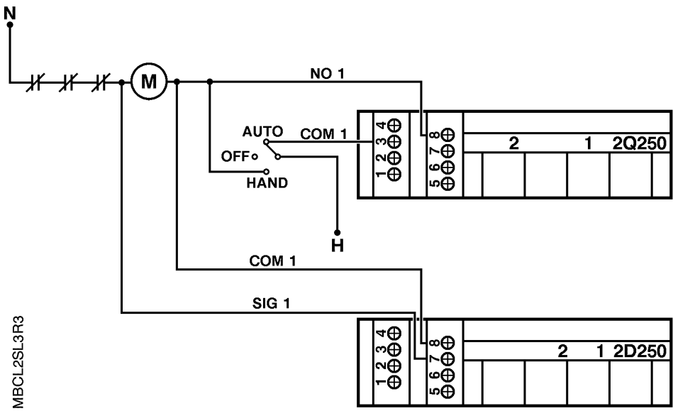
Fig. 148: Connecting an L2SL (Proof of Voltage).
