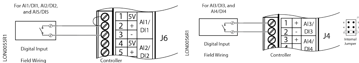
Digital Input Connection to LTEC Inputs AI 1/DI 1, AI 2/DI 2, or AI 5/DI 5. Digital Input Connection to LTEC Inputs AI 3/DI 3 or AI 4/DI 4.
