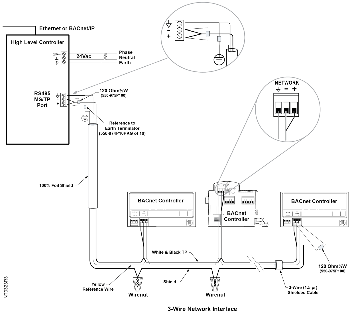
Fig. 15: 3-Wire (1.5 pair) Network Wiring Detail.
