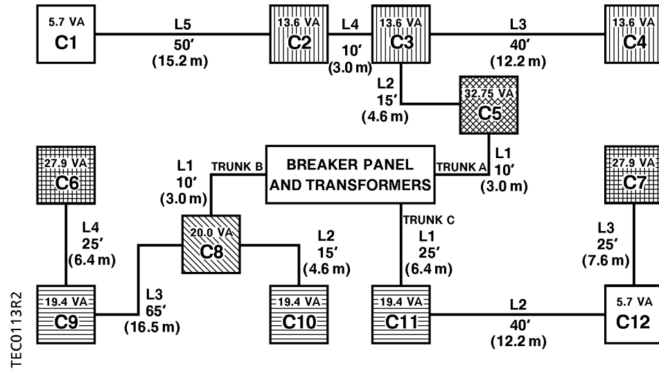
Fig. 42: Completed Example Layout.
