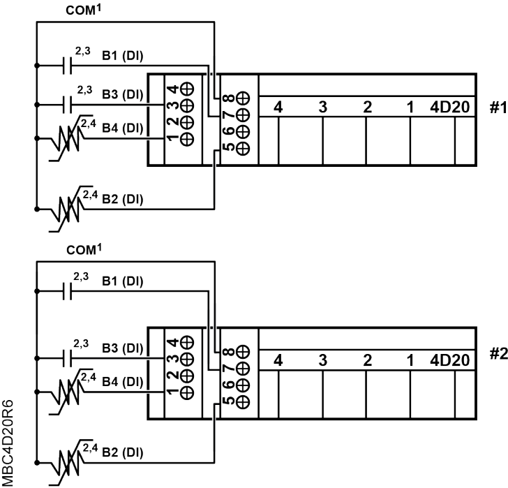
Fig. 130: Connecting a Digital Input (Dry Contacts).
