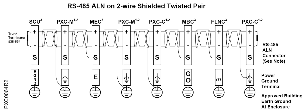
Fig. 22: RS-485 ALN Trunk Shield Connection.
