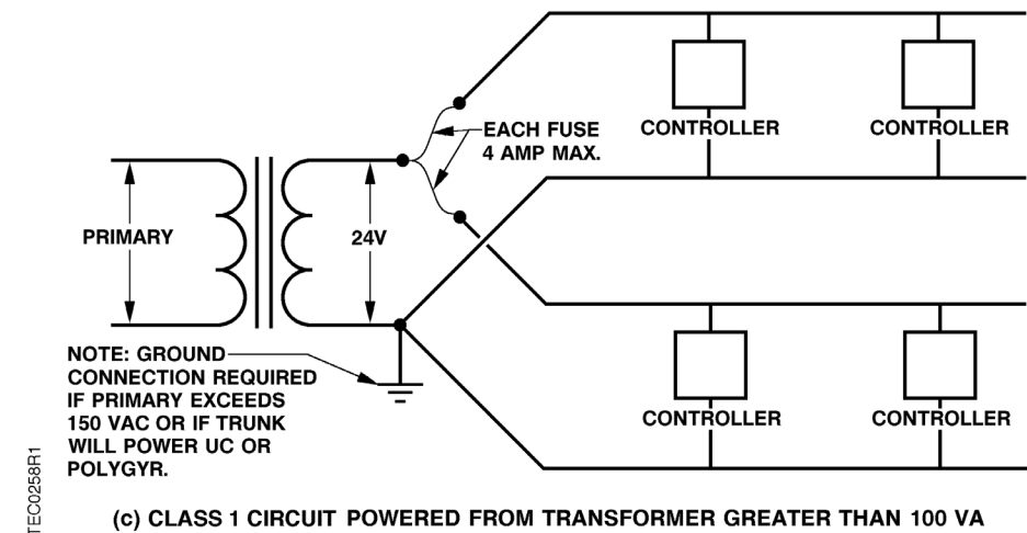
Fig. 39: Power Trunk Layout, Class 1 Circuit.
