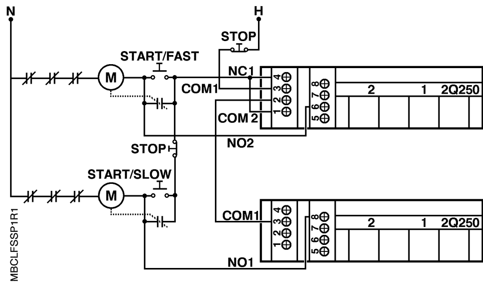
Fig. 137: Connecting an LFSSP (No Proof).
