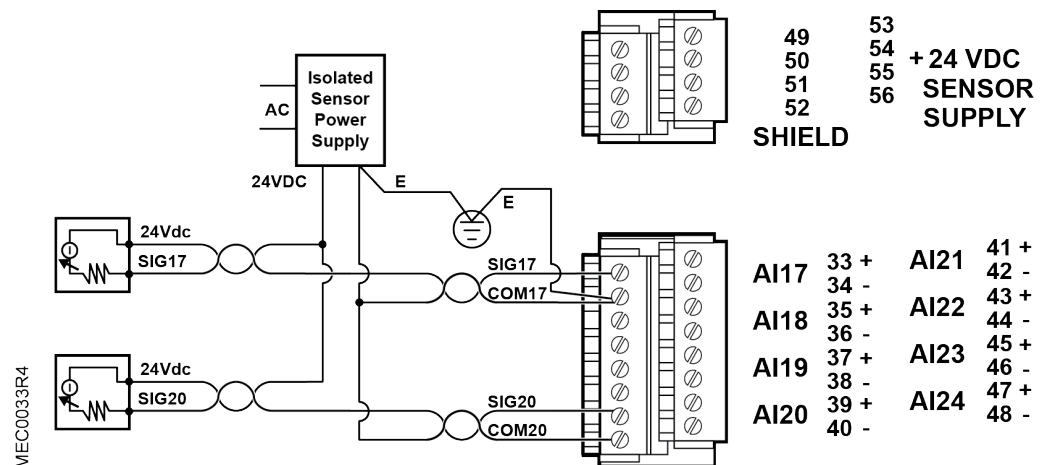
Fig. 106: Connecting an Externally Powered Analog Input (4 to 20 mA).
