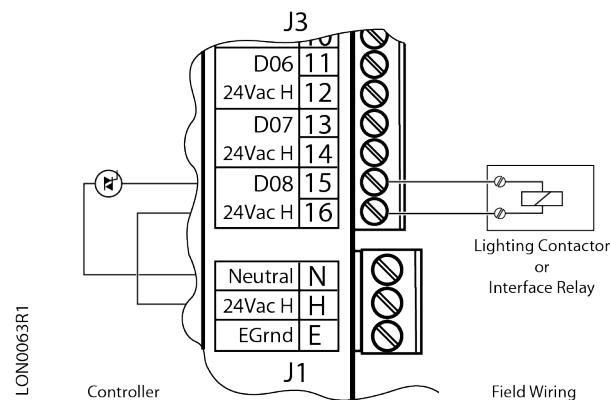
Fig. 166: Lighting Contactor—Maintained Connection to the LTEC.
