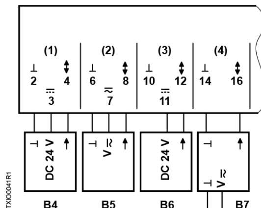
2-wire and 3-wire Active Input (Current); Supervised, Super Universal Modules Only.
