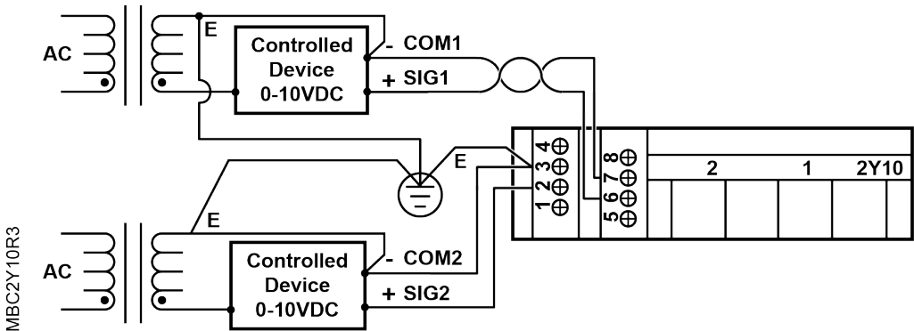
Fig. 128: Connecting an Analog Output (0 to 10 Vdc).
