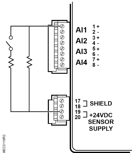
Fig. 117: PXM Wiring Diagram to use an AI as a DI.
