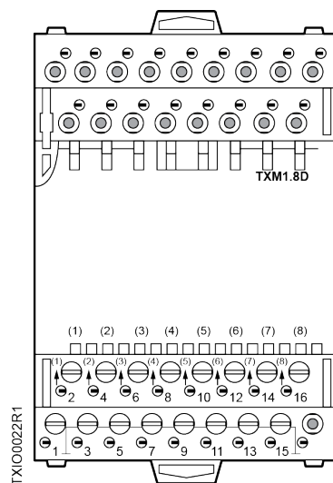
TXM1.8D
