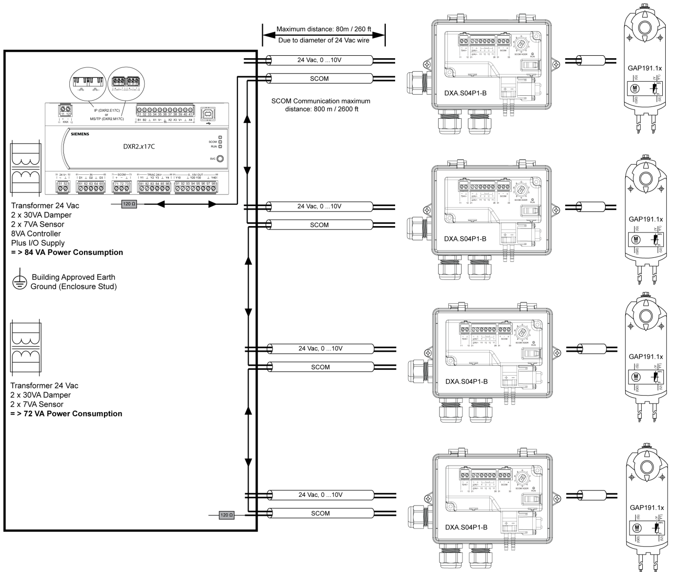
Fig. 90: DXR2.x17CX.. wiring of Sensor/Actuator with four ducts, central transformers, line topology for SCOM.
