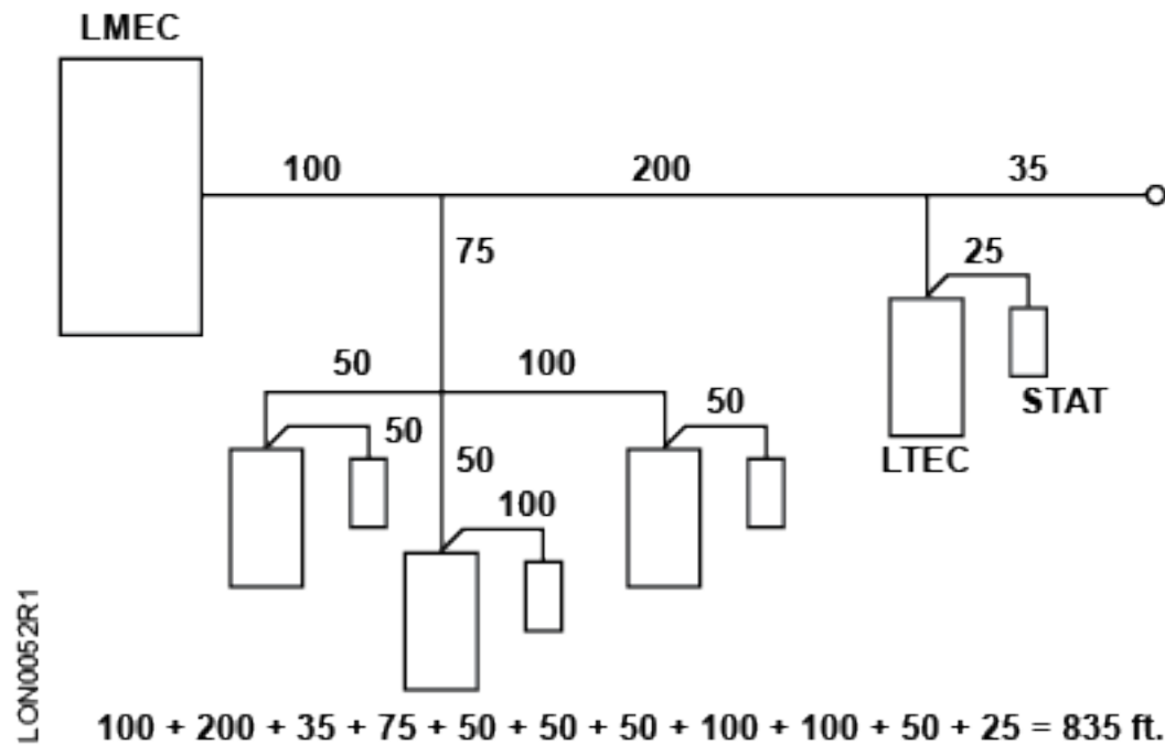
Fig. 36: Determining Network Length—Example.
