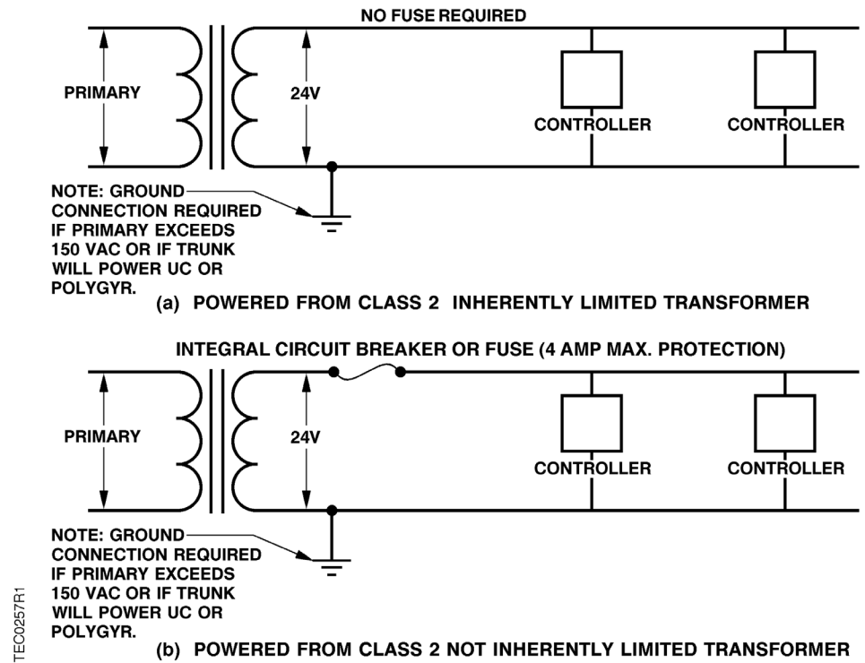
Fig. 38: Power Trunk Layout, Class 2 Circuits.
