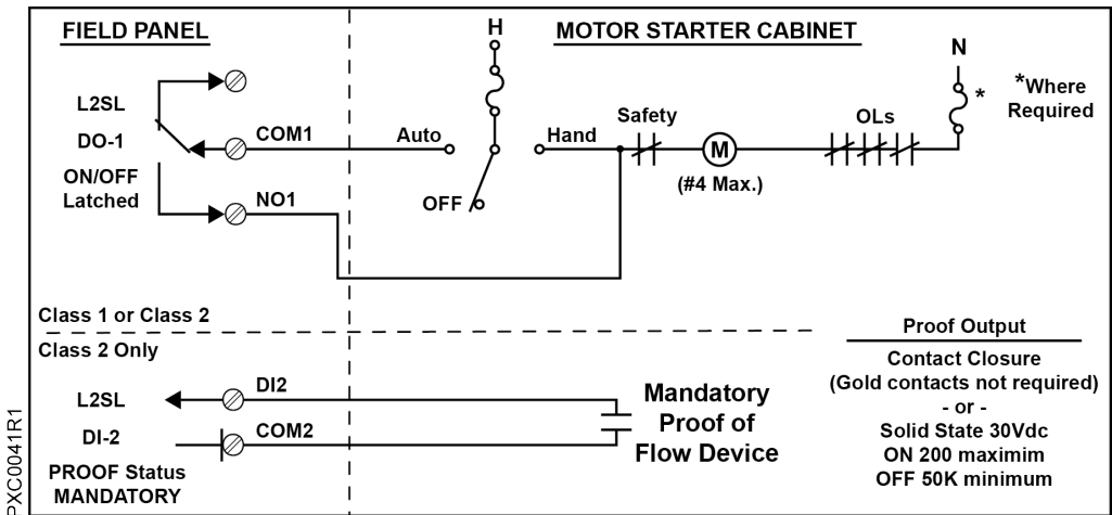
Fig. 47: Connecting an L2SL (Proof Mandatory).
