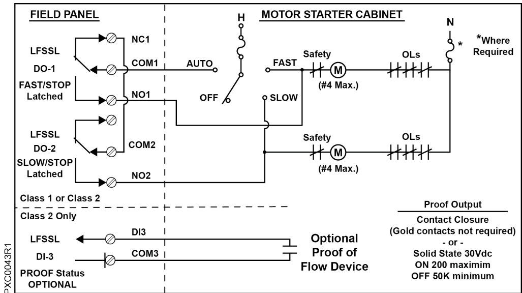
Fig. 43: Connecting an LFSSL (Proof Optional).
