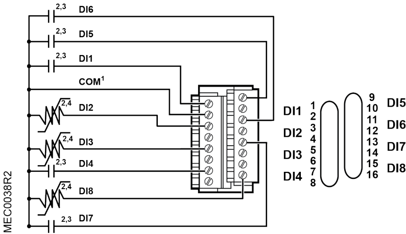
Fig. 113: Connecting a Digital Input (Dry Contacts).
