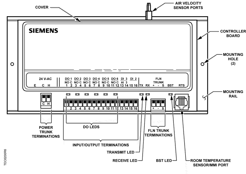
Fig. 172: 6 DO Controller with Air Velocity Sensor.
