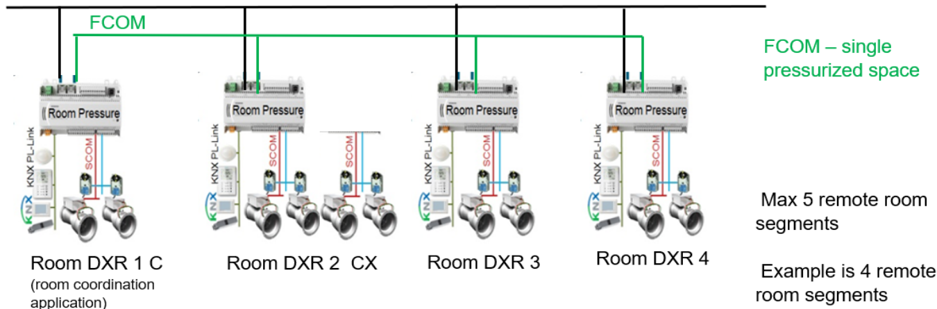
Fig. 73: Lab MS/TP - Common Pressurized Space
