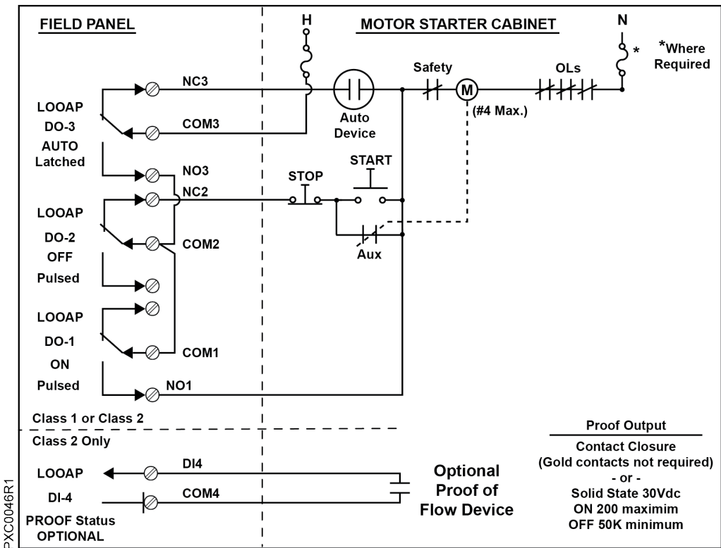
Fig. 46: Connecting an LOOPAP (Proof Optional).
