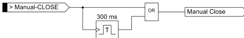
Figure 2-32 Manual close feature
