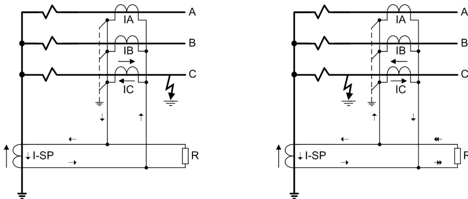
Figure 2-39 Principle of ground fault protection according to the high-impedance principle
