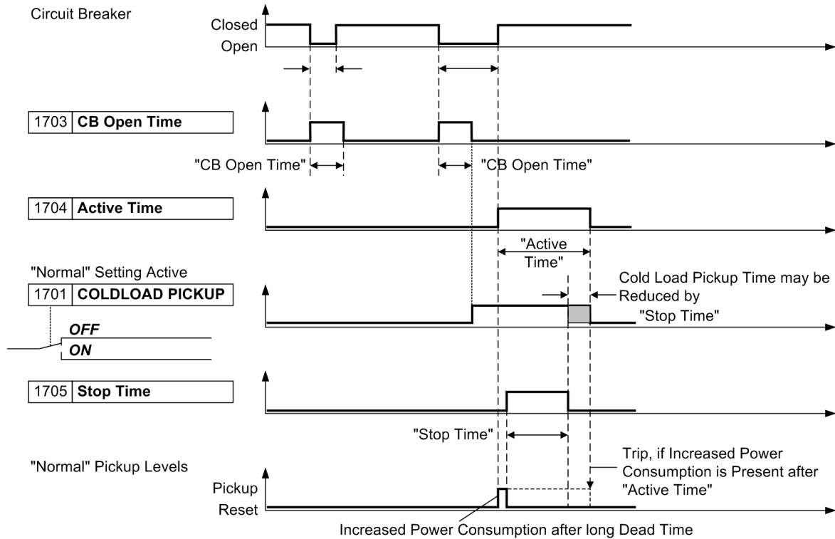
Figure 2-34 Timing charts of the dynamic cold load pickup function
