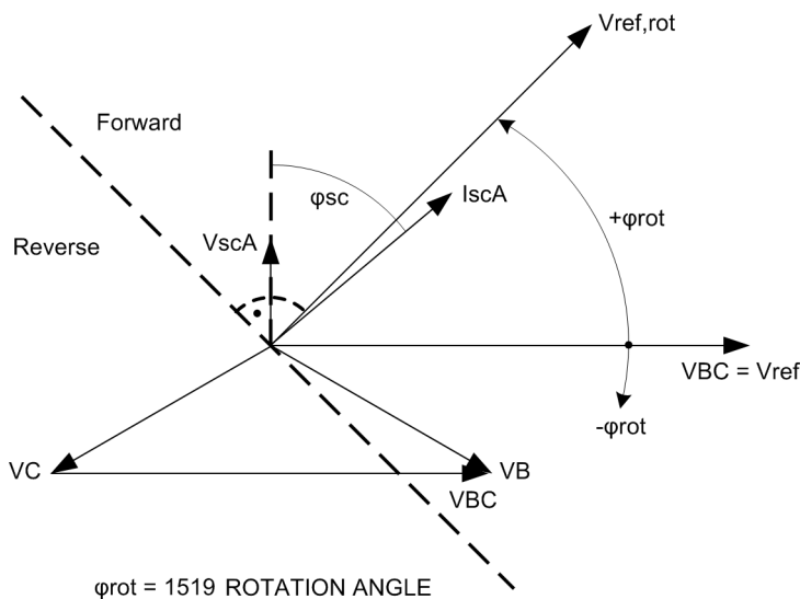
Figure 2-26 Rotation of the reference voltage, directional phase element
