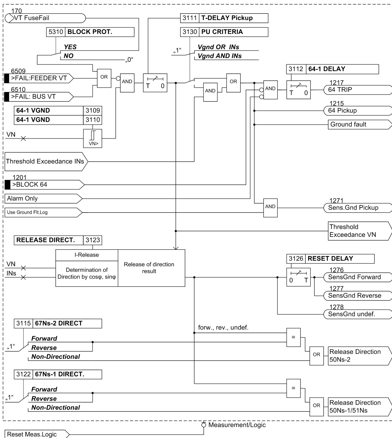
Figure 2-71 Logic diagram of the V_0> element for \cos\phi / \sin\phi measurement
