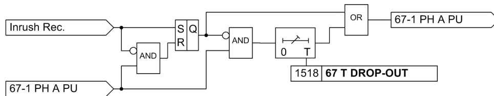
Figure 2-23 Logic of the dropout delay for 67-1
