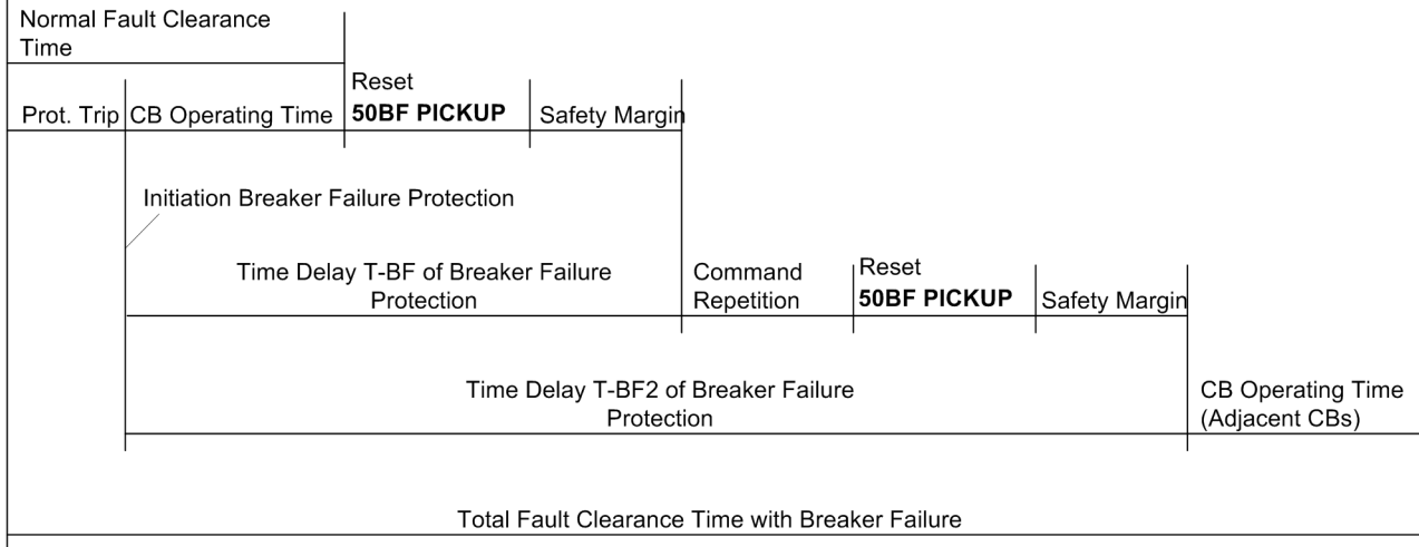
Figure 2-101 Time sequence example for normal clearance of a fault, and for circuit breaker failure with two-element breaker failure protection
