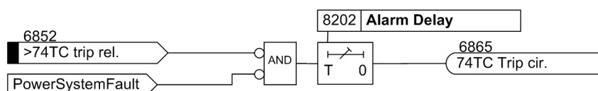
Figure 2-65 Logic diagram of trip circuit supervision with one binary input
