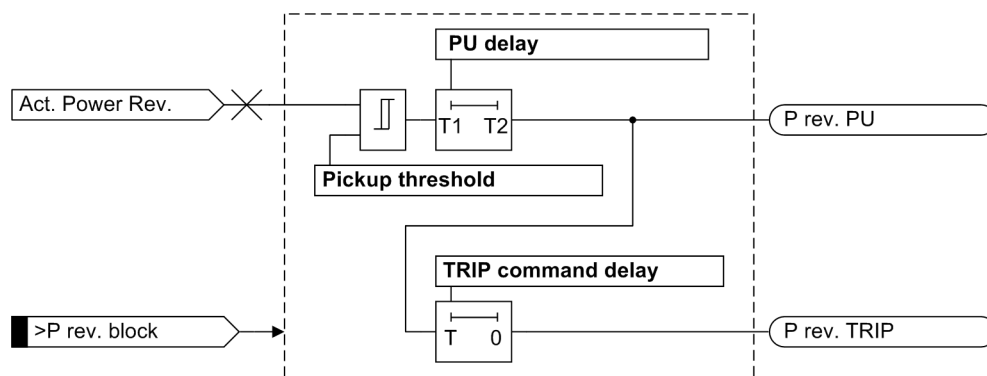
Figure 2-105 Logic diagram of the reverse power determination with flexible protection function
