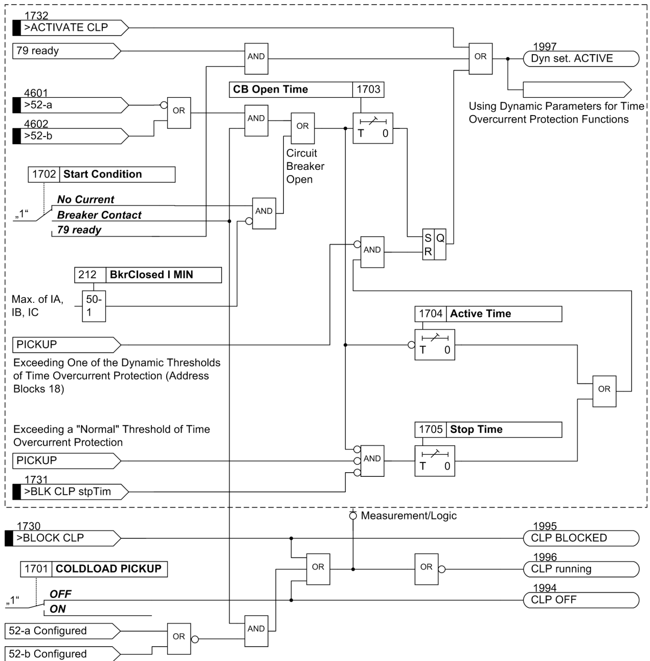
Figure 2-35 Logic diagram of the dynamic cold load pickup function (50c, 50Nc, 51c, 51Nc, 67c, 67Nc)
