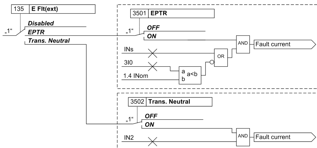
Figure 2-78 Activation of the Functions EPTR or Transformer Neutral Point (TNP)
