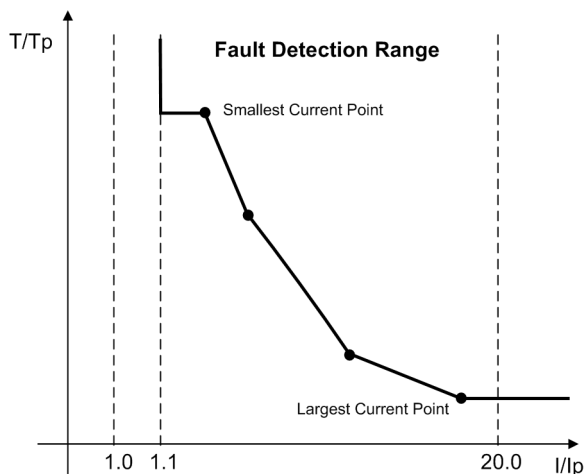
Figure 2-83 Use of a user-defined characteristic
