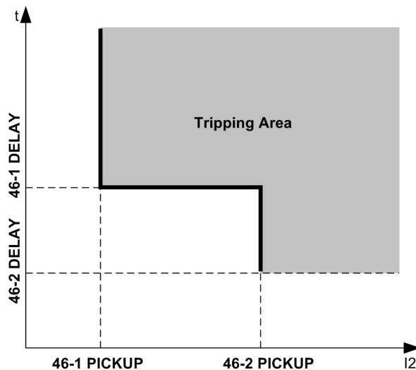
Figure 2-48 Definite time characteristic for negative sequence protection
