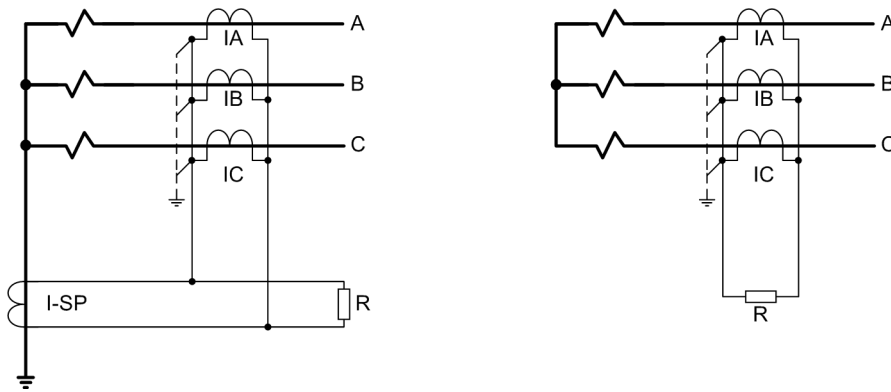
Figure 2-38 Ground fault protection according to the high-impedance principle
