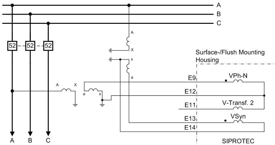
Figure C-17 Example for connection type "Vph-n, Vsyn"
