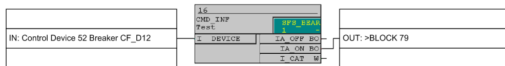
Figure 2-95 Blocking of the automatic reclose function using the internal control function
