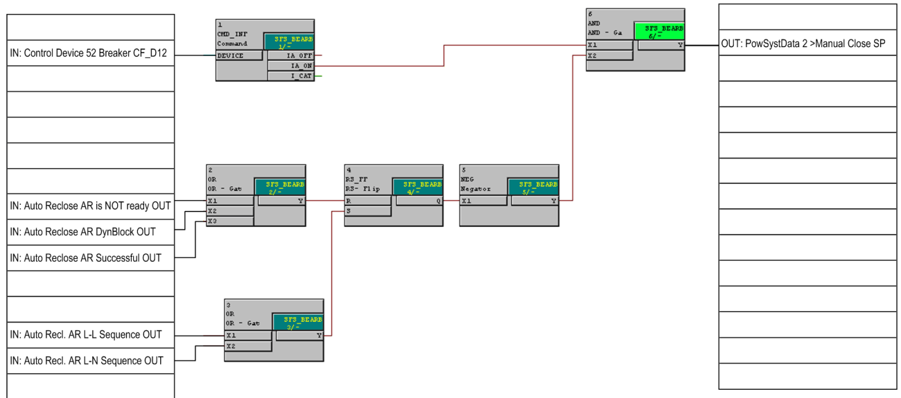
Figure 2-94 CFC logic for Manual Close with automatic reclosing via control
