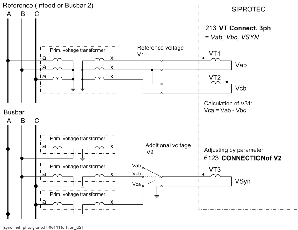
Figure 2-118 Phase-to-phase voltage connection (open-delta connection)
