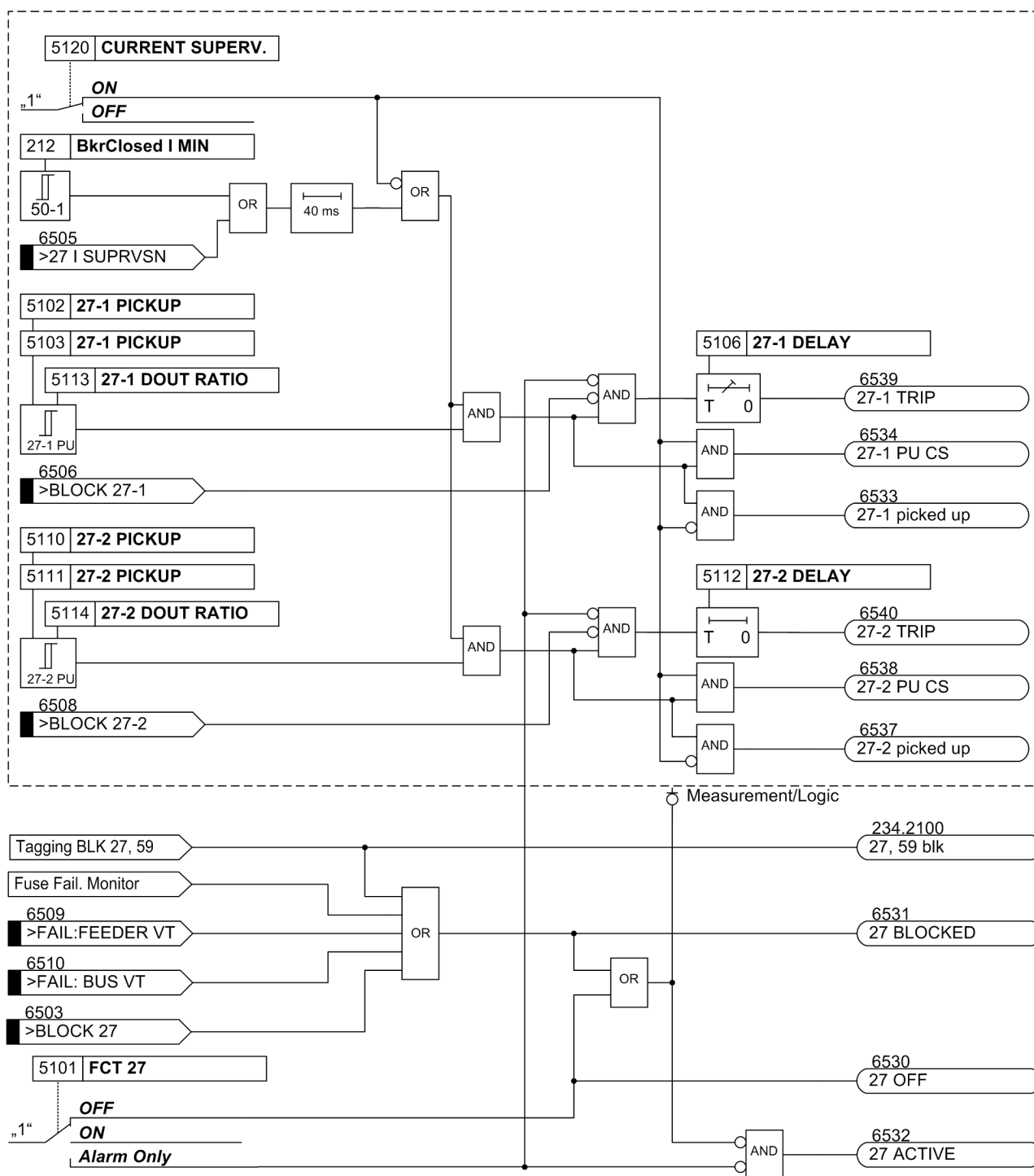
Figure 2-47 Logic diagram of the undervoltage protection
