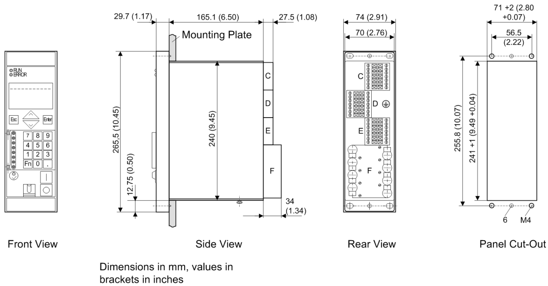
Figure 4-12 Dimensional drawing of a 7SJ80 for panel flush or cubicle mounting (housing size 1/6)
