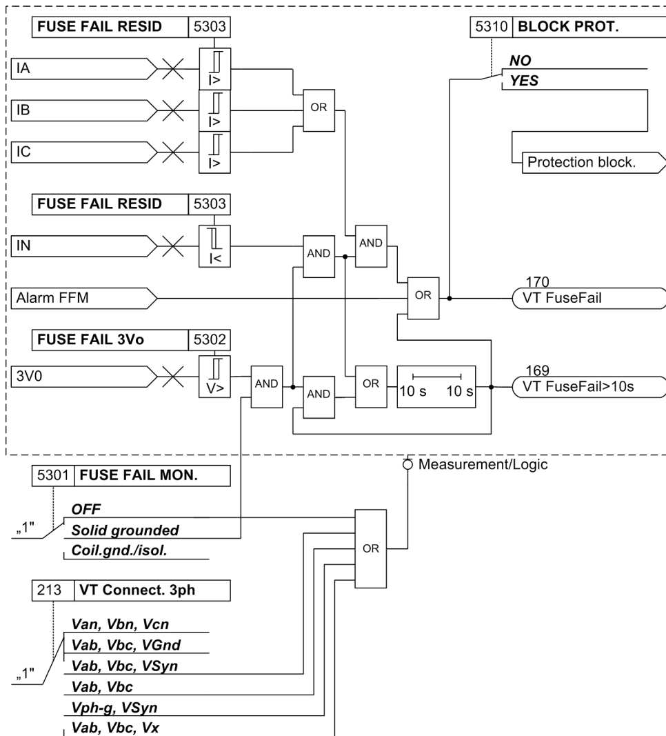
Figure 2-59 Logic diagram of the Fuse Failure Monitor for grounded networks only
