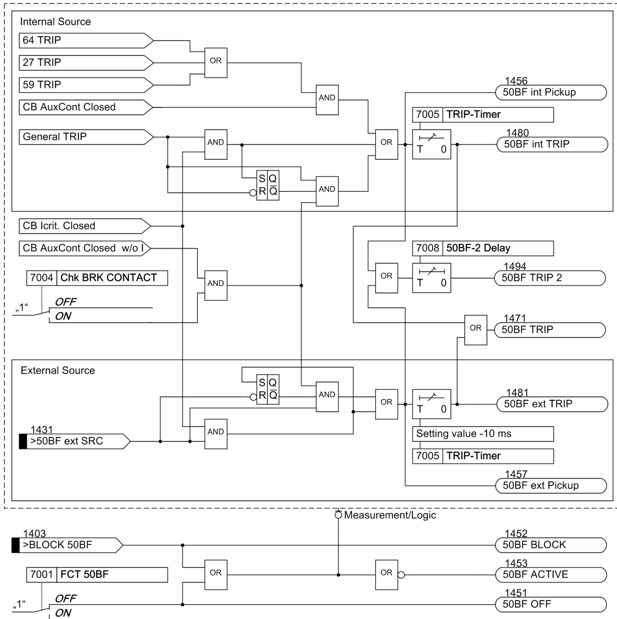
Figure 2-99 Logic diagram of the breaker failure protection
