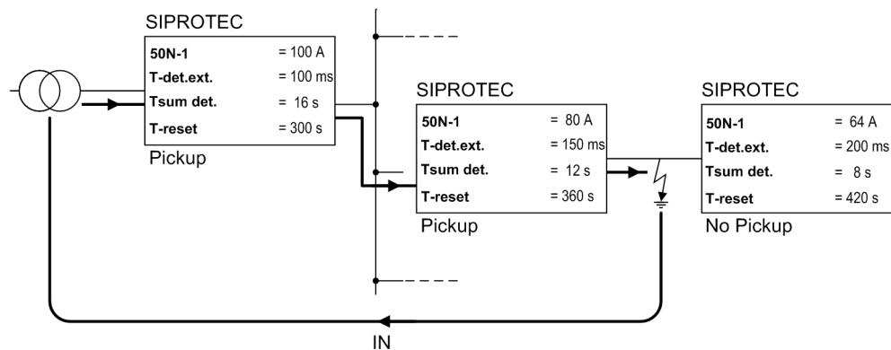
Figure 2-87 Example of selectivity criteria of the intermittent ground fault protection
