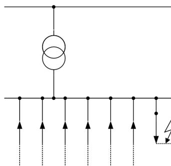
Figure 2-81 Location of ground faults in a radial network
