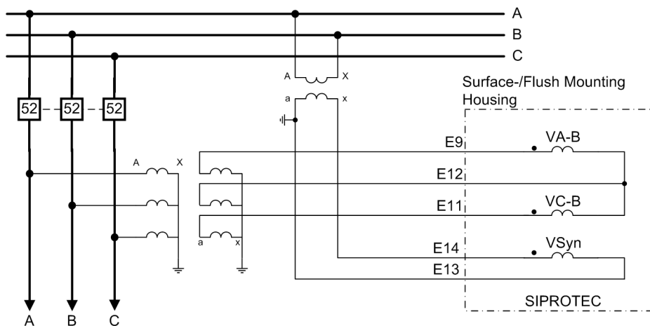
Figure C-21 Example for connection type "VAB, VBC, VSYN"
