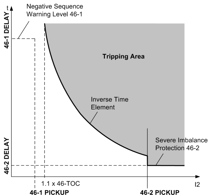
Figure 2-49 Inverse time characteristic for negative sequence protection
