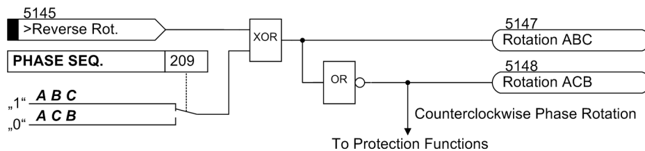
Figure 2-120 Message logic of the phase rotation reversal
