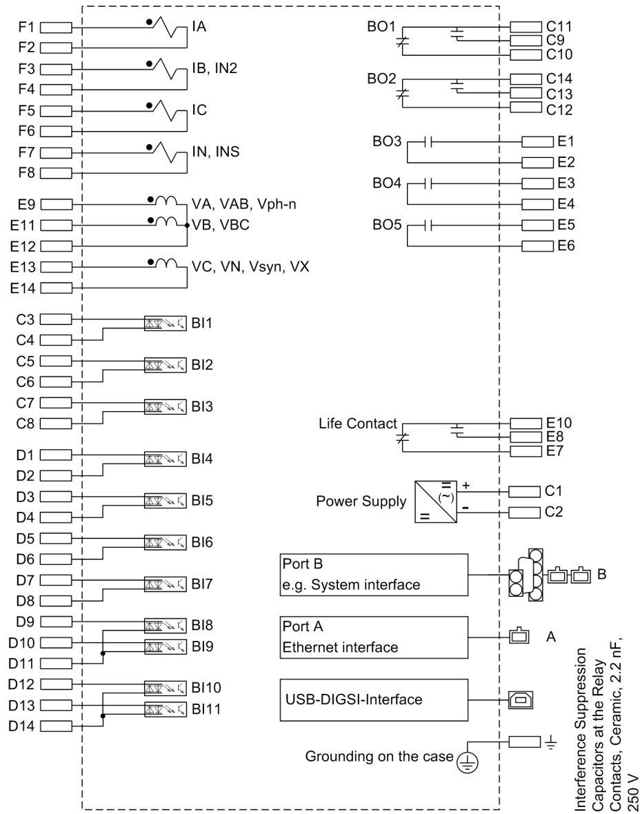
Figure B-6 Block diagram 7SJ808*
