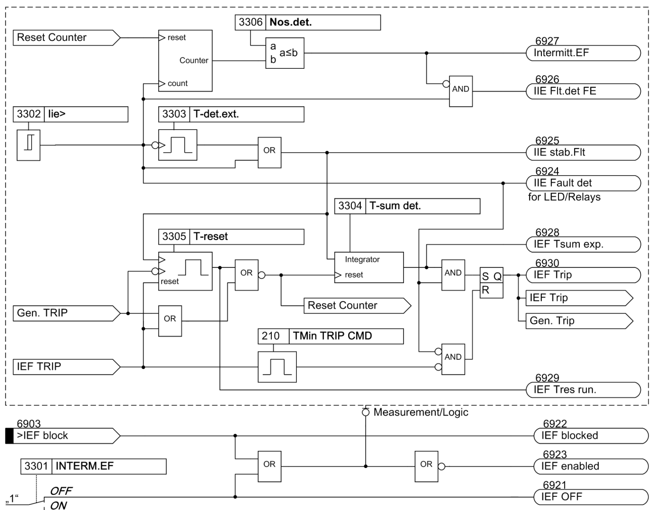
Figure 2-86 Logic diagram of the intermittent ground fault protection – principle
