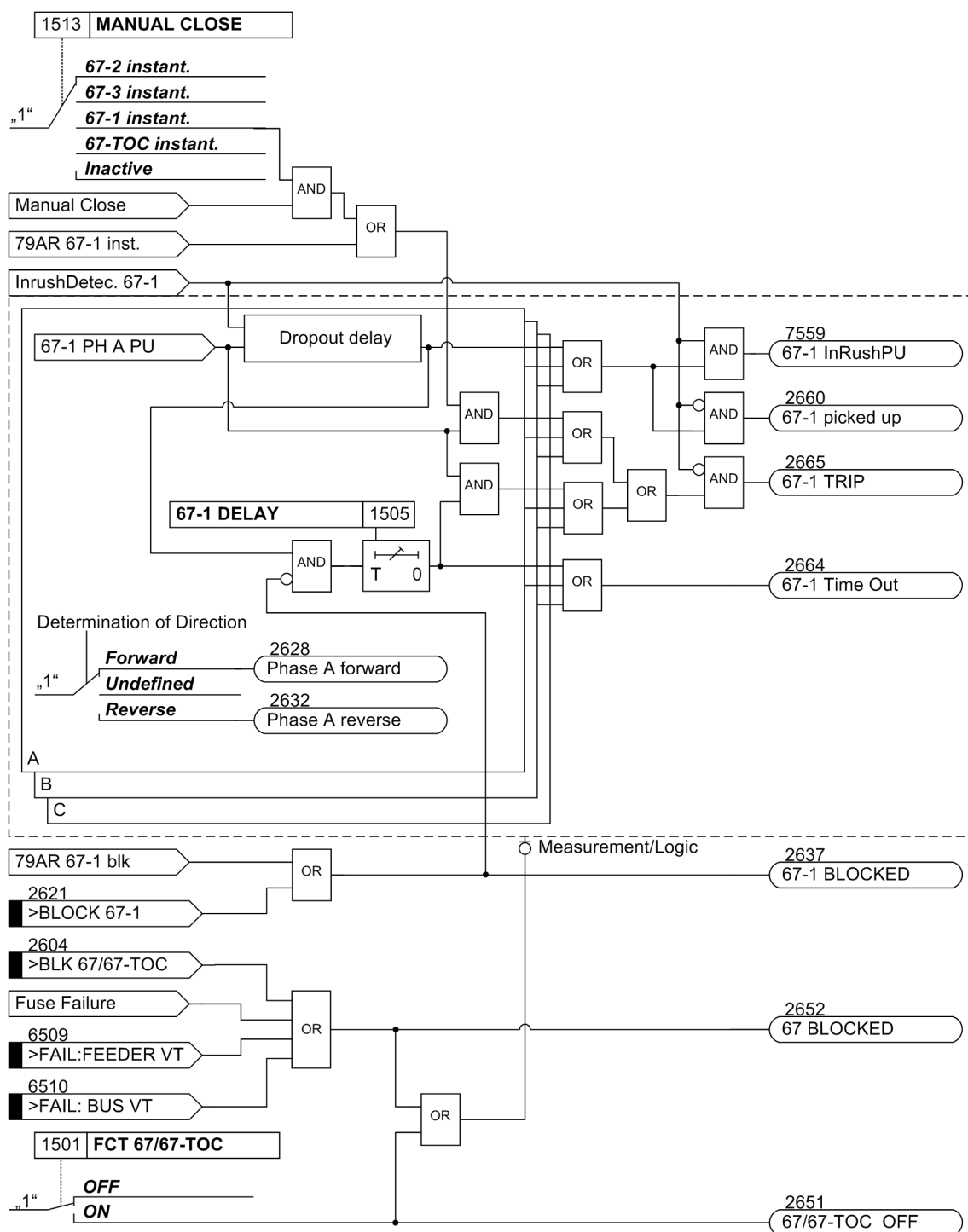
Figure 2-22 Logic diagram for the directional relay element 67-1 for phases
