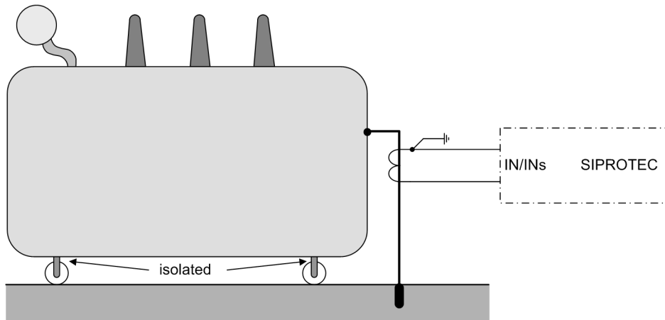
Figure 2-41 Principle of tank-leakage protection
