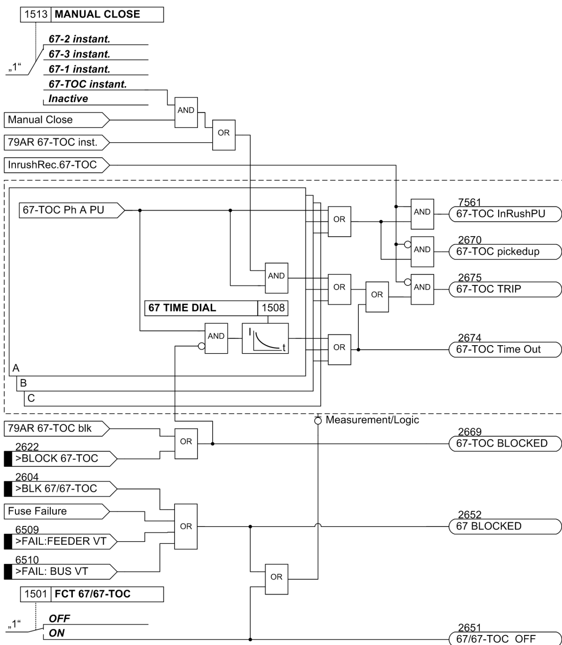
Figure 2-24 Logic diagram for the directional overcurrent protection: 67-TOC relay element
