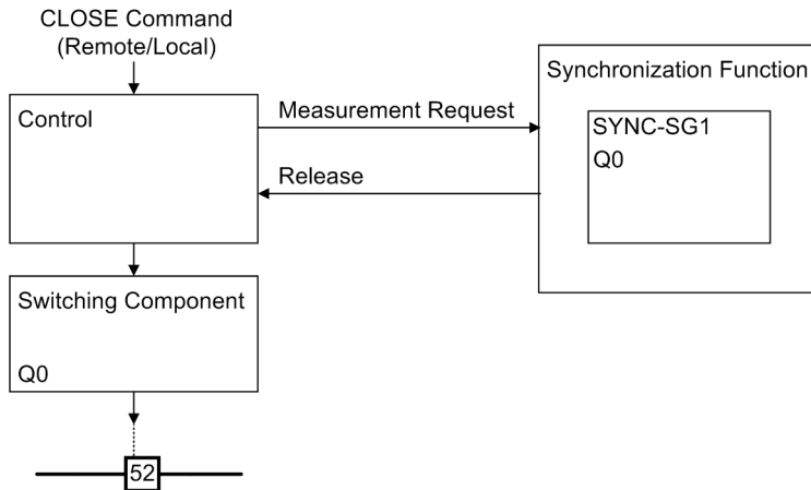
Figure 2-114 Interaction of control and synchrocheck function
