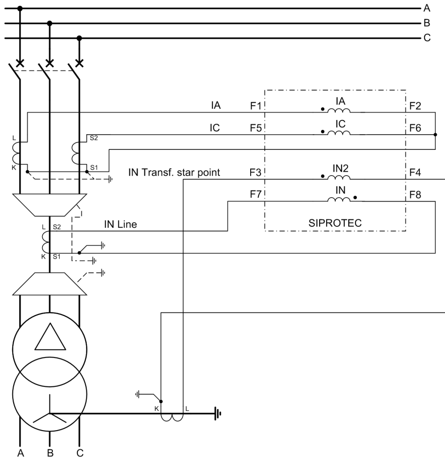
Figure C-12 Current transformer connections to two phase currents and two ground currents; IN/INs – ground current of the line, IN2 – ground current of the transformer starpoint
