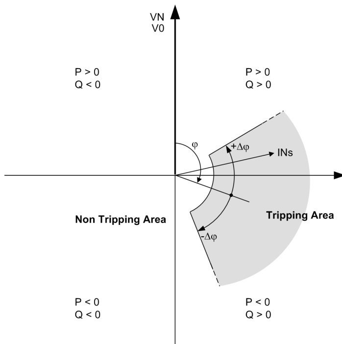
Figure 2-74 Tripping range of V_0 - I_0 - \phi characteristic
