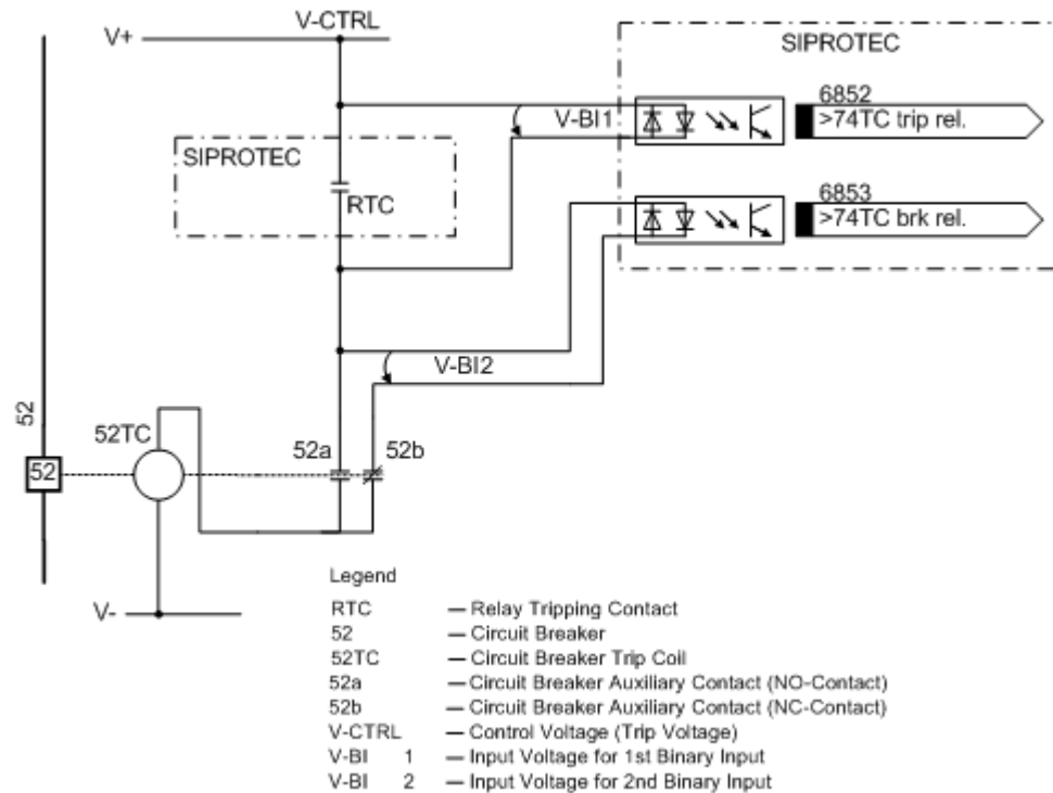
Figure 2-62 Principle of the trip circuit supervision with two binary inputs
