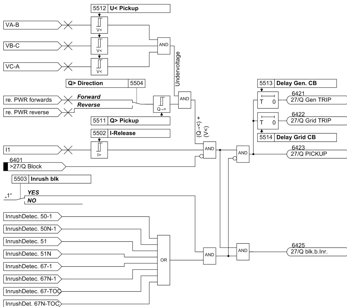
Figure 2-52 Logic diagram of the QU protection
