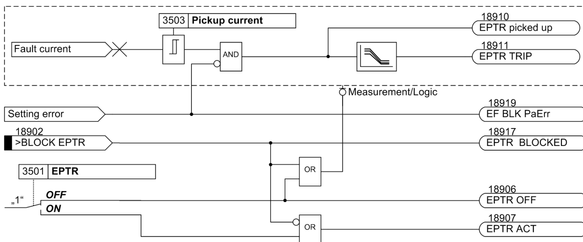
Figure 2-79 Logic of the Ground-Fault Detection EPTR
