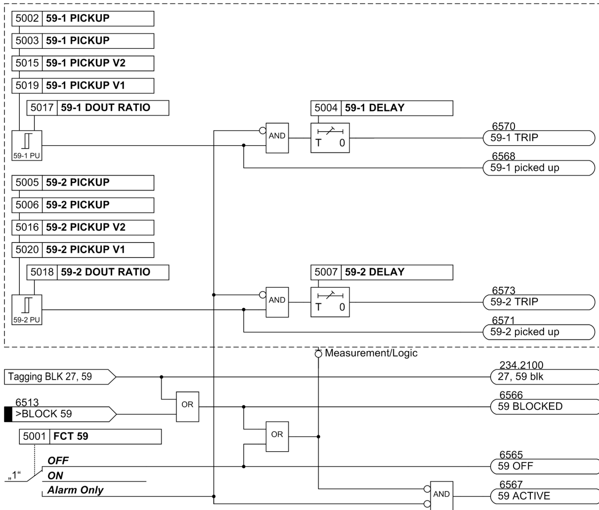
Figure 2-44 Logic diagram of the overvoltage protection
