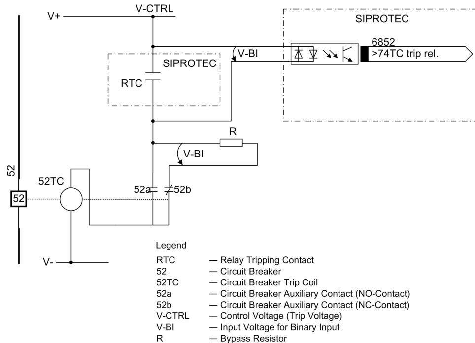
Figure 2-64 Trip circuit supervision with one binary input
