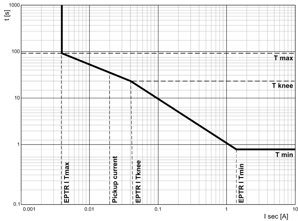
Figure 4-11 Tripping Time Characteristic Curves of the Inverse-Time Ground-Fault Protection with Logarithmic-Inverse Knee-Point Characteristic Curve, Example EPTR
