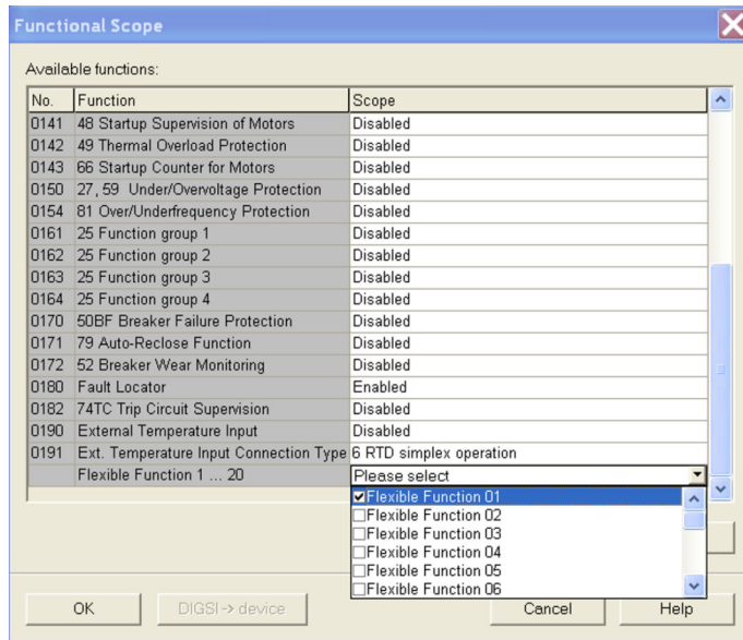
Figure 2-106 Configuration of a flexible protection function
