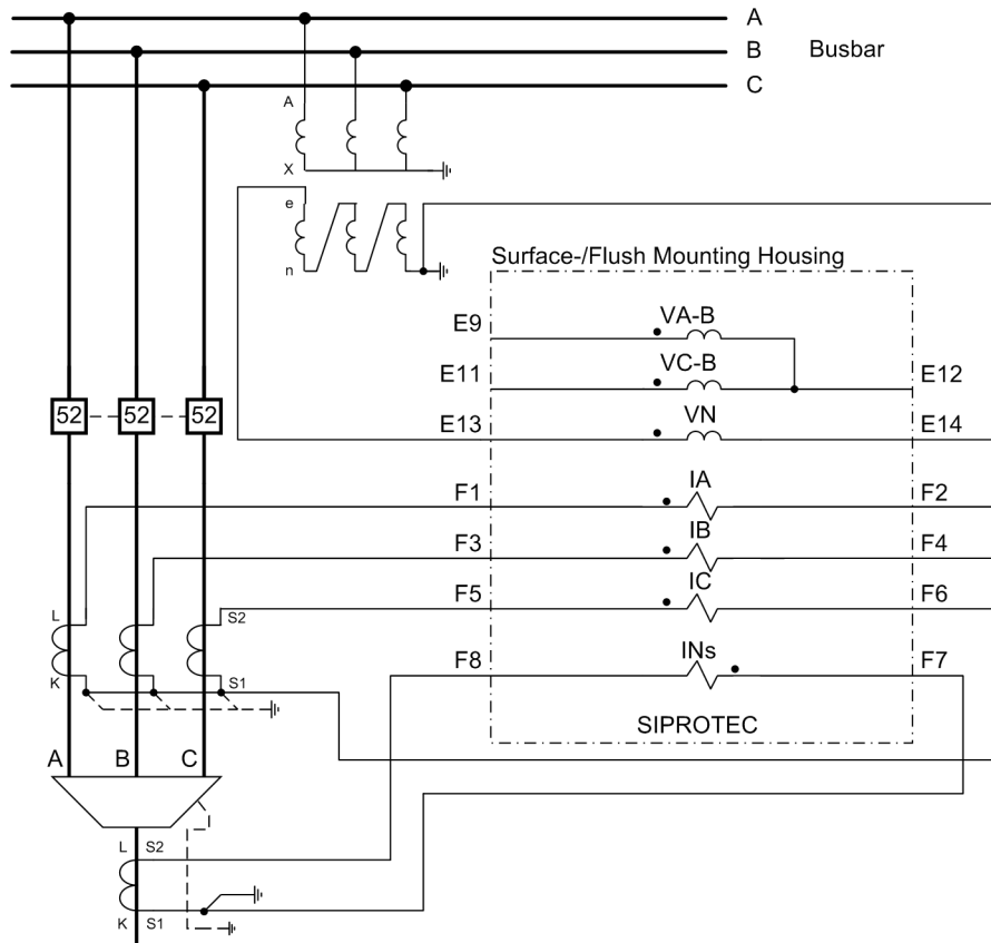
Figure C-10 Transformer connections to three current transformers, cable-type current transformer and broken delta winding, maximum precision for sensitive ground fault detection
