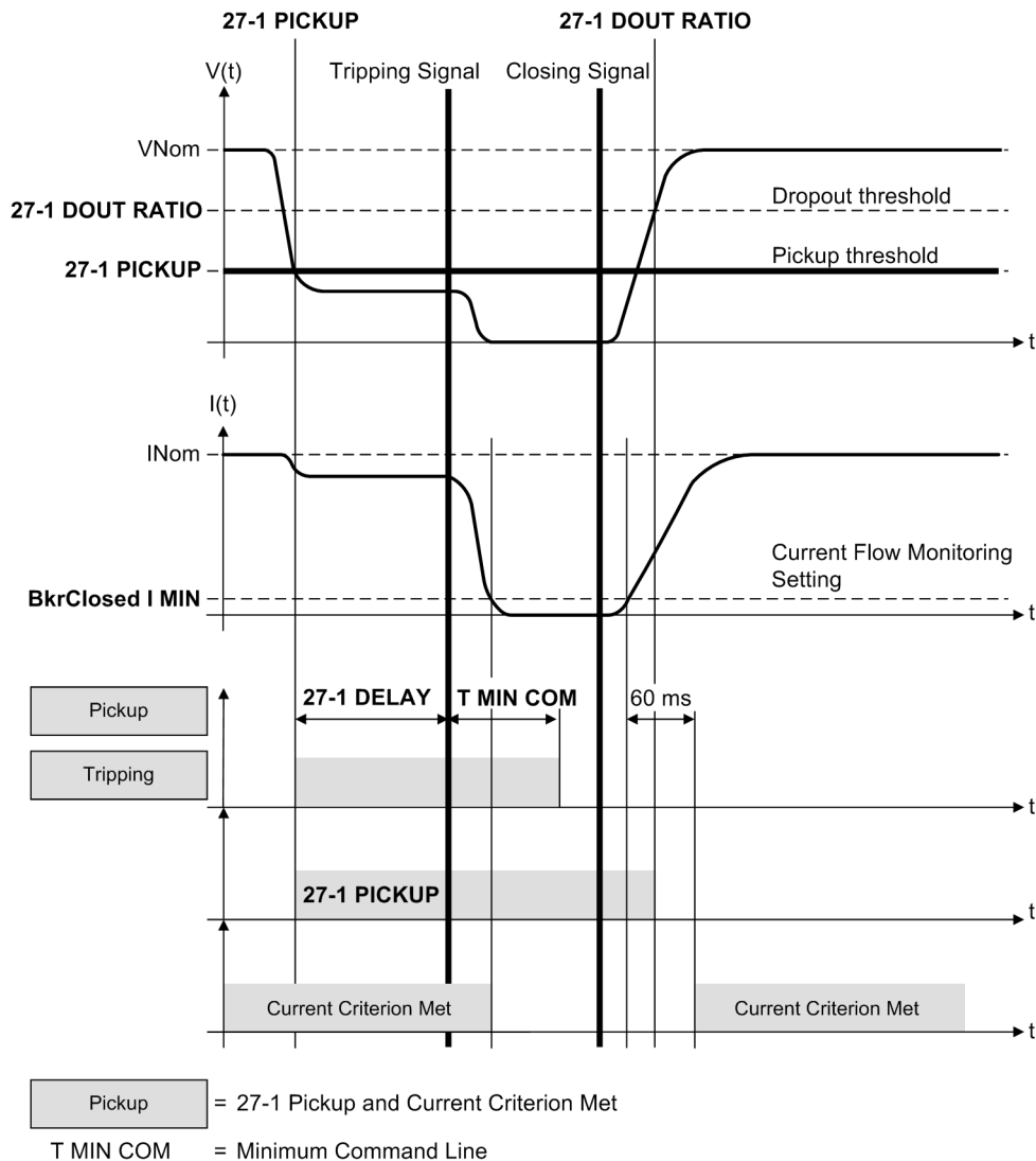
Figure 2-46 Typical fault profile for load side connection of the voltage transformers (with current supervision)
