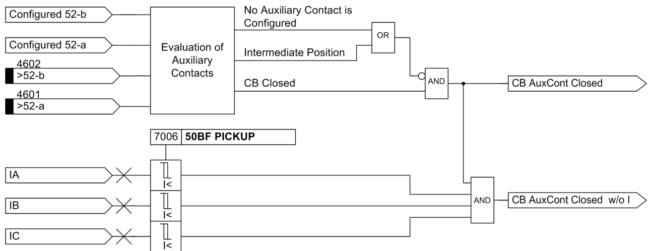
Figure 2-98 Logic diagram for breaker failure protection, monitoring of the circuit-breaker auxiliary contacts
