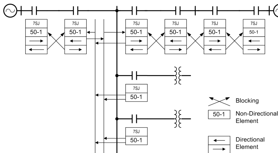
Figure 2-30 Reverse interlocking using directional elements
