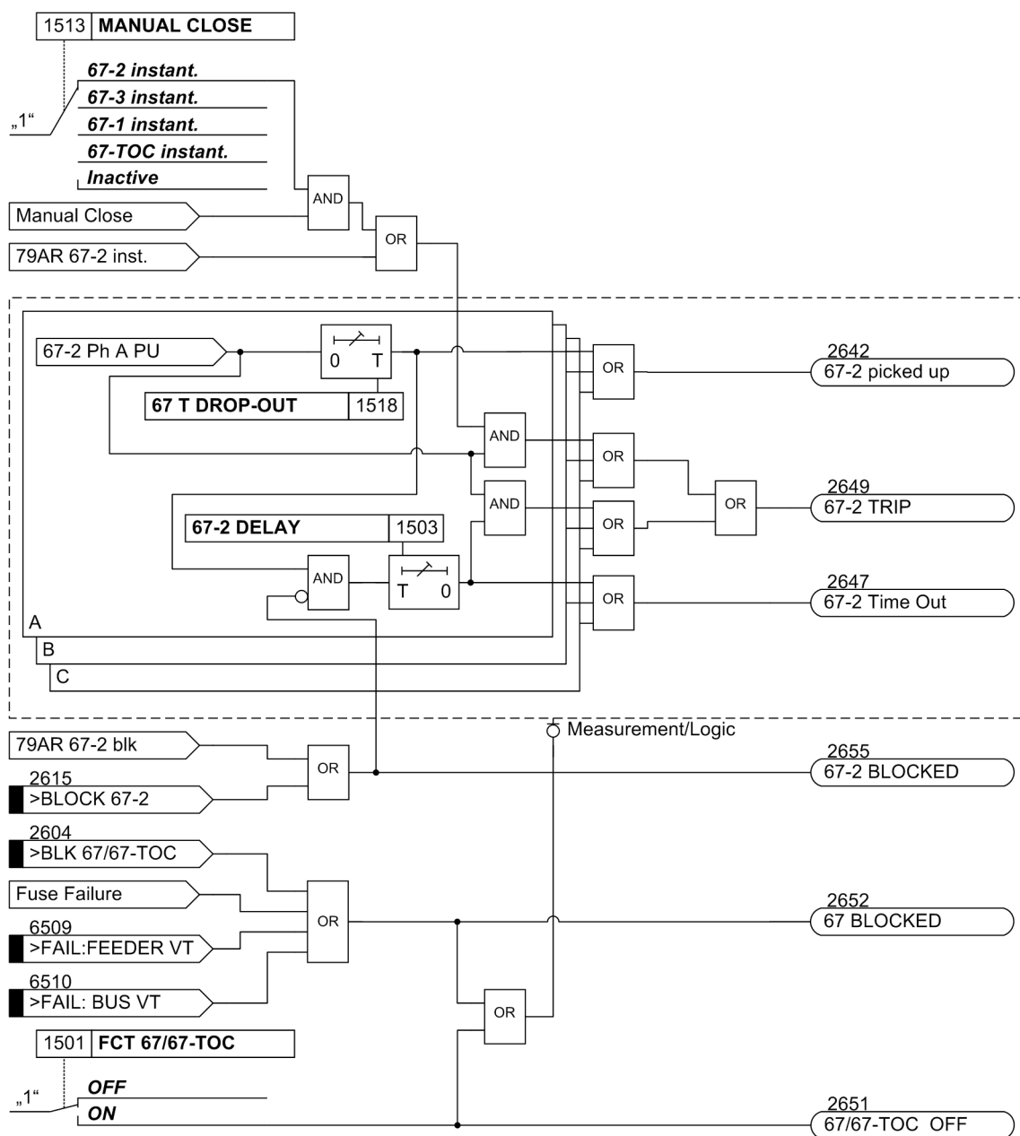
Figure 2-21 Logic diagram for directional high-set element 67-2 for phases
