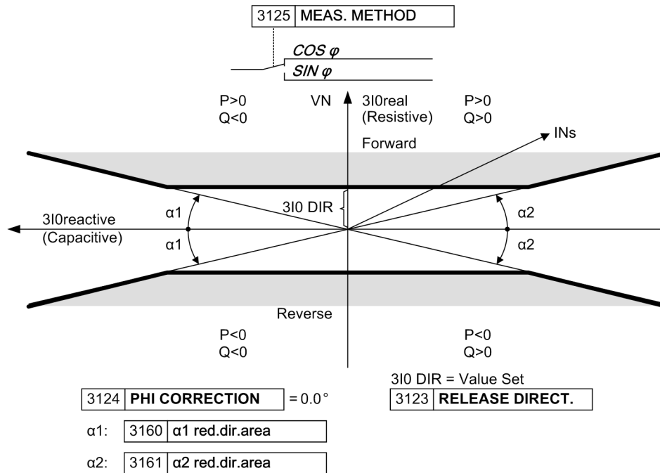
Figure 2-68 Directional characteristic for \cos\phi -measurement
