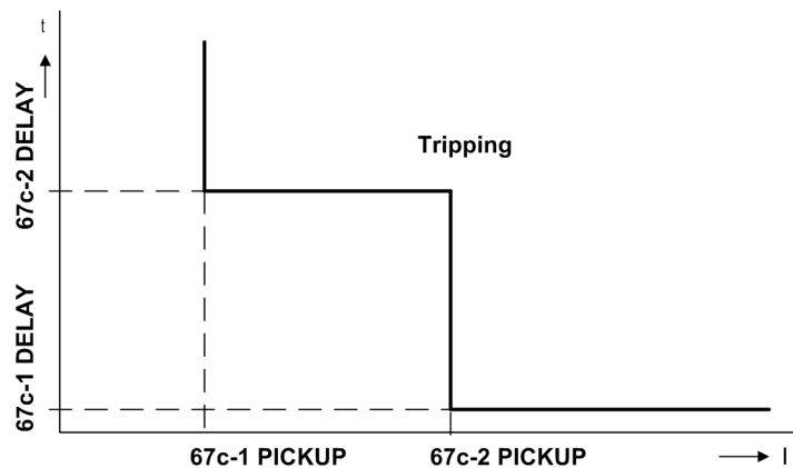
Figure 2-36 Two-stage characteristic of the single-phase time-overcurrent protection
