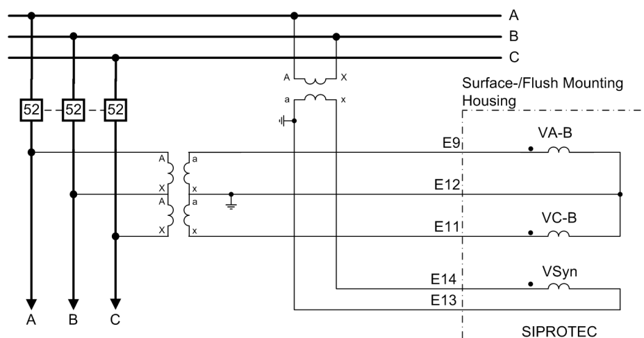
Figure C-22 Example for connection type "VAB, VBC, VSYN" with phase voltage connection as open-delta connection
