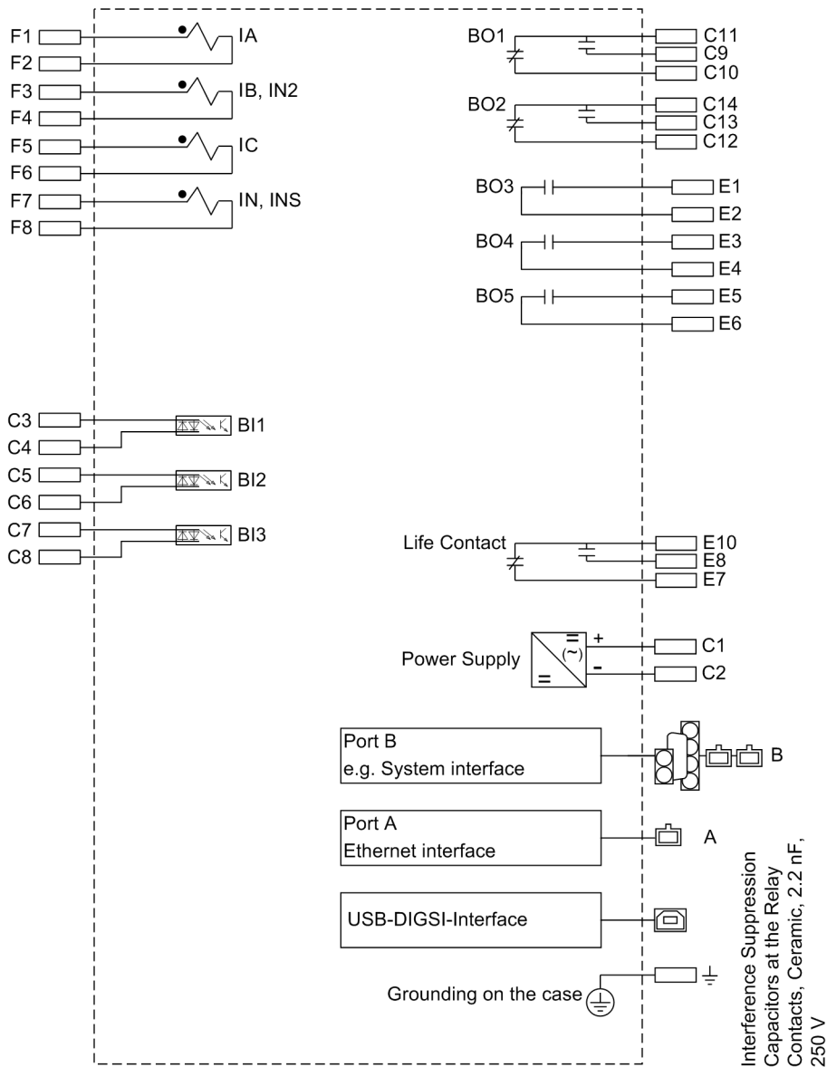
Figure B-1 Block diagram 7SJ801*
