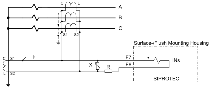
Figure C-13 High-impedance differential protection for a grounded transformer winding (the illustration shows the partial connection for high-impedance differential protection)
