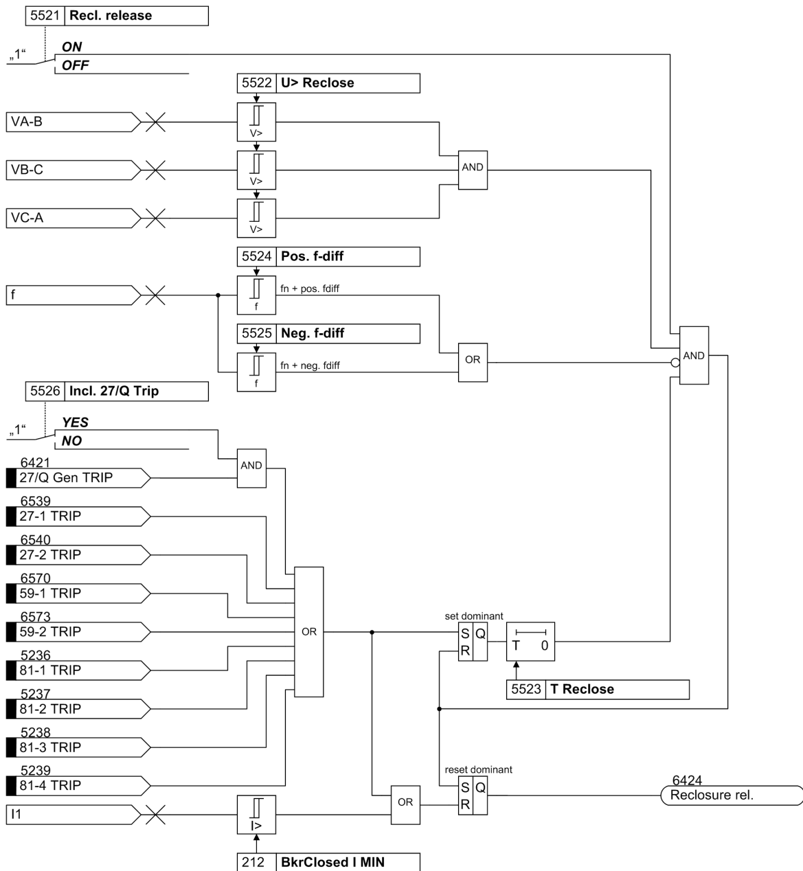
Figure 2-53 Logic diagram of QU protection restarting
