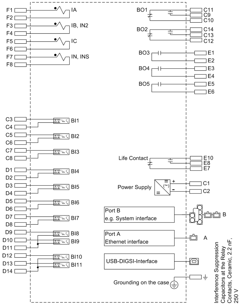
Figure B-5 Block diagram 7SJ807*
