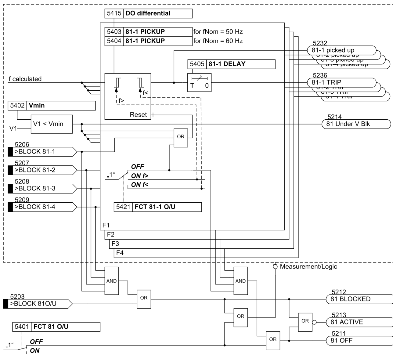
Figure 2-51 Logic diagram of the frequency protection
