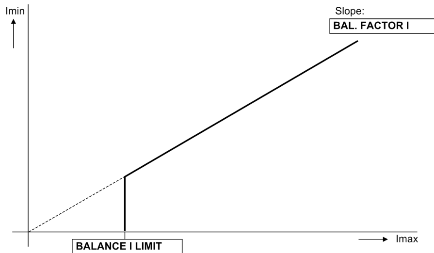
Figure 2-57 Current symmetry monitoring
