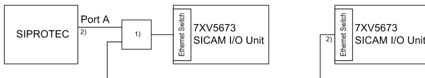
Figure C-23 Connection of 2 SICAM I/O units to port A via Y cable (up to 2 SICAM I/O units connectable)
