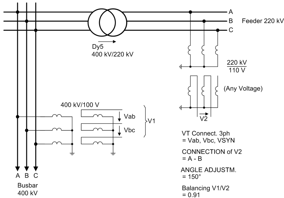
Figure 2-117 Busbar voltage measured across the transformer
