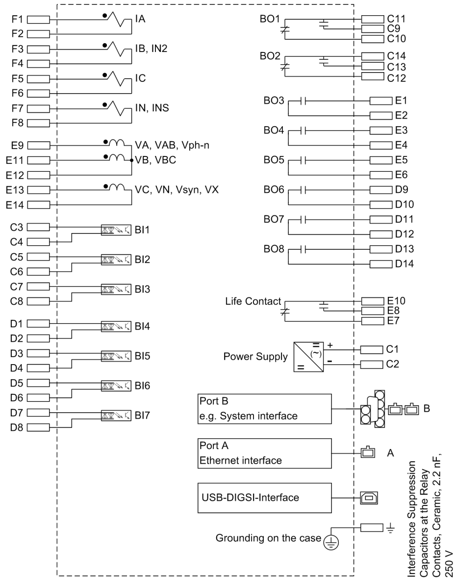
Figure B-4 Block diagram 7SJ804*
