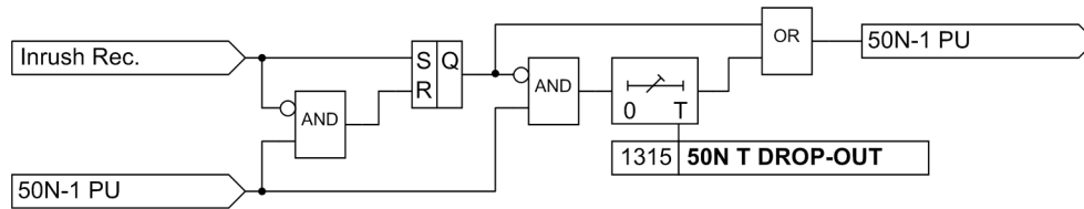
Figure 2-9 Logic of the dropout delay for 50N-1
