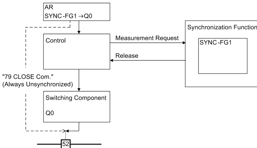
Figure 2-115 Connection of the automatic reclosing function to the synchrocheck function
