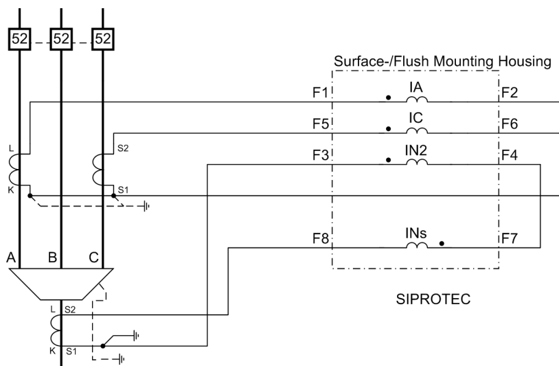
Figure C-11 Current transformer connections to two phase-current transformers and a ground-current transformer; the ground current is taken via the highly sensitive and sensitive ground input.
