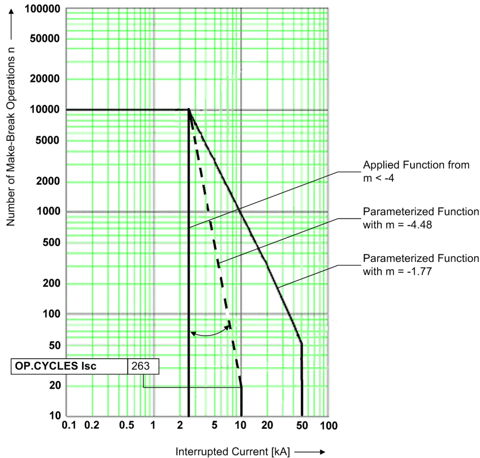
Figure 2-126 Value limitation of directional coefficient
