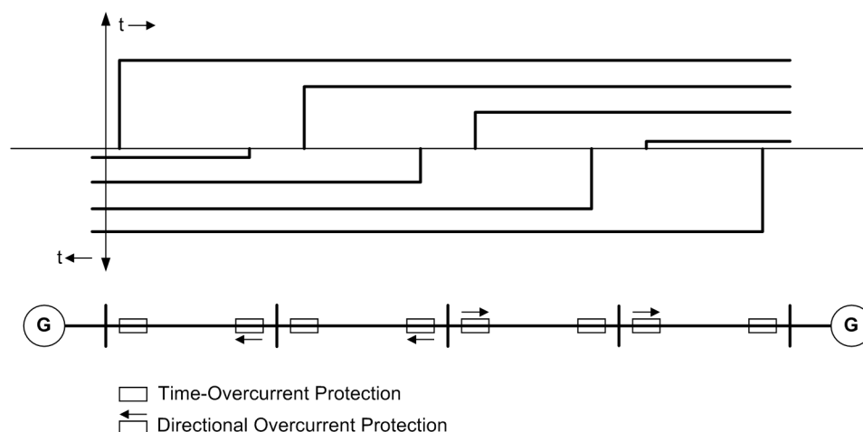
Figure 2-20 Transmission lines with sources at both ends
