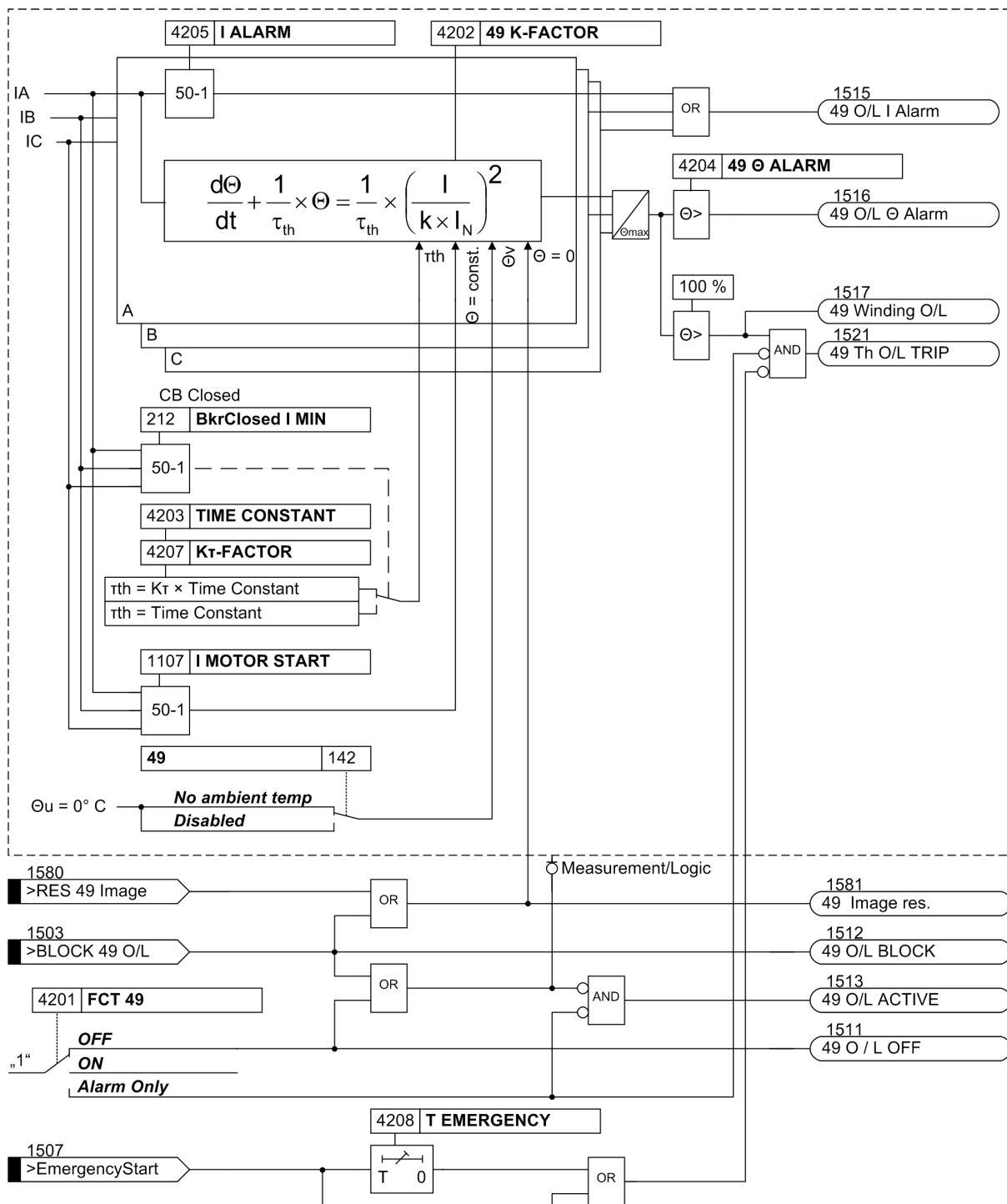
Figure 2-54 Logic diagram of the overload protection
