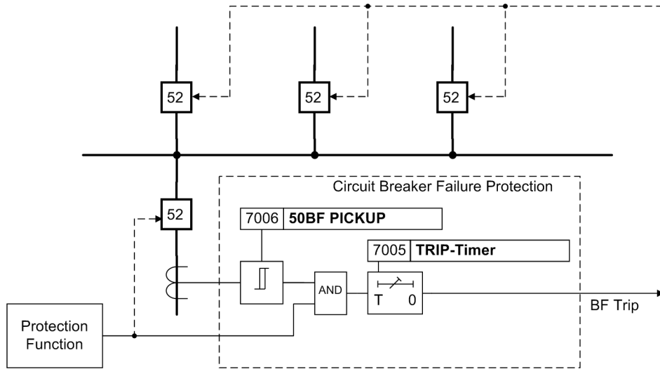
Figure 2-96 Function principle of the breaker failure protection
