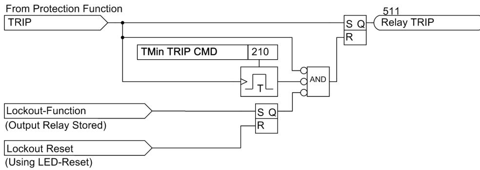
Figure 2-121 Terminating the Trip Signal
