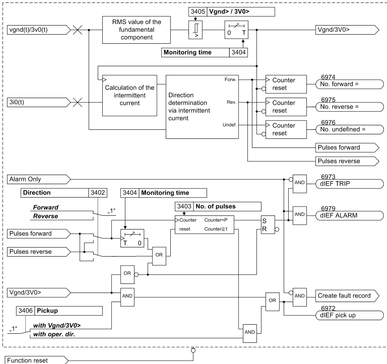
Figure 2-89 Logic diagram of the directional intermittent ground fault protection
