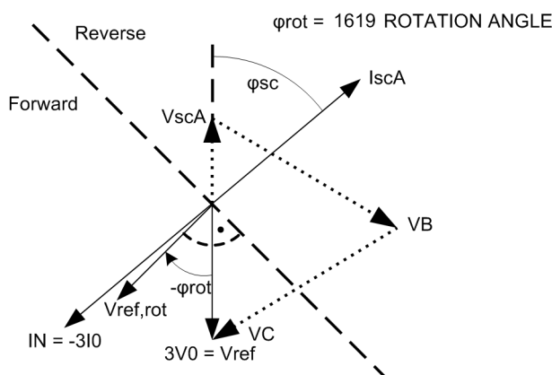
Figure 2-28 Rotation of the reference voltage, directional ground element with zero sequence values
