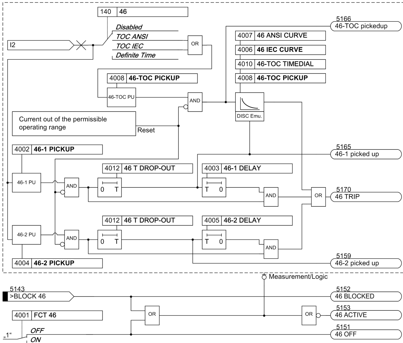
Figure 2-50 Logic diagram of the unbalanced load protection
