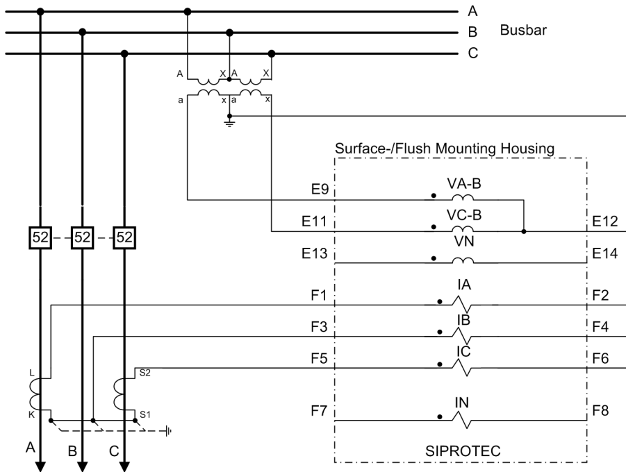
Figure C-8 Current transformer connections to two current transformers and as open-delta connection the voltage transformer – for isolated or resonant-grounded networks when no directional ground protection is needed
