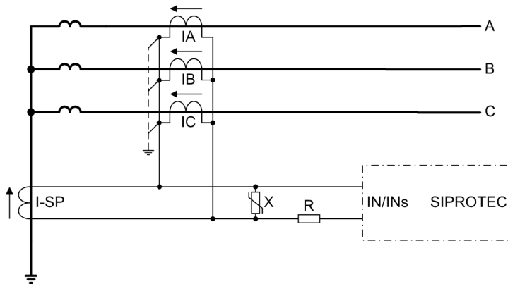
Figure 2-43 Connection diagram of the ground fault differential protection according to the high-impedance principle
