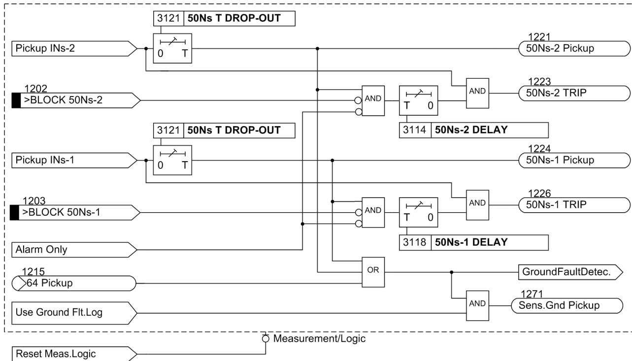
Figure 2-77 Logic diagram for V0-I/0 -φ measurement, part 2
