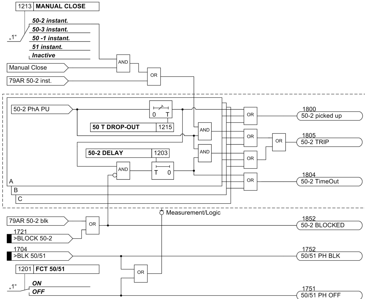
Figure 2-4 Logic diagram for 50-2 high-set element for phases
