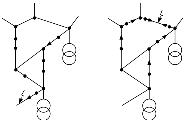
Figure 2-82 Determination of the ground fault location basing on directional indicators in the meshed system
