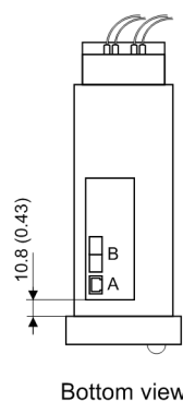
Figure 4-14 Bottom view of a 7SJ80 (housing size 1/6)
