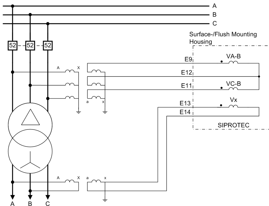
Figure C-18 Example for connection type "VAB, VBC, Vx"
