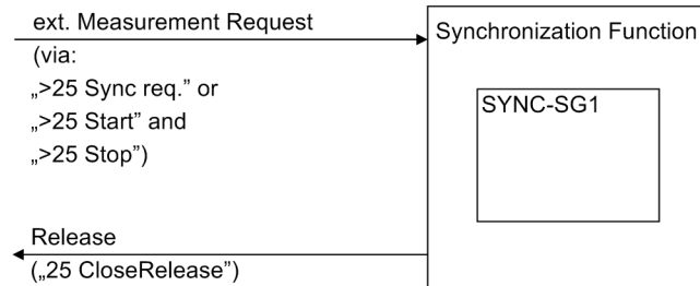
Figure 2-116 Interaction of synchrocheck function and external control
