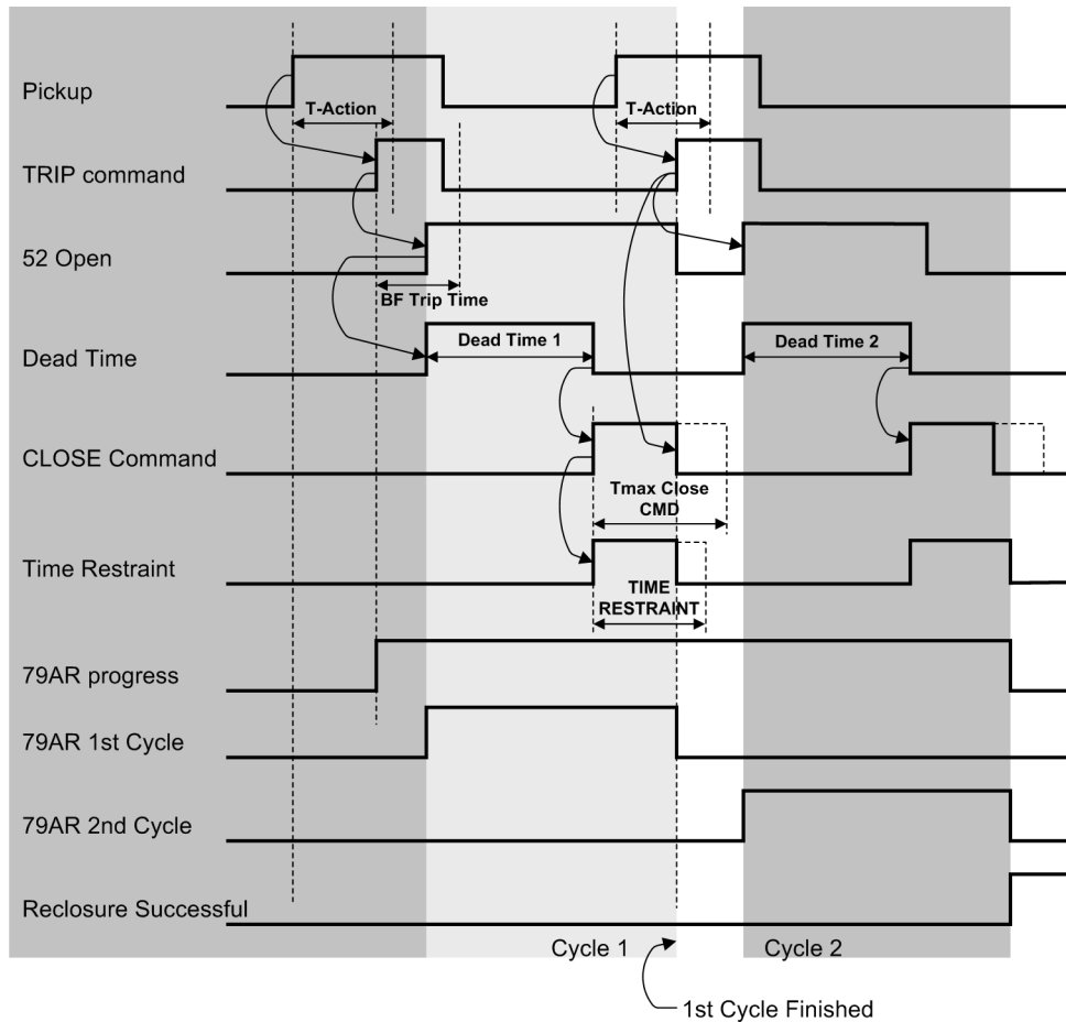
Figure 2-90 Timing diagram showing two reclosing shots, first cycle unsuccessful, second cycle successful
