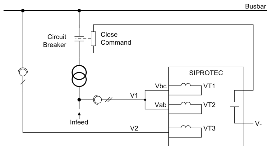
Figure 2-112 Infeed
