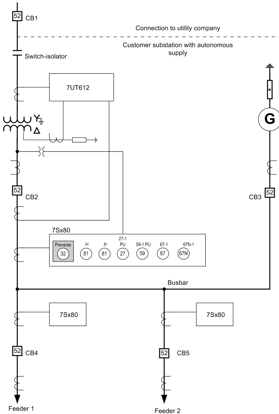
Figure 2-103 Example of a substation with autonomous generator supply
