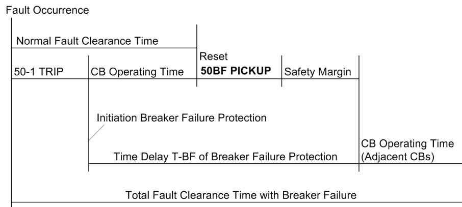
Figure 2-100 Time sequence example for normal clearance of a fault, and for circuit breaker failure with single-element breaker failure protection
