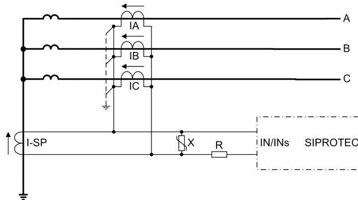
Figure 2-40 Connection diagram of the ground fault differential protection according to the high-impedance principle
