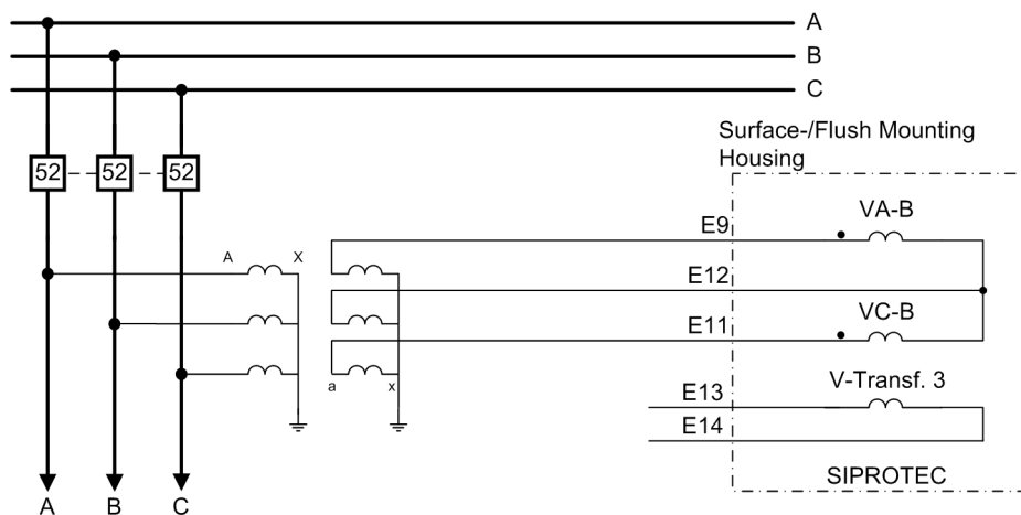
Figure C-19 Example for connection type "VAB, VBC"
