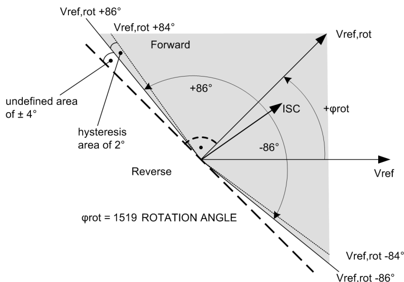
Figure 2-27 Forward characteristic of the directional function, directional phase element
