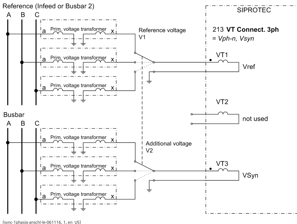
Figure 2-119 Phase-to-ground voltage connection
