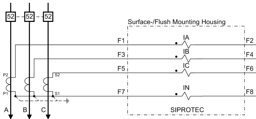
Figure C-1 Current transformer connections to three current transformers and neutral point current (ground current) (Holmgreen connection) – appropriate for all networks
