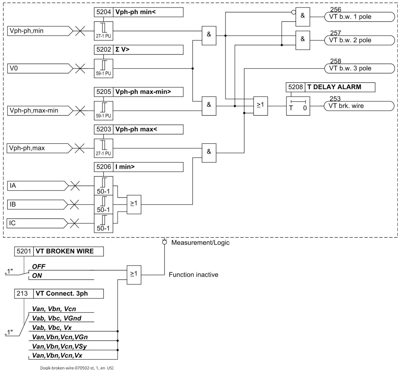
Figure 2-61 Logic diagram for broken wire monitoring
