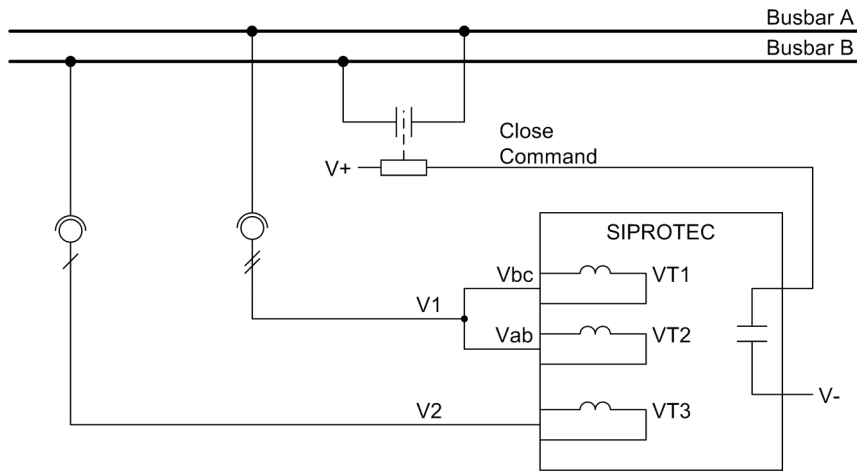
Figure 2-113 Cross coupling
