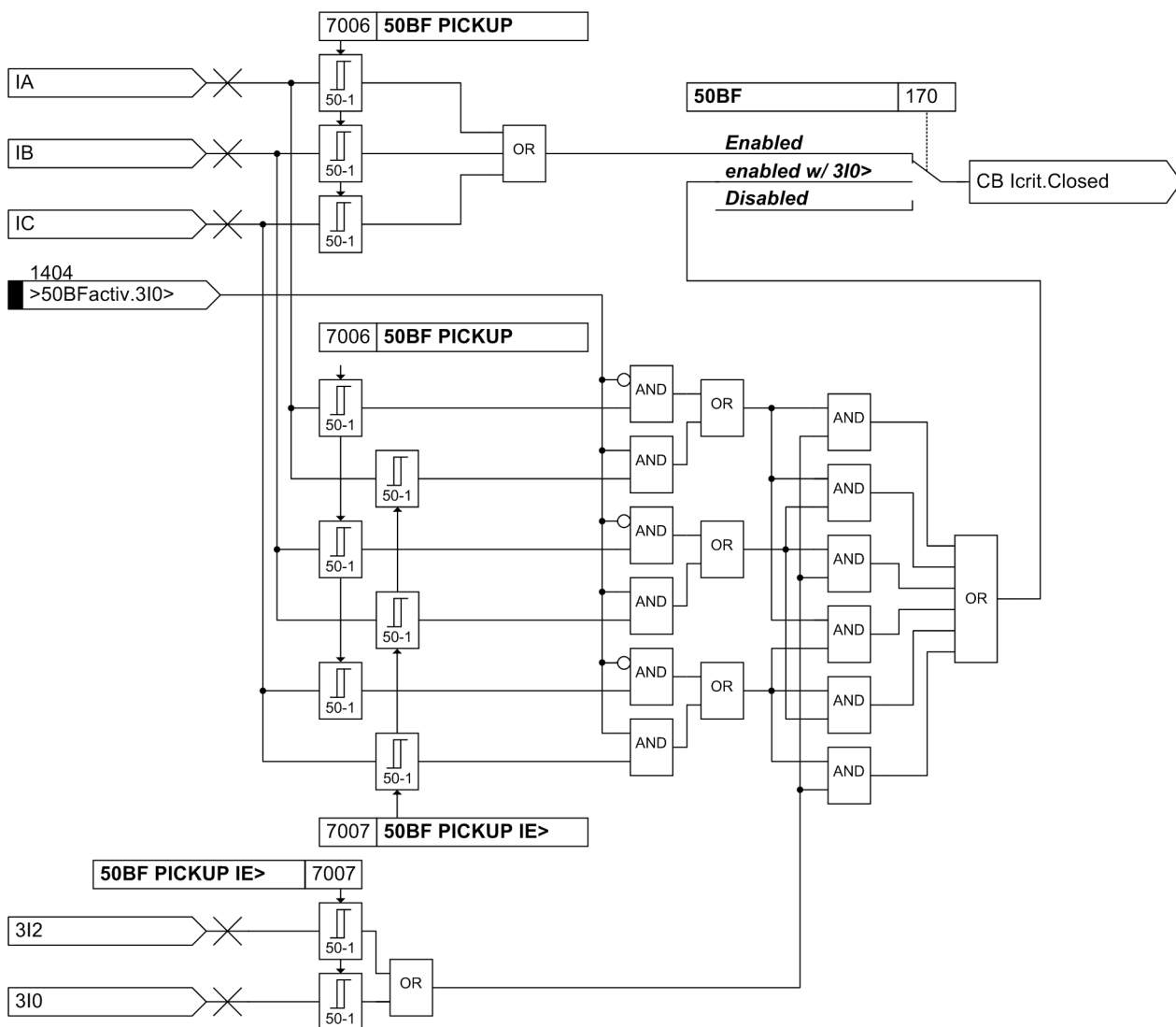
Figure 2-97 Monitoring of the current flow
