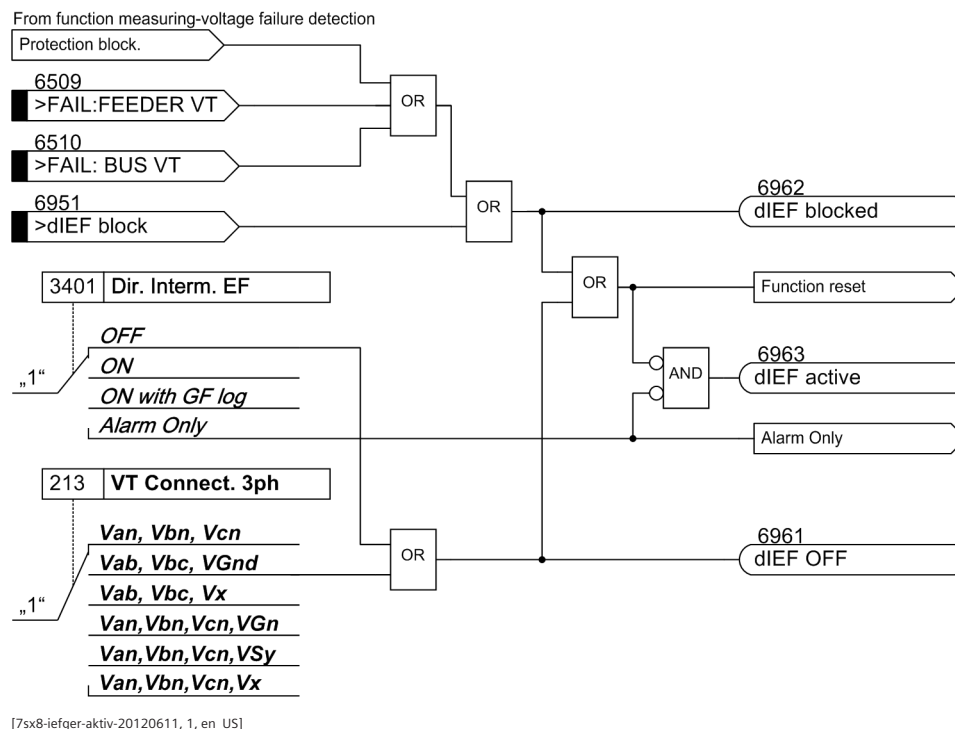
Figure 2-88 Activation of the directional intermittent ground fault protection
