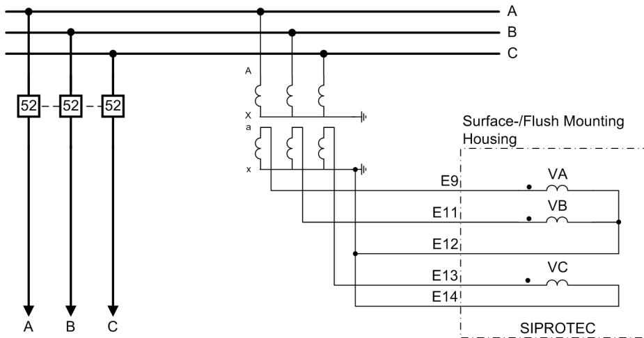
Figure C-16 Example for connection type "VAN, VBN, VCN" busbar-side voltage connection
