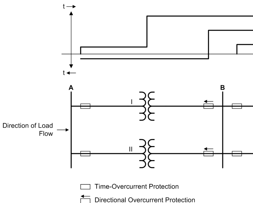
Figure 2-19 Overcurrent protection for parallel transformers
