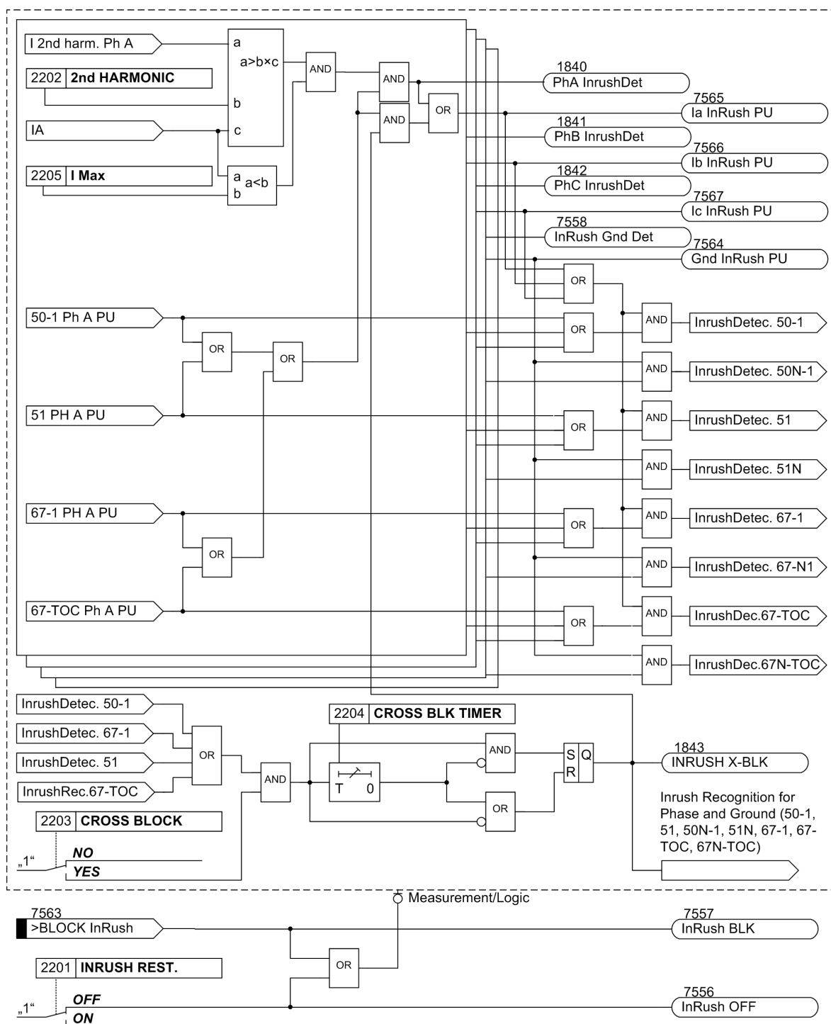
Figure 2-15 Logic diagram for inrush restraint
