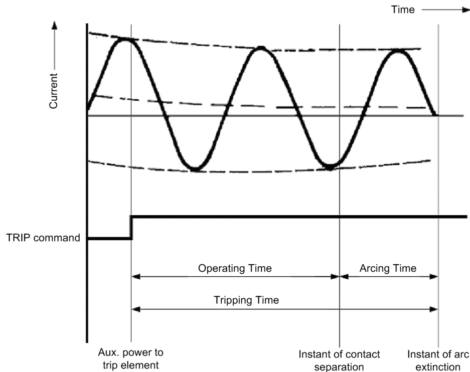
Figure 2-127 Illustration of the CB times
