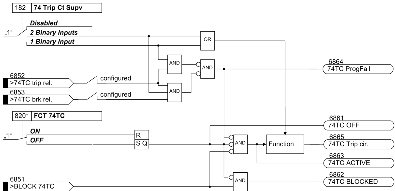
Figure 2-66 Message logic for trip circuit supervision
