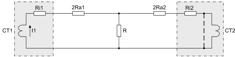
Figure 2-42 Simplified equivalent circuit of a circulating current system for high-impedance protection
