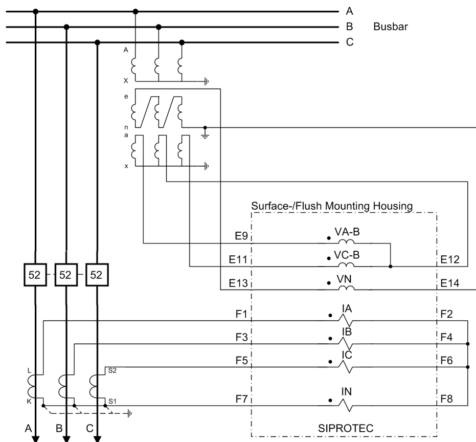
Figure C-7 Transformer connections to three current transformers, two voltage transformers (phase-to-phase voltages) and broken delta winding (da-dn) – appropriate for all networks
