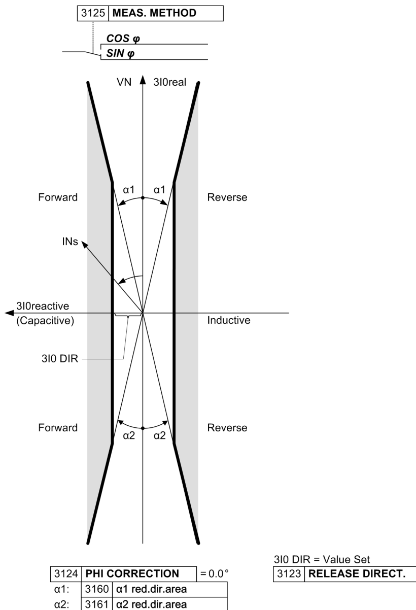
Figure 2-84 Directional characteristic for sin-φ-measurement
