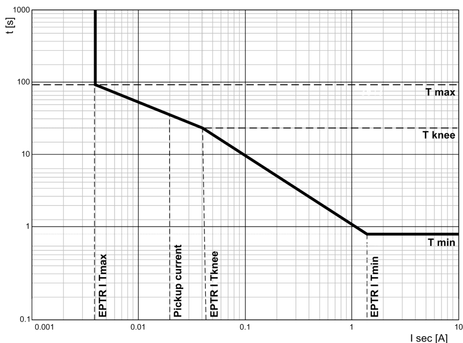
Figure 2-85 Tripping Time Characteristic Curves of the Inverse-Time Ground-Fault Protection with Logarithmic-Inverse Knee-Point Characteristic Curve, Example EPTR
