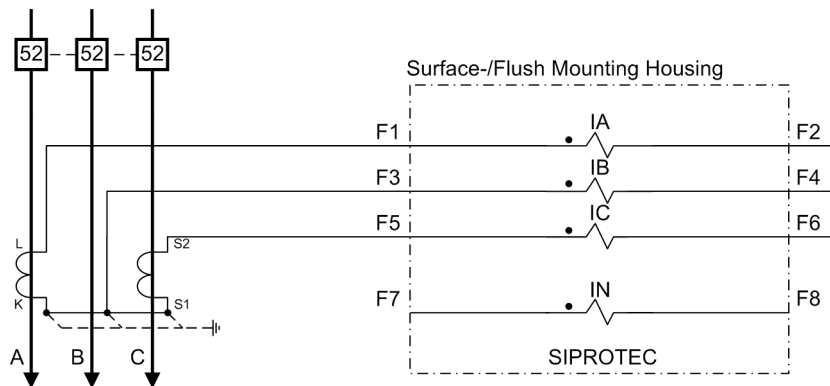
Figure C-2 Current transformer connections to two current transformers – only for isolated or resonant-grounded networks
