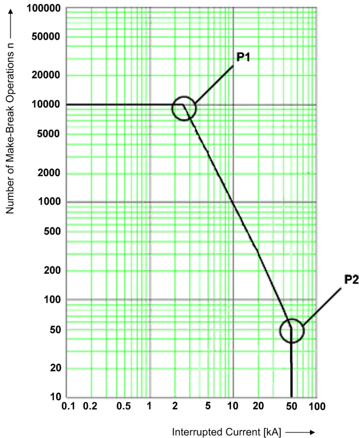
Figure 2-125 Diagram of operating cycles for the 2P procedure
