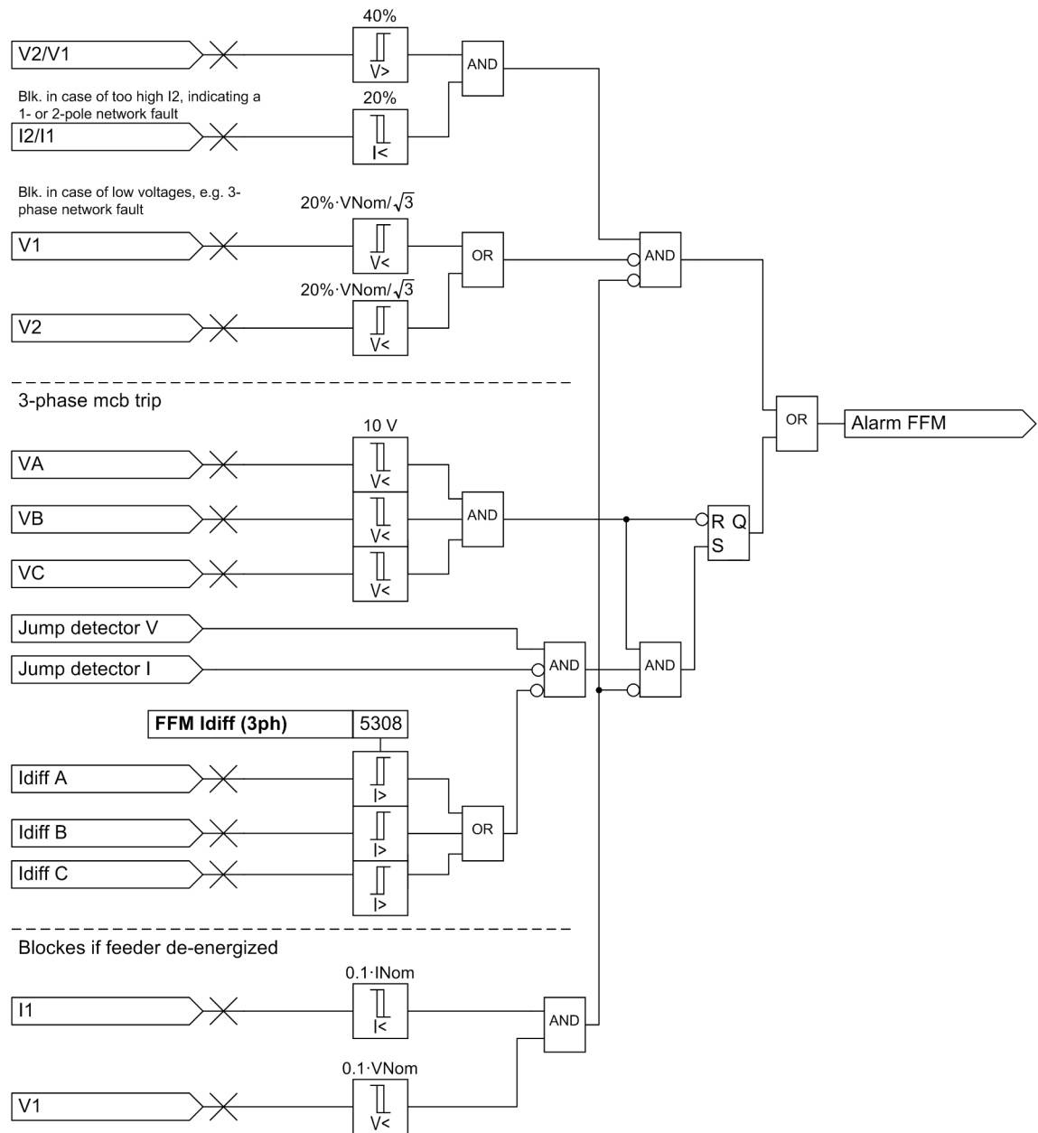
Figure 2-60 Logic diagram of the Fuse Failure Monitor for isolated and grounded systems
