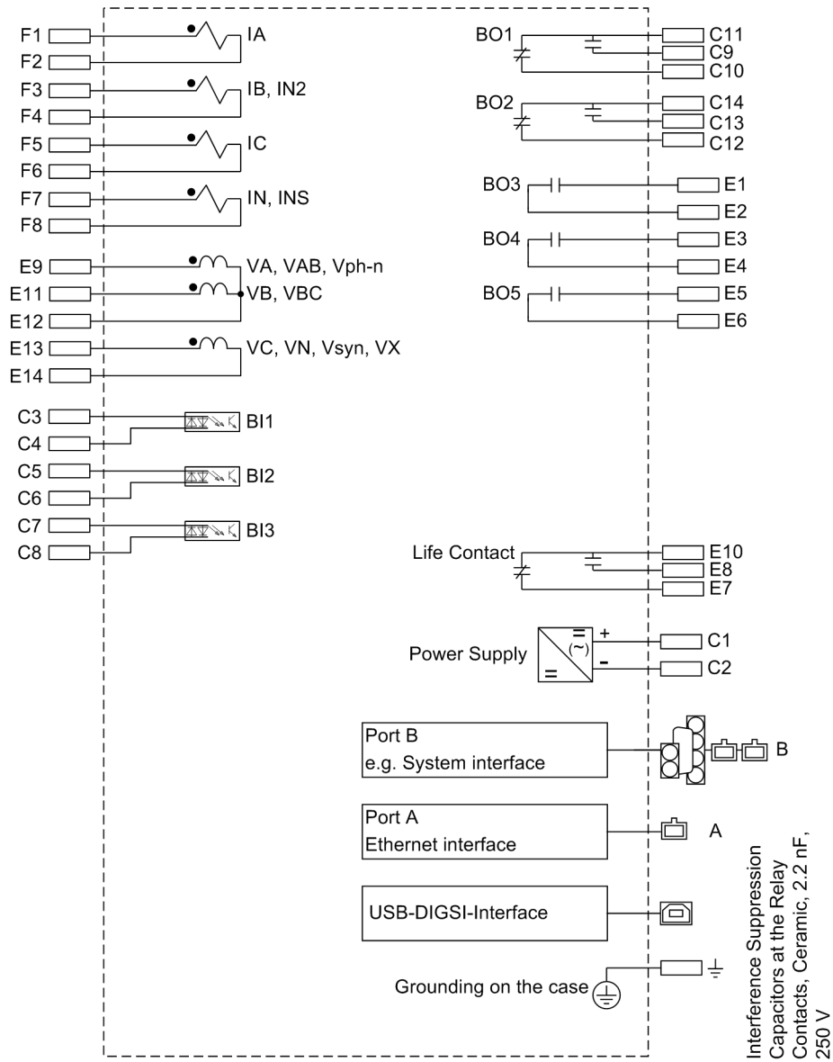
Figure B-3 Block diagram 7SJ803*
