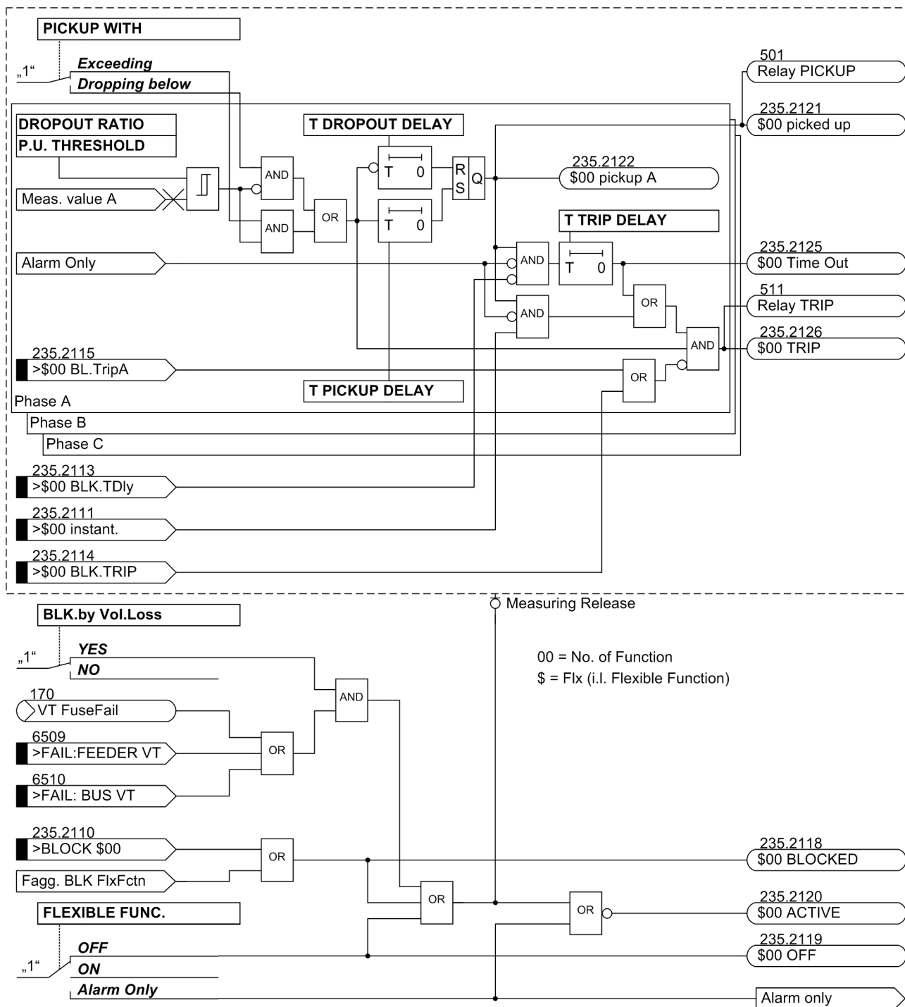
Figure 2-102 Logic diagram of the flexible protection functions
