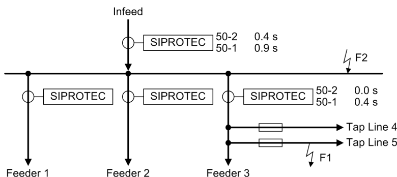
Figure 2-93 Zone sequencing with a fault occurring at Tap Line 5 and at the busbar
