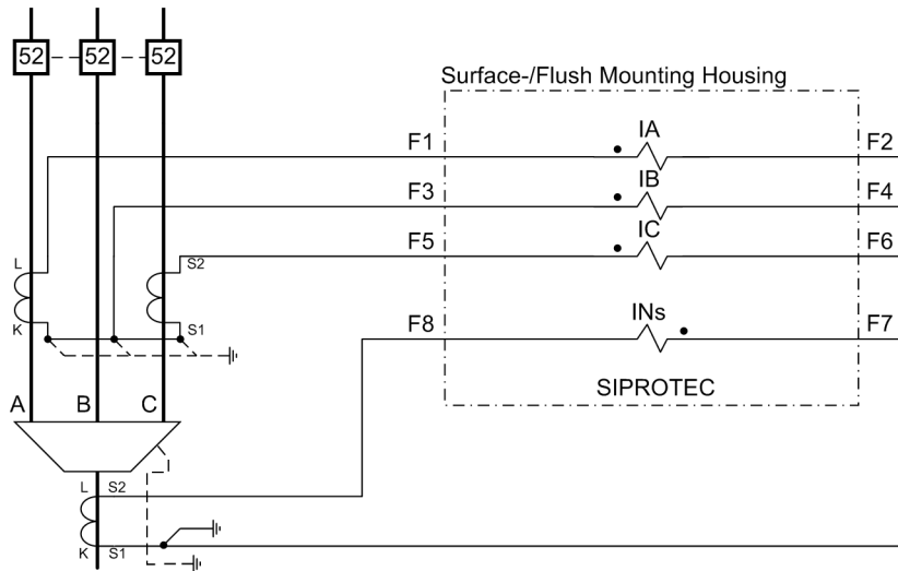
Figure C-4 Current transformer connections to two current transformers - additional cable-type current transformer for sensitive ground fault detection - only for isolated or resonant-grounded networks
