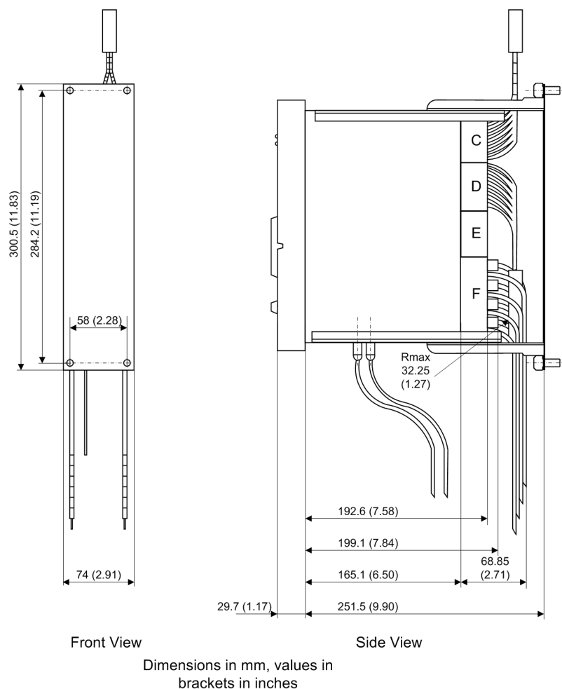
Figure 4-13 Dimensional drawing of a 7SJ80 for panel surface mounting (housing size 1/6)
