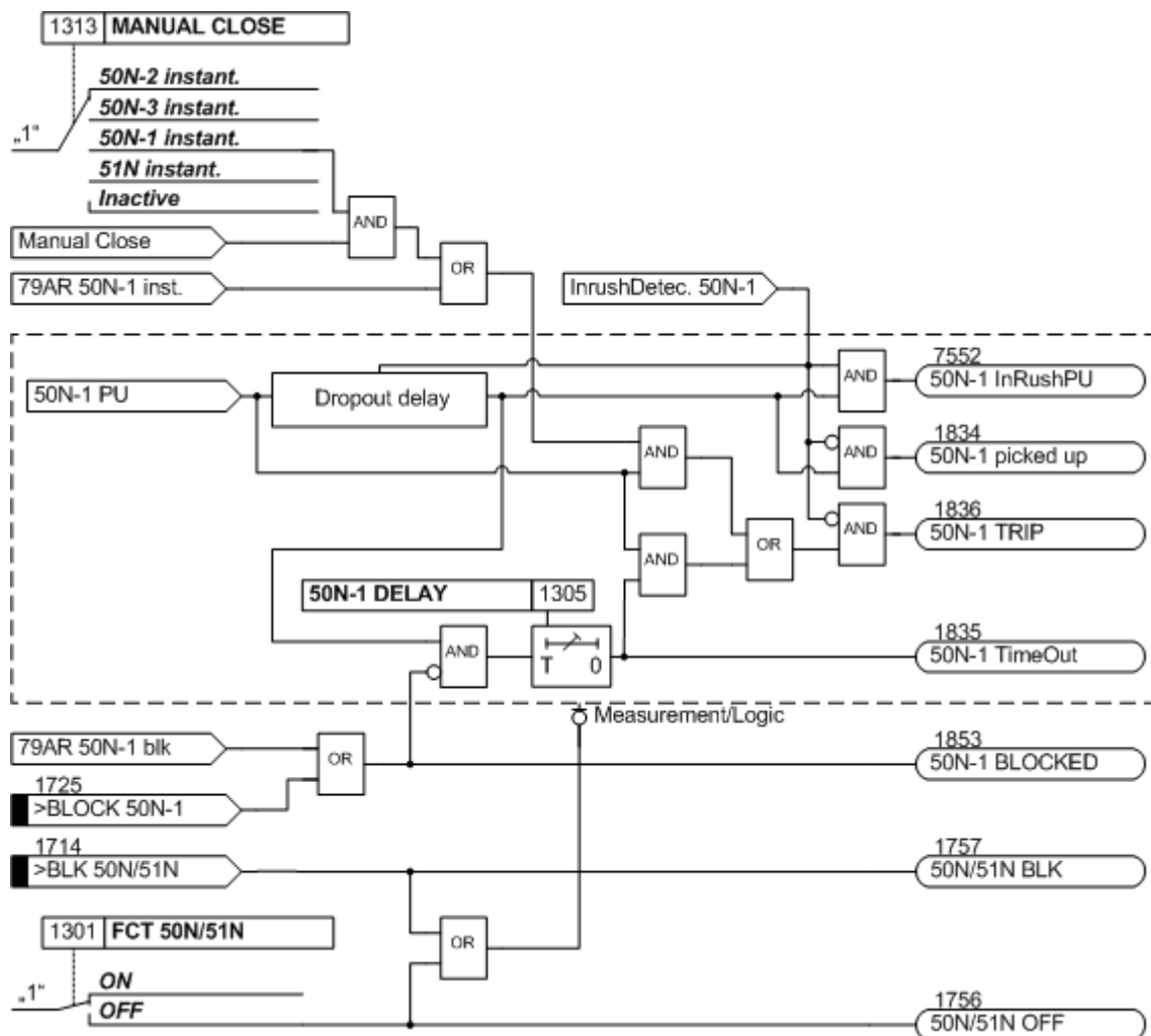
Figure 2-8 Logic diagram for the 50N-1 overcurrent current element
