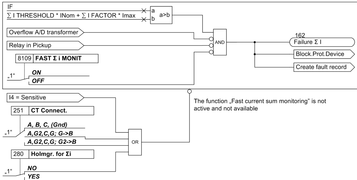
Figure 2-56 Logic Diagram of the fast current sum monitoring
