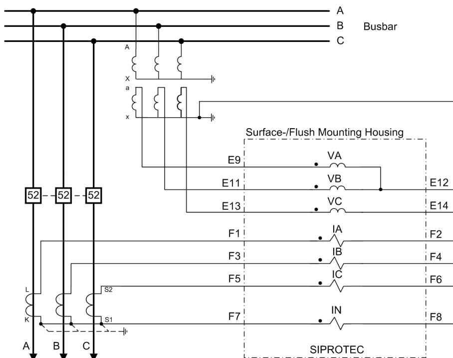
Figure C-6 Transformer connections to three current transformers and three voltage transformers (phase-to-ground voltages), normal circuit layout – appropriate for all networks
