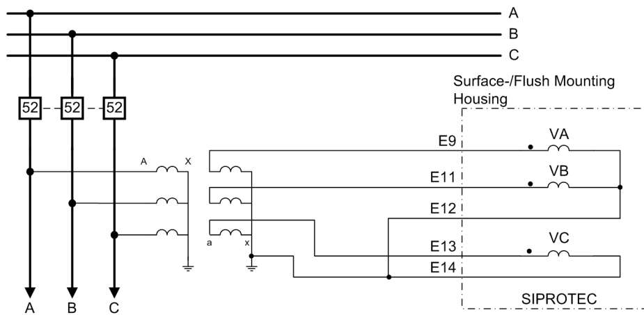
Figure C-14 Example for the connection type "VAN, VBN, VCN" with voltage connection on the feeder side
