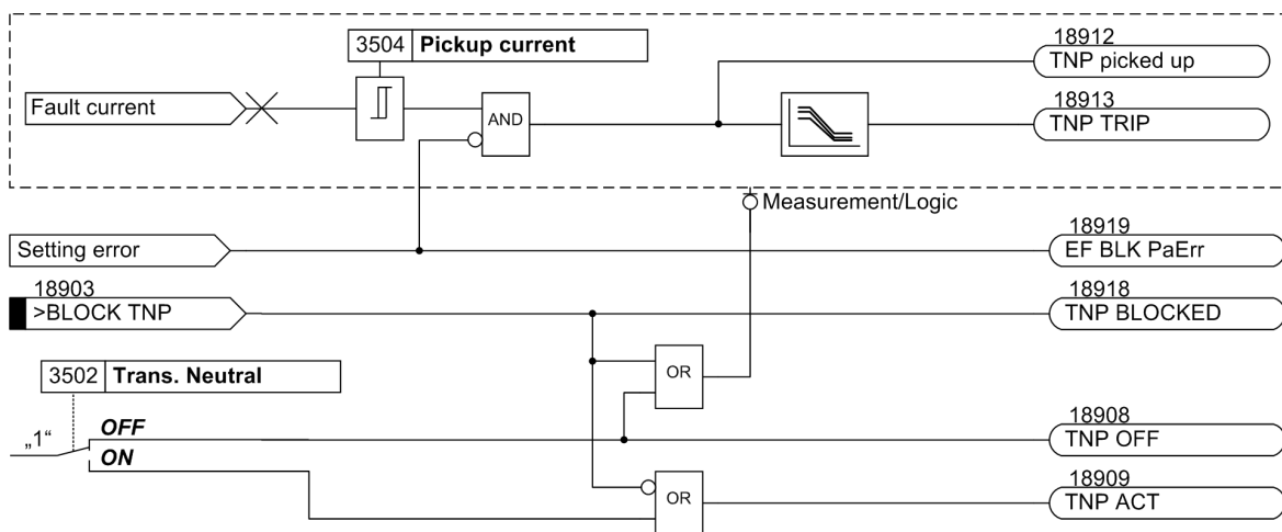
Figure 2-80 Logic of the Ground-Fault Detection for a Transformer with Grounded Neutral Point
