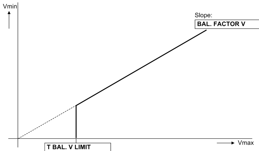
Figure 2-58 Voltage symmetry monitoring
