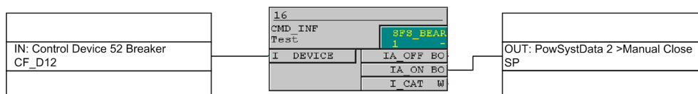
Figure 2-33 Example for the generation of a manual close signal using the internal control function
