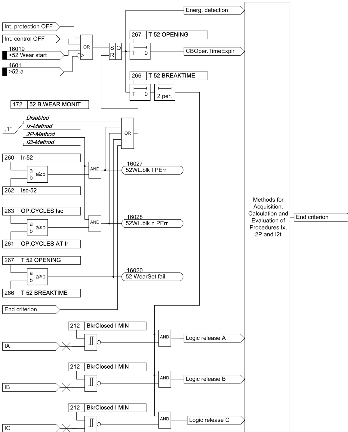
Figure 2-124 Logic of the start and end criterion
