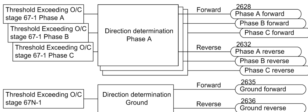
Figure 2-31 Logic diagram for the generation of fault direction signals
