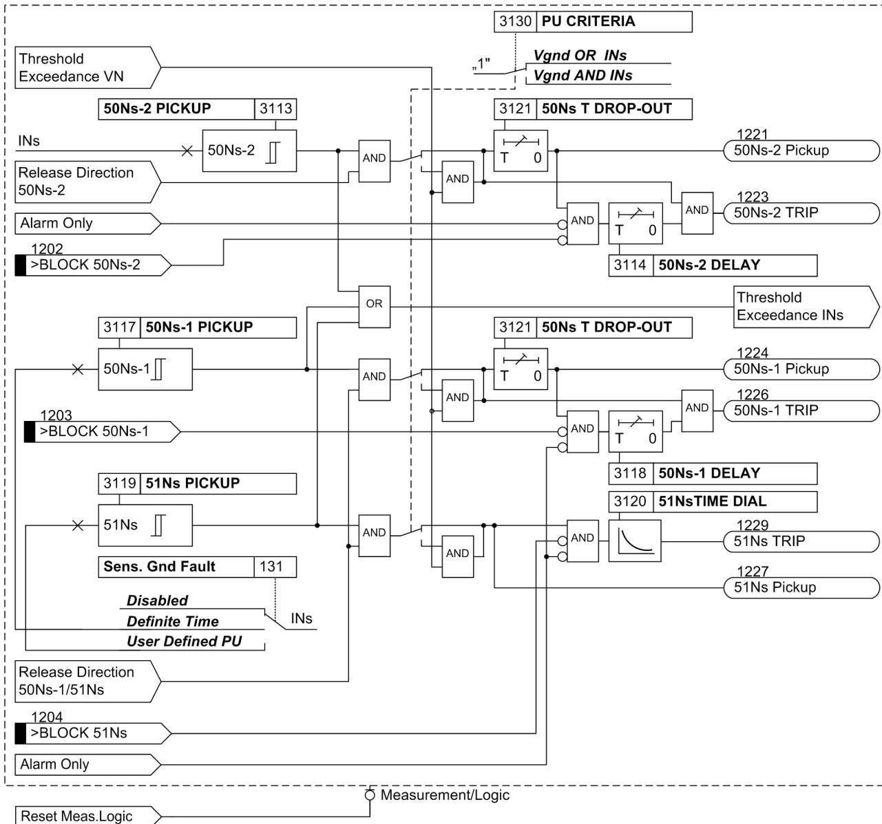
Figure 2-72 Logic diagram of the I_{Ns} elements for \cos\phi / \sin\phi measurement
