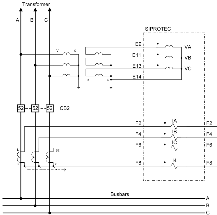
Figure 2-104 Wiring diagram for a 7SJ80 as reverse power protection
