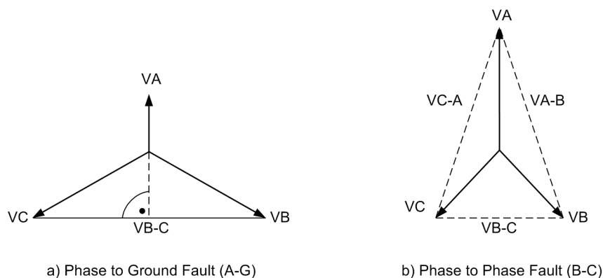
Figure 2-25 Cross-polarized voltages for direction determination
