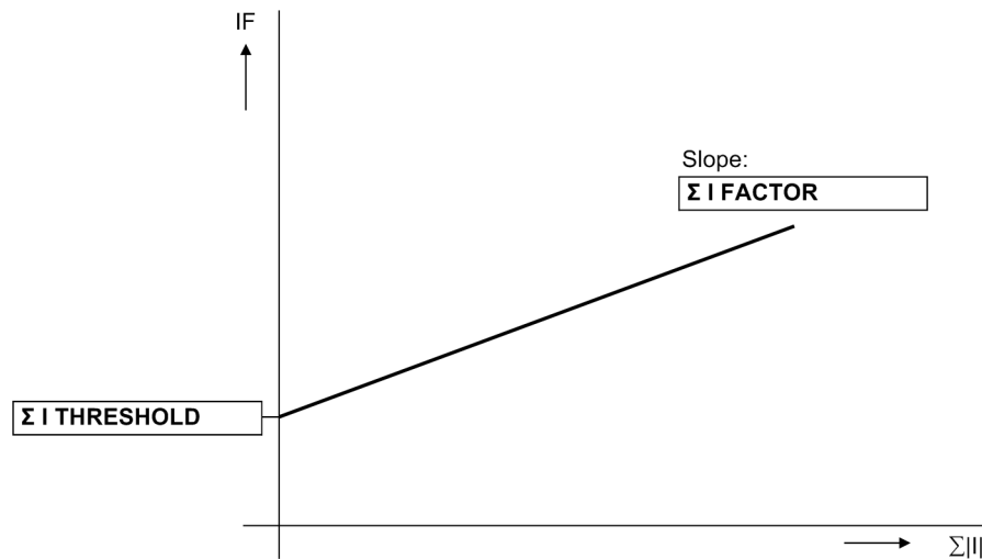
Figure 2-55 Current sum monitoring
