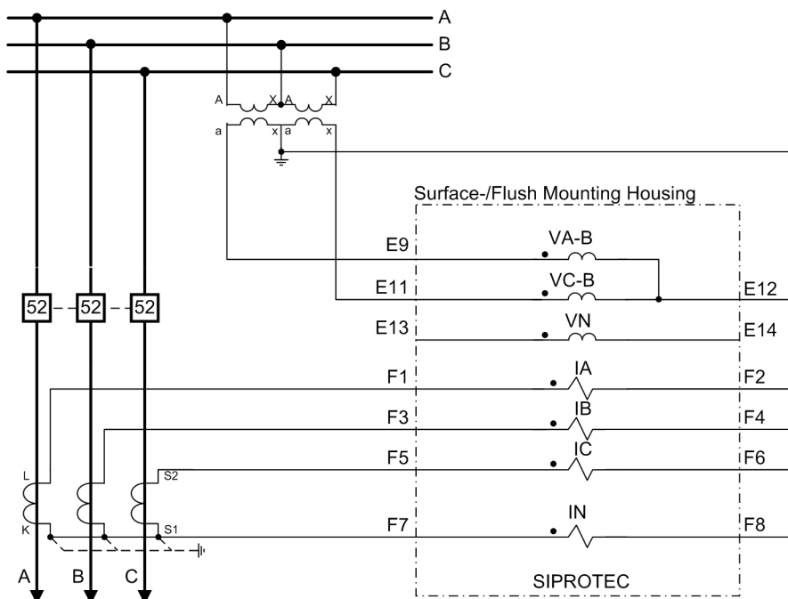
Figure C-9 Current transformer connections to three current transformers, two voltage transformers in open-deltaconnection, only for isolated or resonant-grounded networks; no directional ground protection since displacement voltage cannot be calculated
