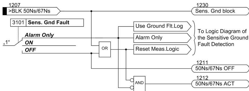
Figure 2-70 Activation of the sensitive ground-fault detection for \cos\phi / \sin\phi measurement
