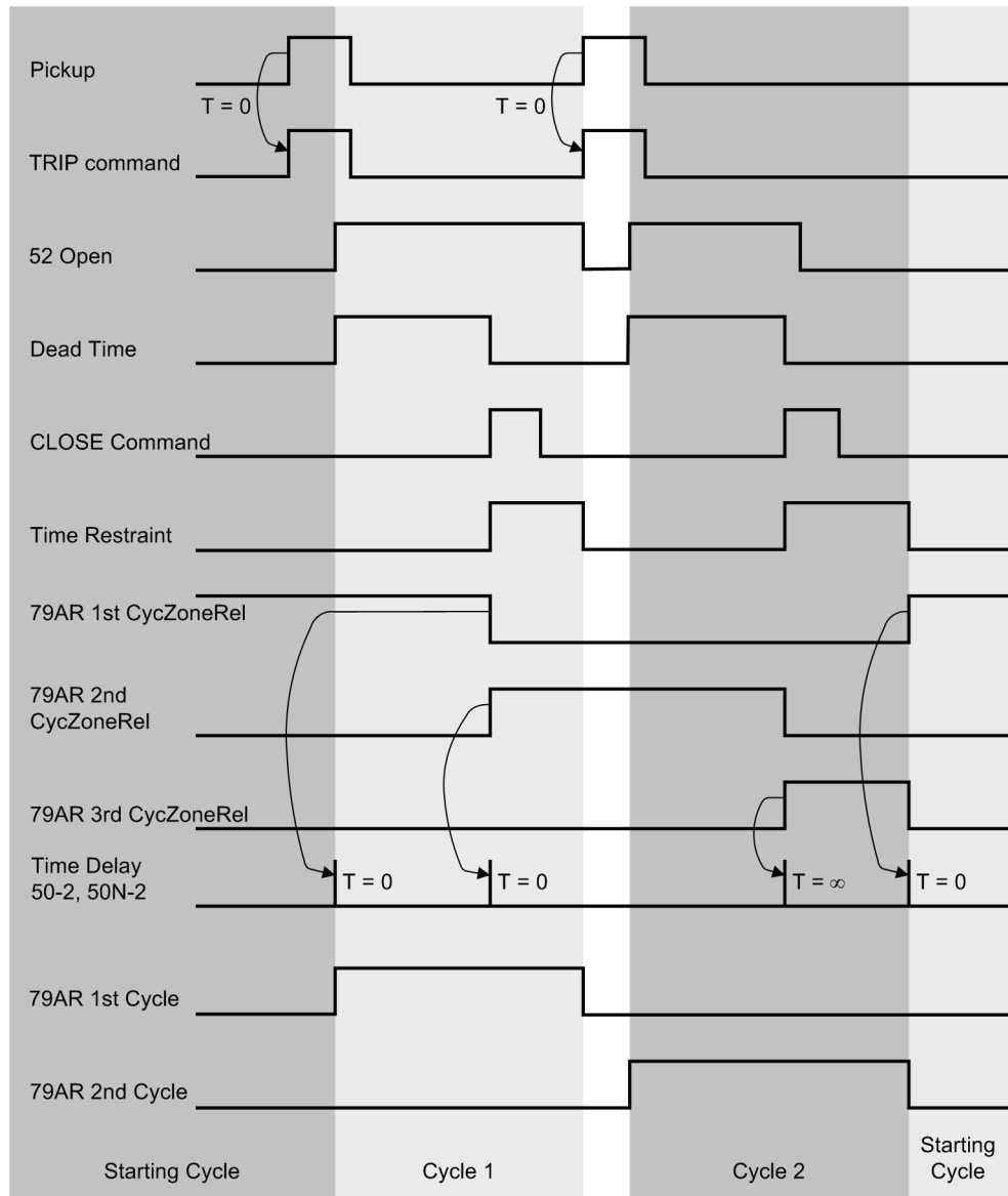
Figure 2-92 Control of protection elements for two-fold, successful automatic reclosure
