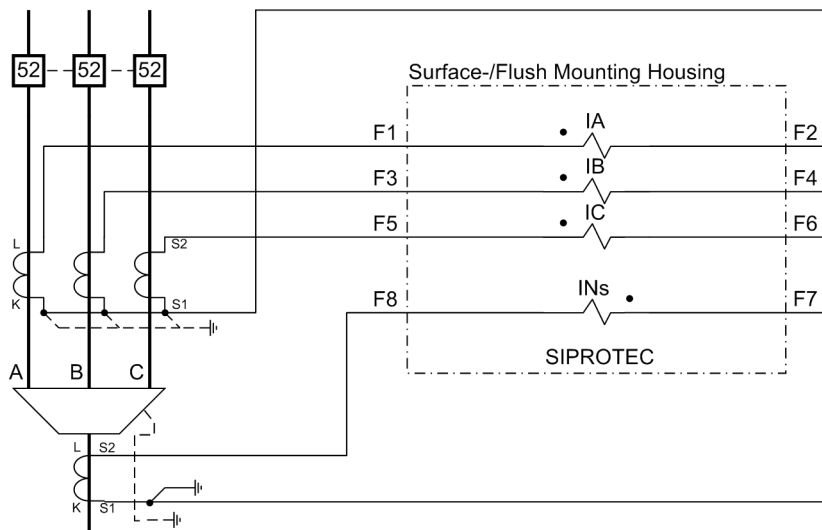
Figure C-5 Current transformer connections to three current transformers - ground current from additional cable-type current transformer for sensitive ground fault detection
