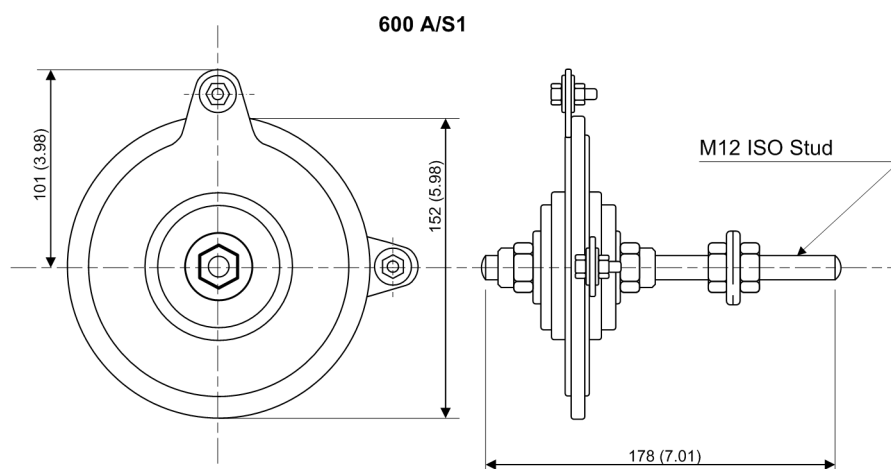
Figure 4-15 Dimensional drawing of the varistor for voltage limiting in high-impedance differential protection
