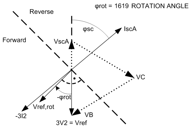
Figure 2-29 Rotation of the reference voltage, directional ground element with negative sequence values
