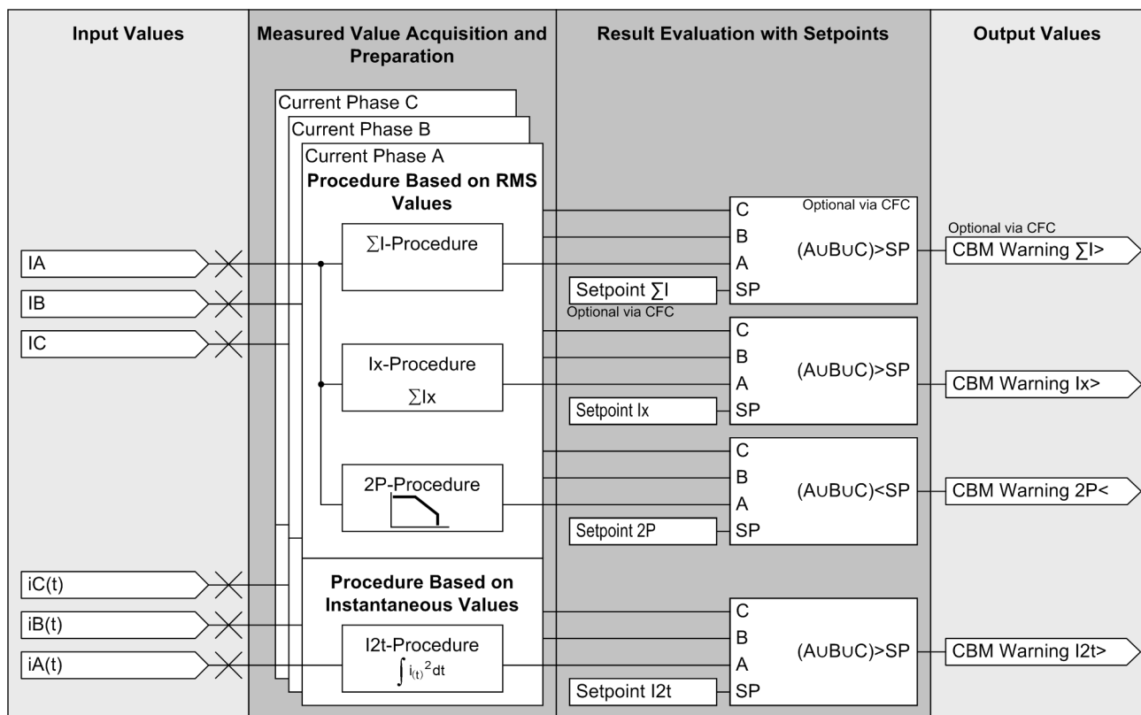
Figure 2-123 Diagram of CB maintenance procedures
