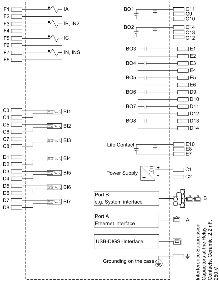
Figure B-2 Block diagram 7SJ802*
