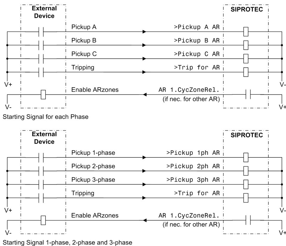
Figure 2-57 Connection example with external protection device for fault detection dependent dead time — dead time control by pickup signals of the protection device; AR control mode = with PICKUP
