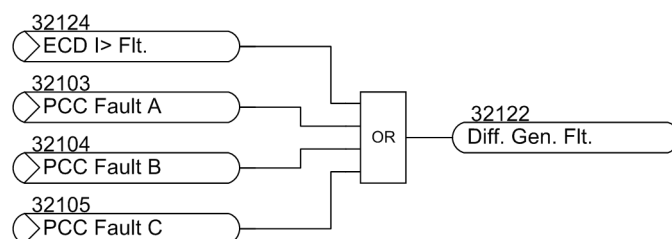
Figure 2-15 General pickup
