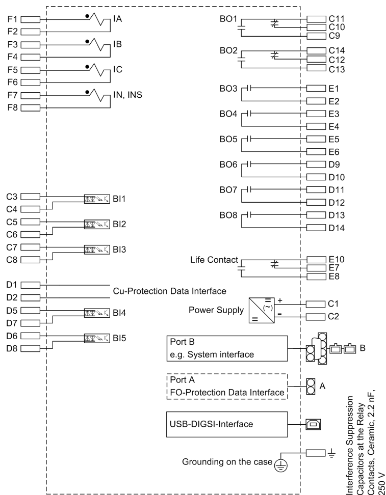
Figure A-3 Connection diagram 7SD803*
