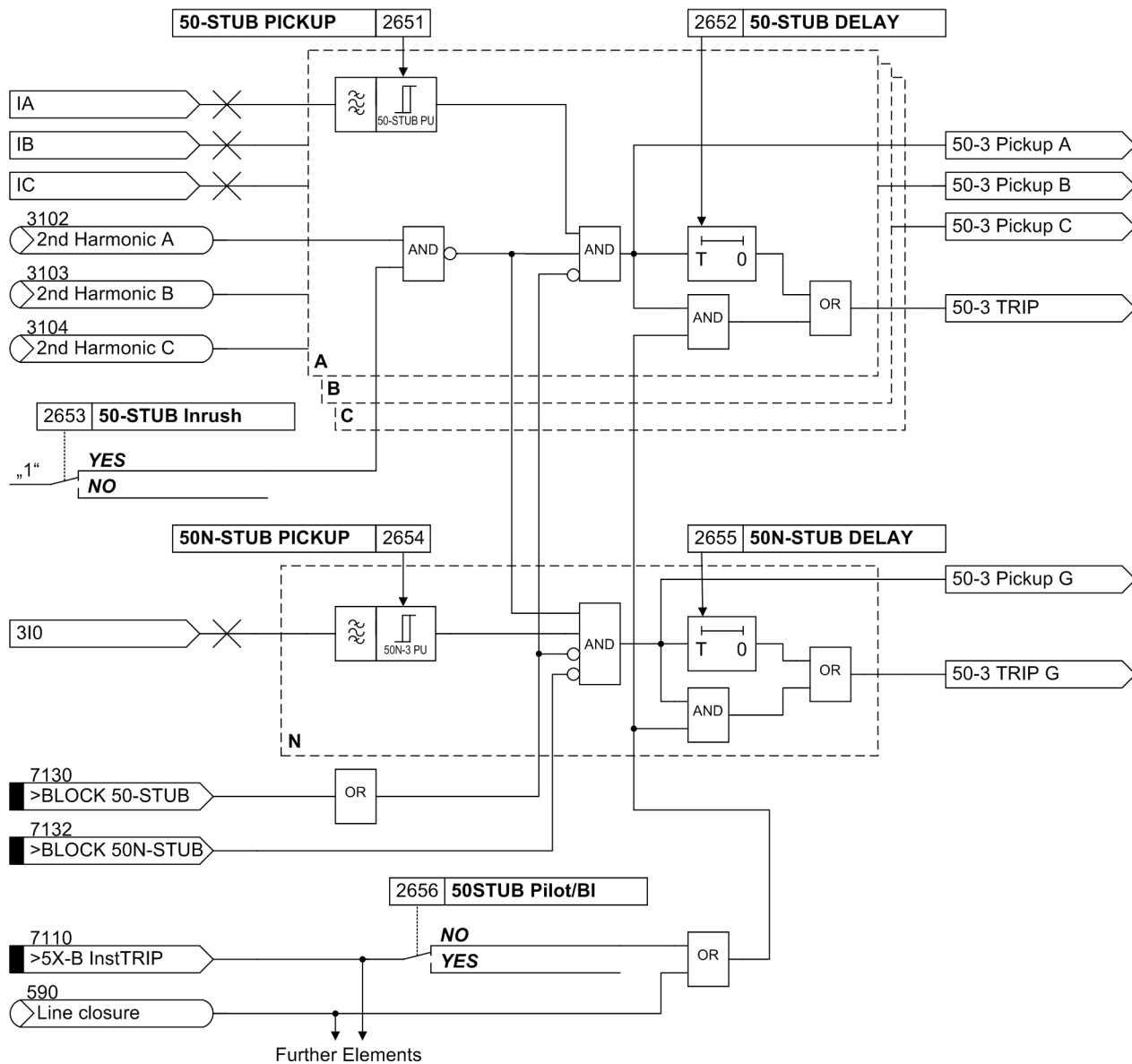
Figure 2-27 Logic diagram of the 50-3 element
