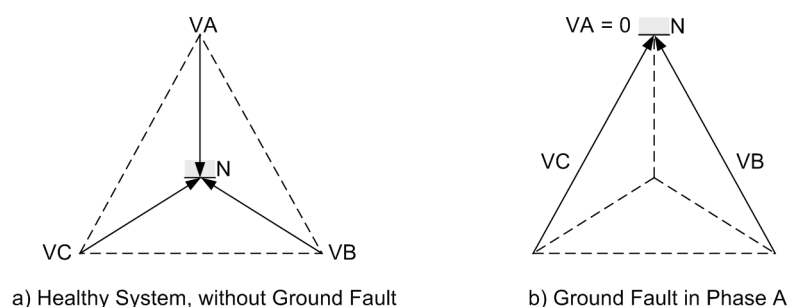
Figure 2-13 Ground fault in non-grounded neutral system
