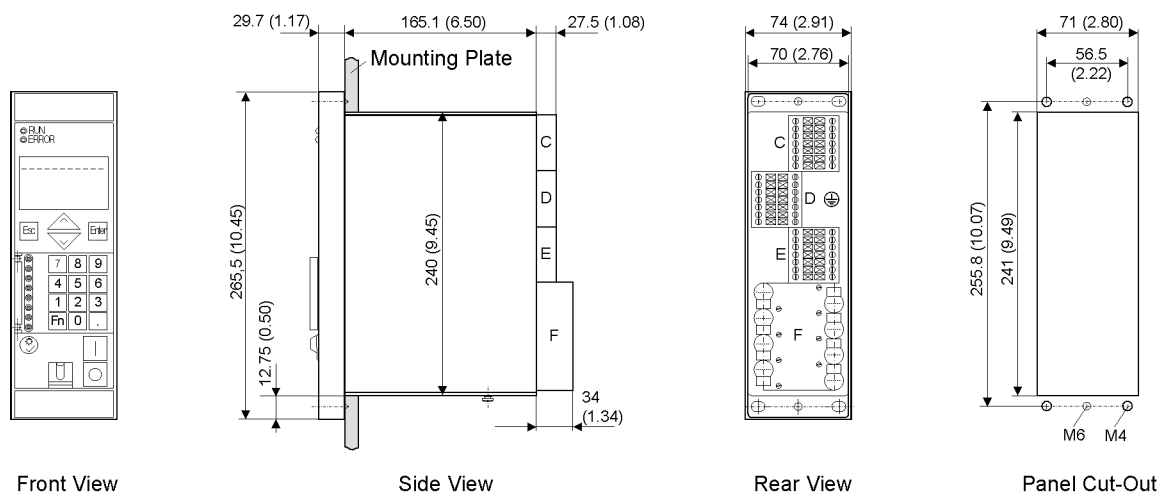
Figure 4-7 Dimensional drawing of a 7SD80 for panel flush mounting and cabinet flush mounting (housing size 1/6)
