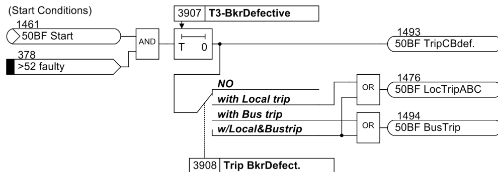
Figure 2-40 Circuit-breaker faulty
