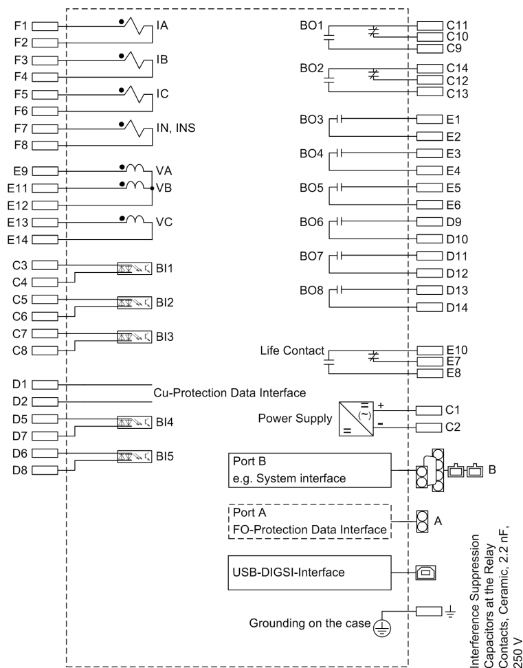
Figure A-6 Connection diagram 7SD807*
