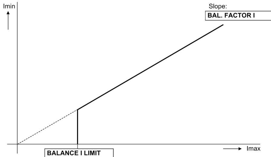
Figure 2-65 Current symmetry monitoring
