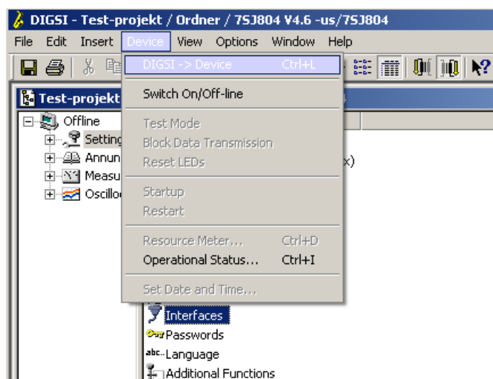
Figure 3-25 Transmitting data
