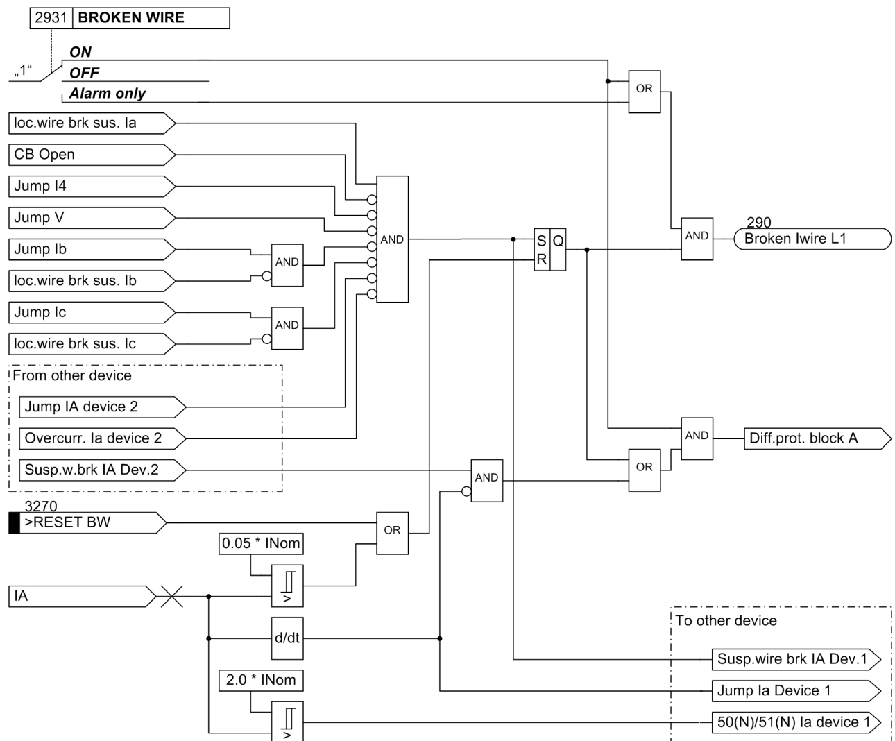
Figure 2-68 Broken-wire monitoring
