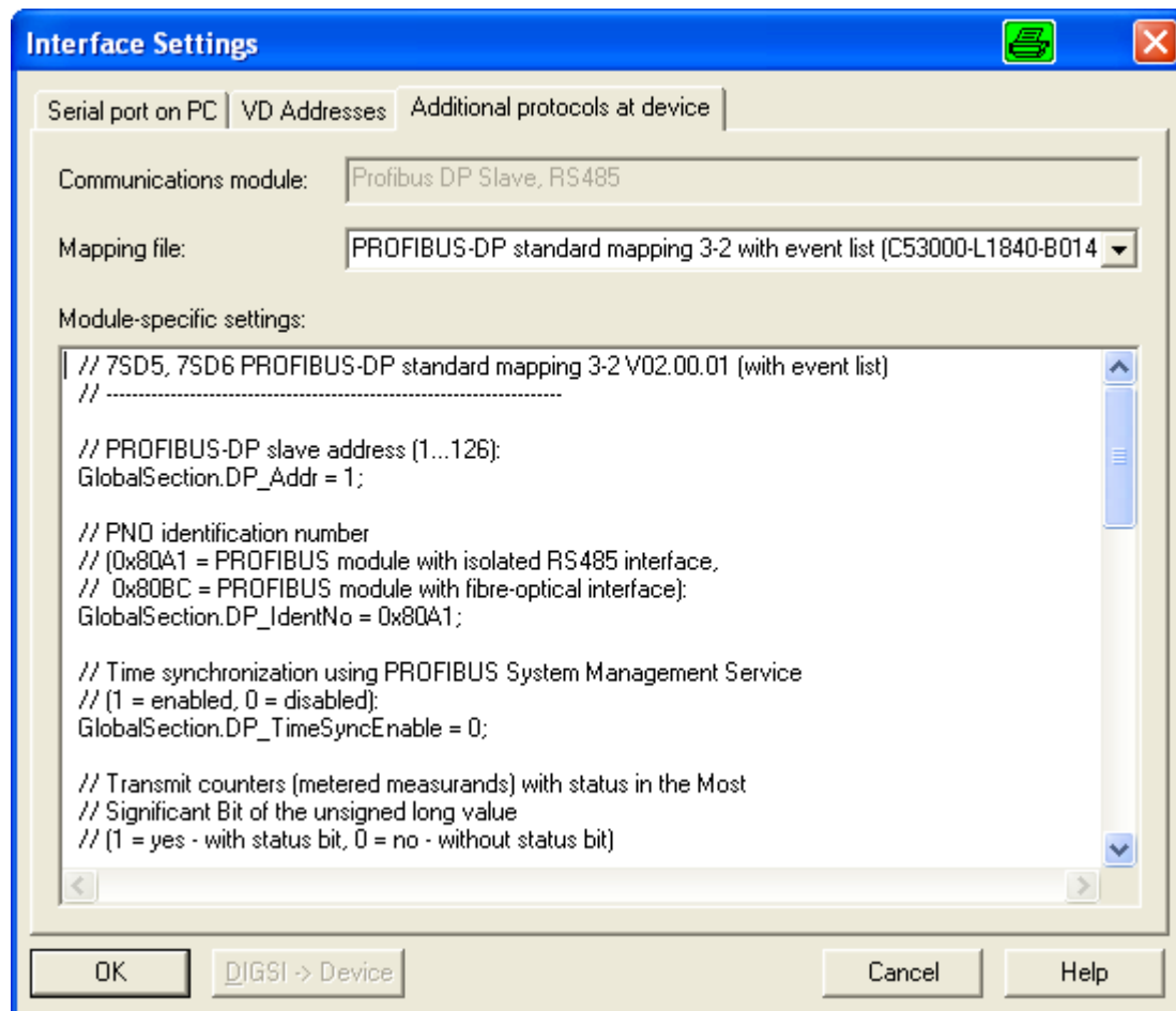
Figure 3-24 Module-specific settings
