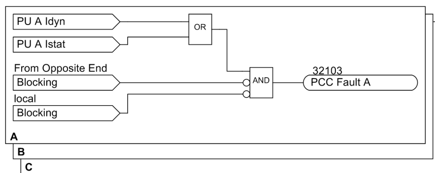
Figure 2-8 Logic diagram of phase comparison protection for pickup in a grounded system
