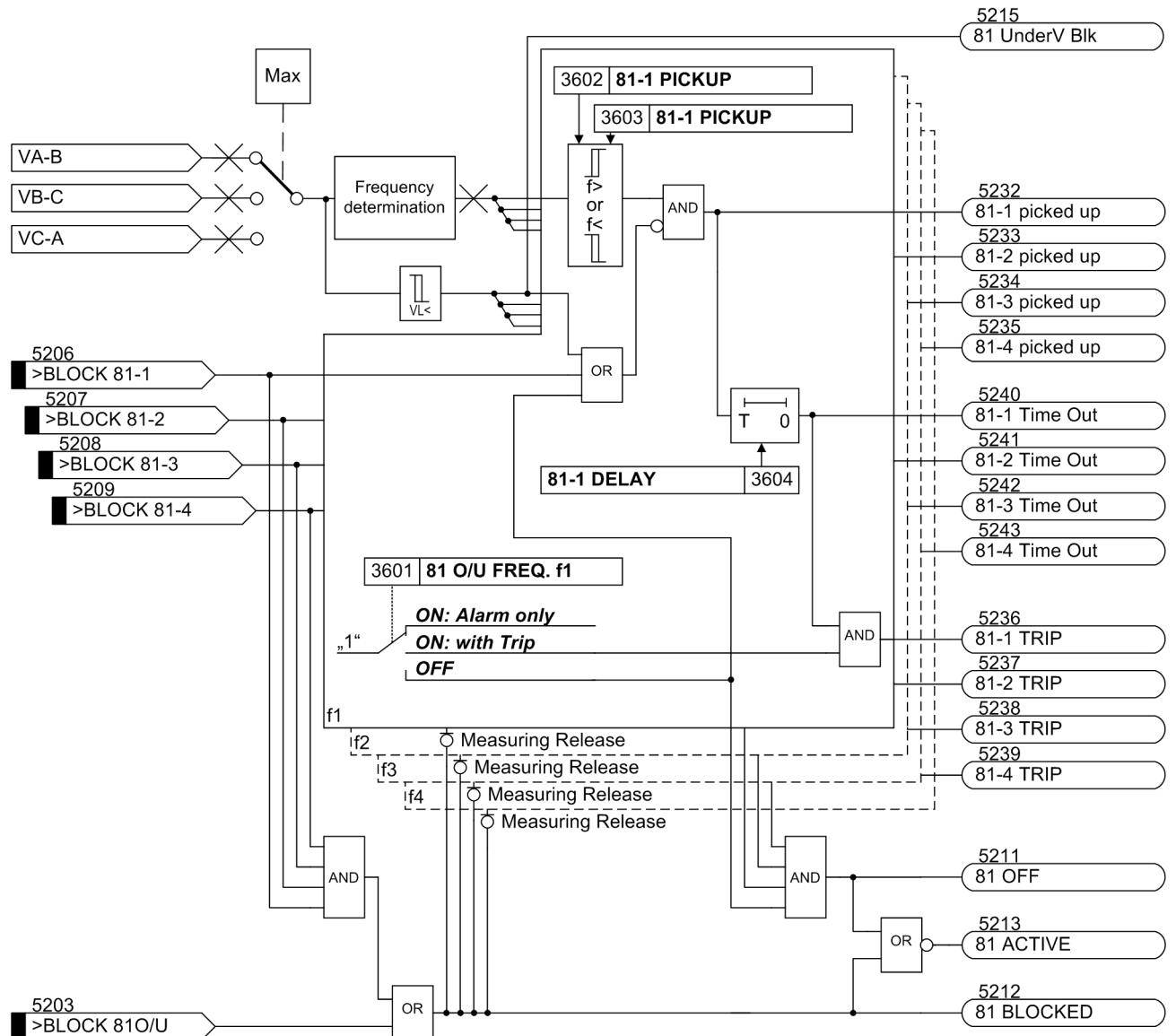
Figure 2-52 Logic diagram of frequency protection for 50 Hz rated frequency
