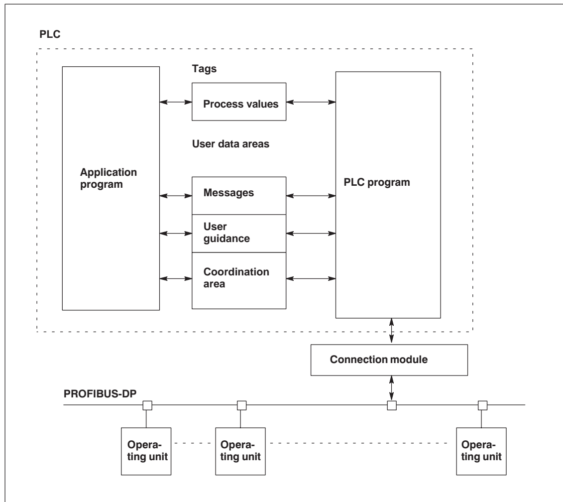
Figure 13-1 Communication structure
