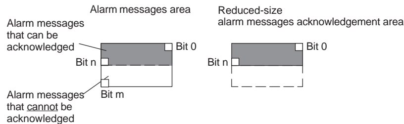
Figure 7-7 Reduced-size acknowledgement area
