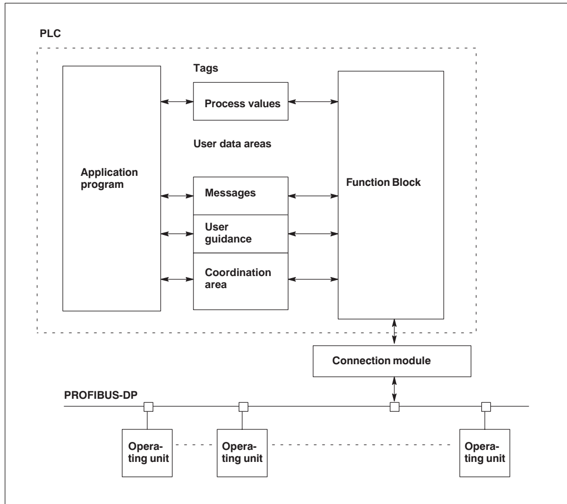
Figure 4-1 Communication structure
