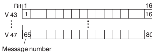
Figure 14-2 Assignment of message bit and message number
