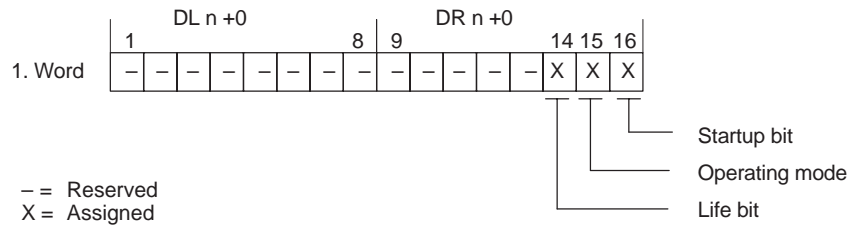
Figure 14-10 Significance of the bits in the coordination area
