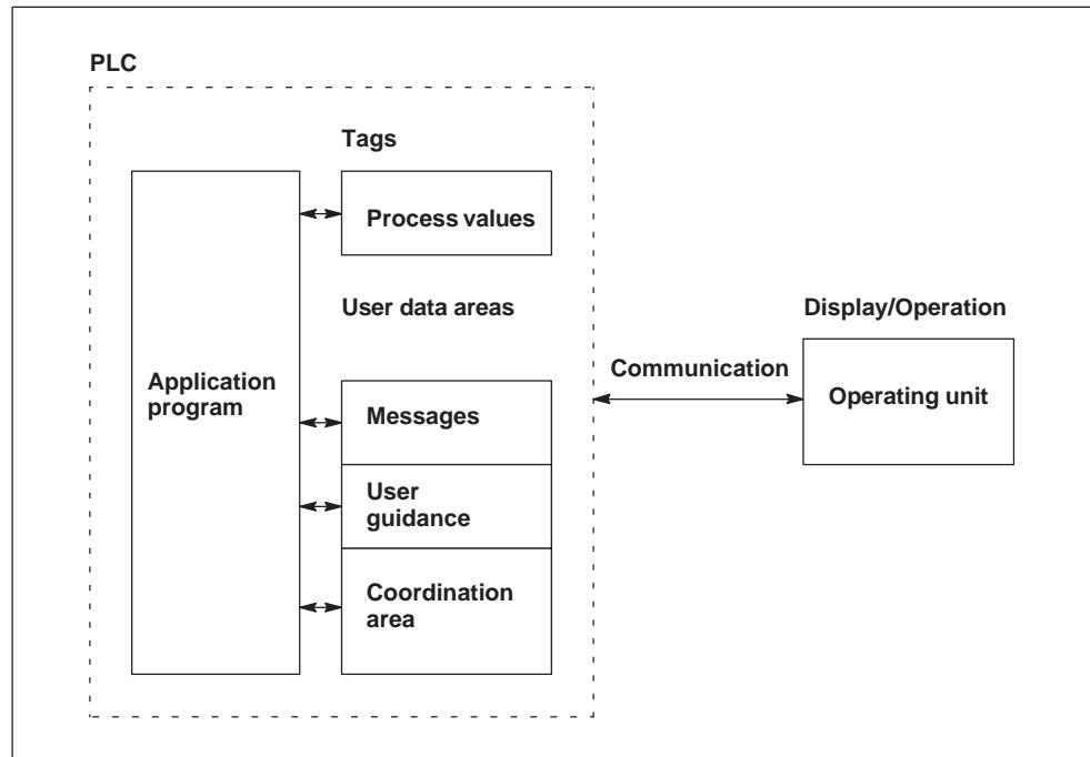
Figure 16-1 Communication structure
