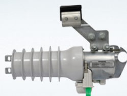
3AD8 Fusesaver
