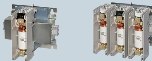
3TM1 and 3TM3 vacuum contactors
