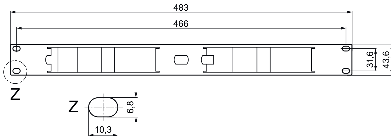
Figure 9-5 Front view
