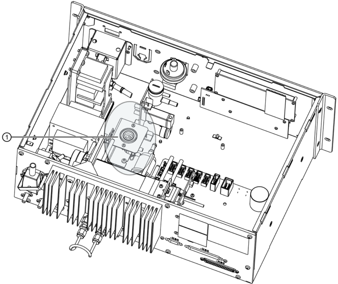
Figure 10-2 Sensor holder ① (shaded)
