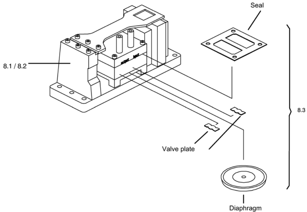
Figure 13-8 Pump
