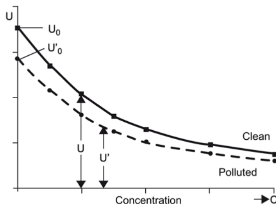
Figure 3-8 Calibration
