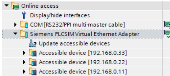
Figure 4-10 Accessible devices on the Siemens PLCSIM Virtual Ethernet Adapter
