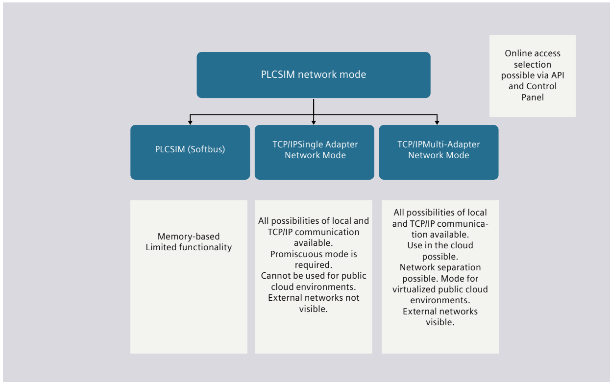
Figure 4-6 S7-PLCSIM networking
